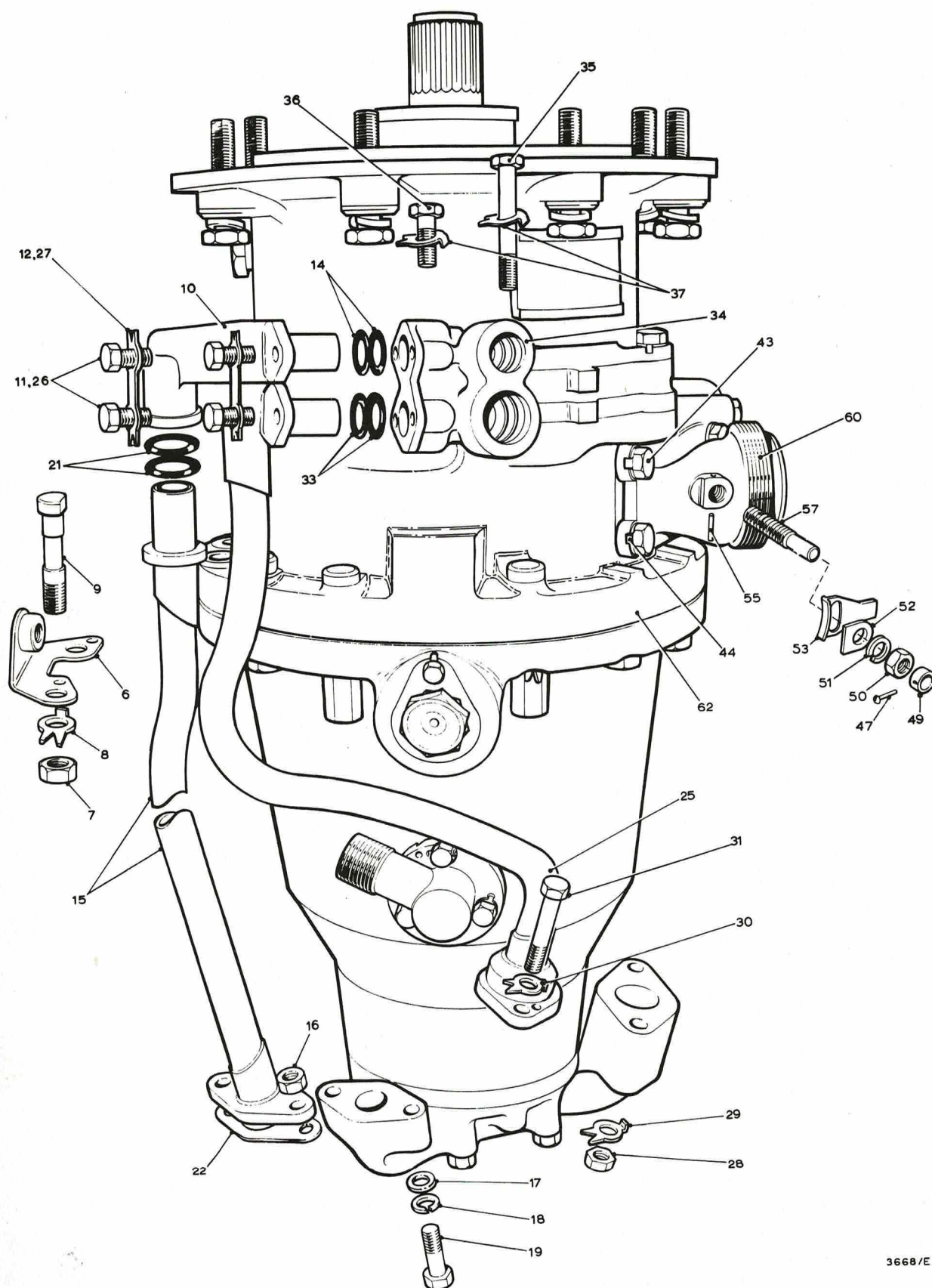
Fig.1 Engine group 5/E1
