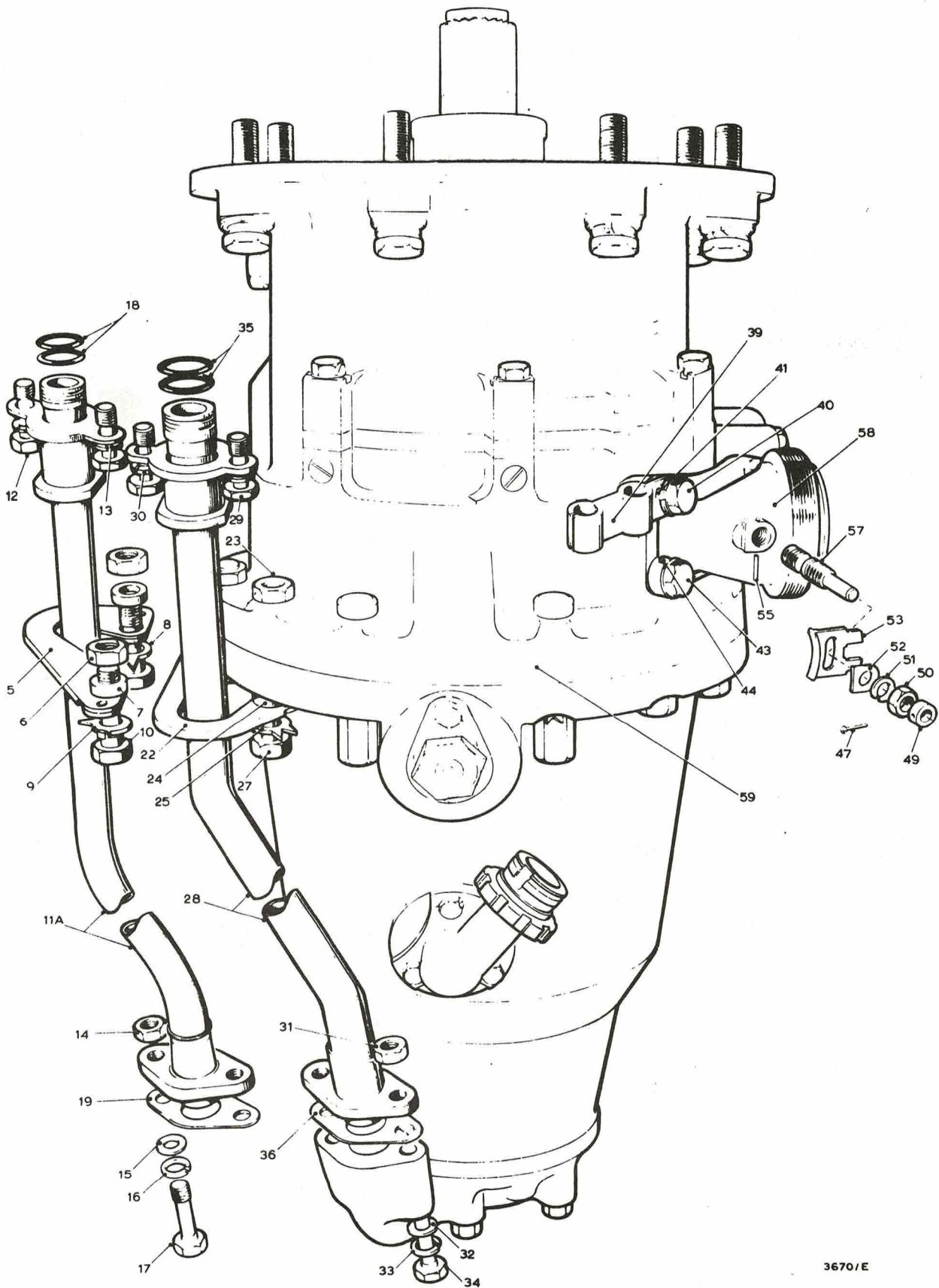
Fig.2 Engine group 5/E2
