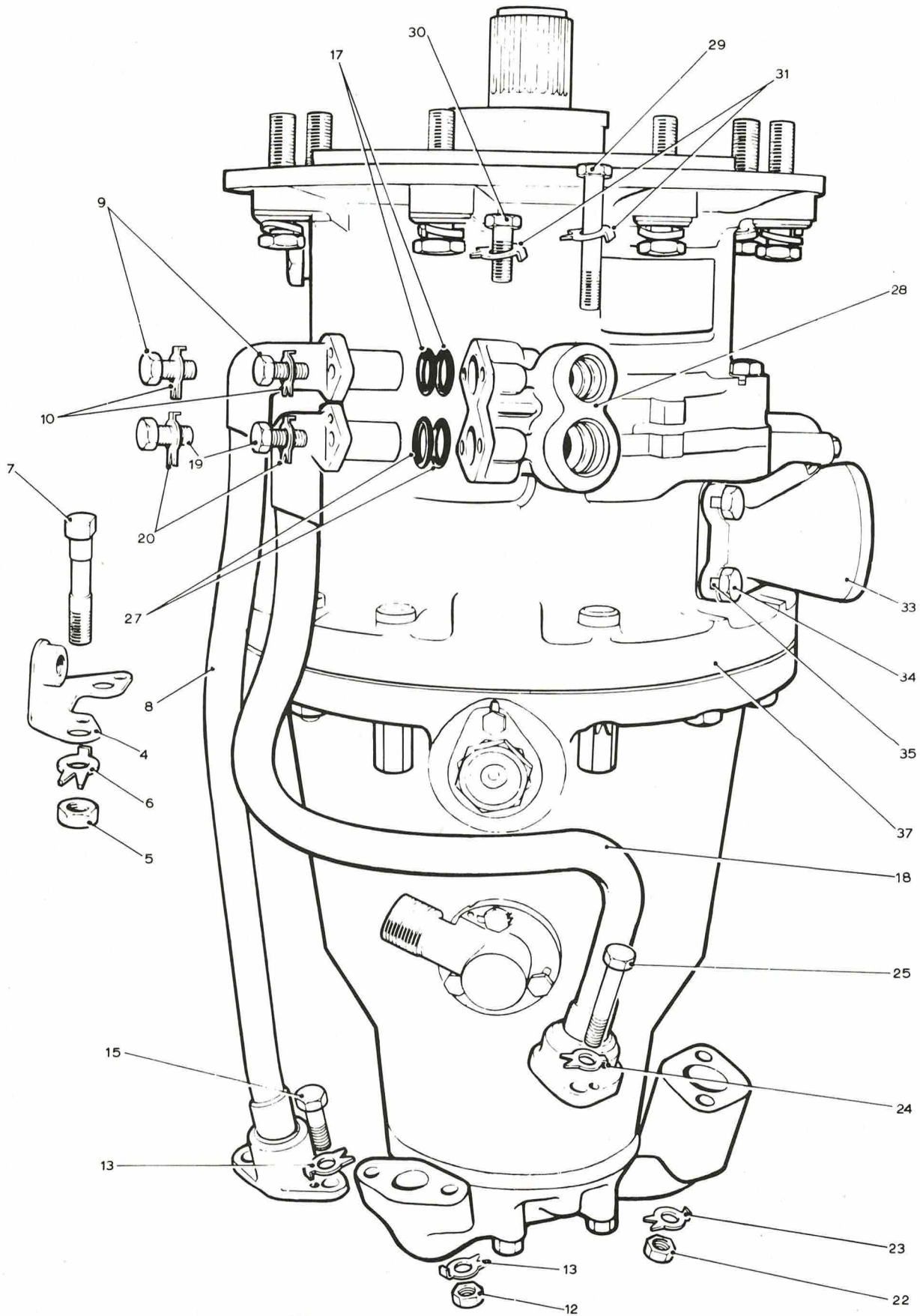
Fig.3 Engine group 23/E
