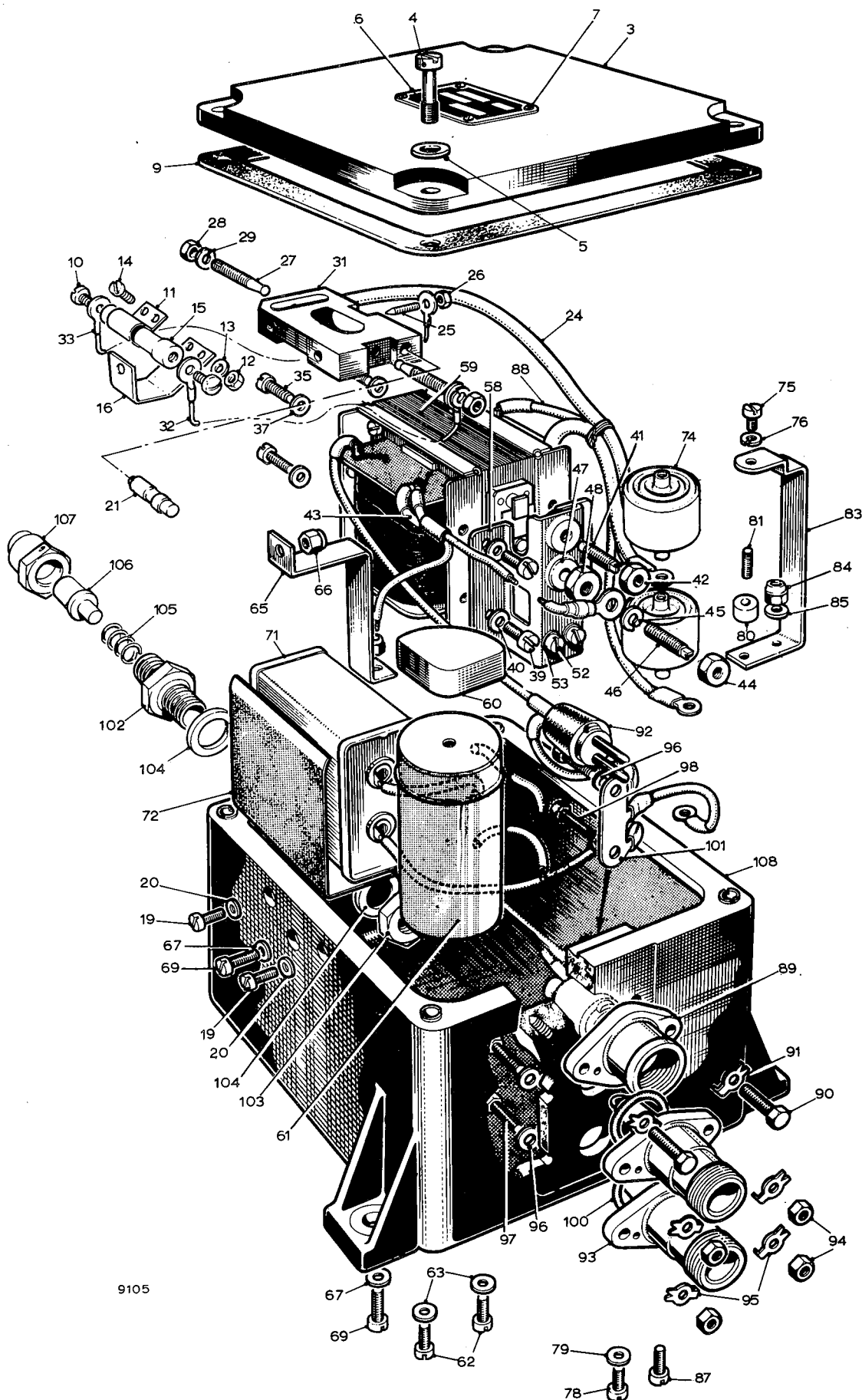
Fig.1 Ignition unit
