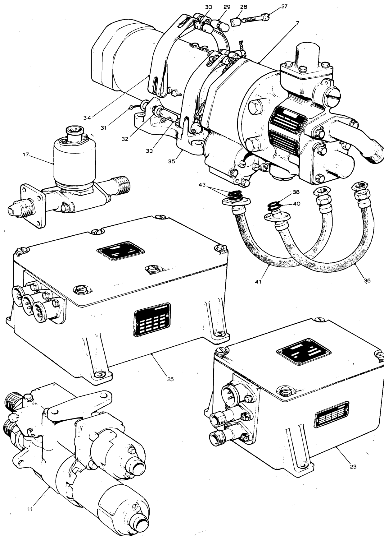
Fig.1 Airframe group (basic)
