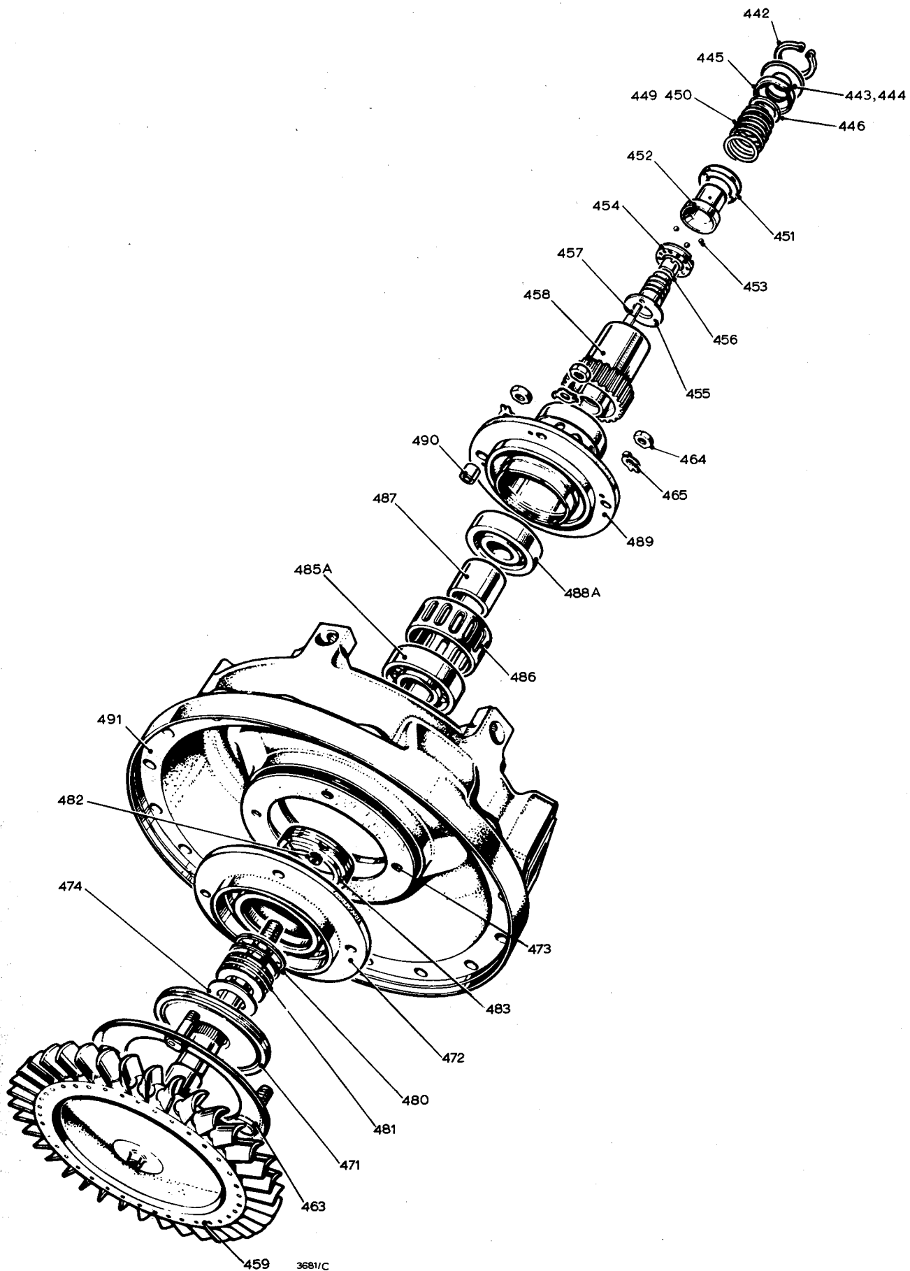
Fig.11 Turbine unit
