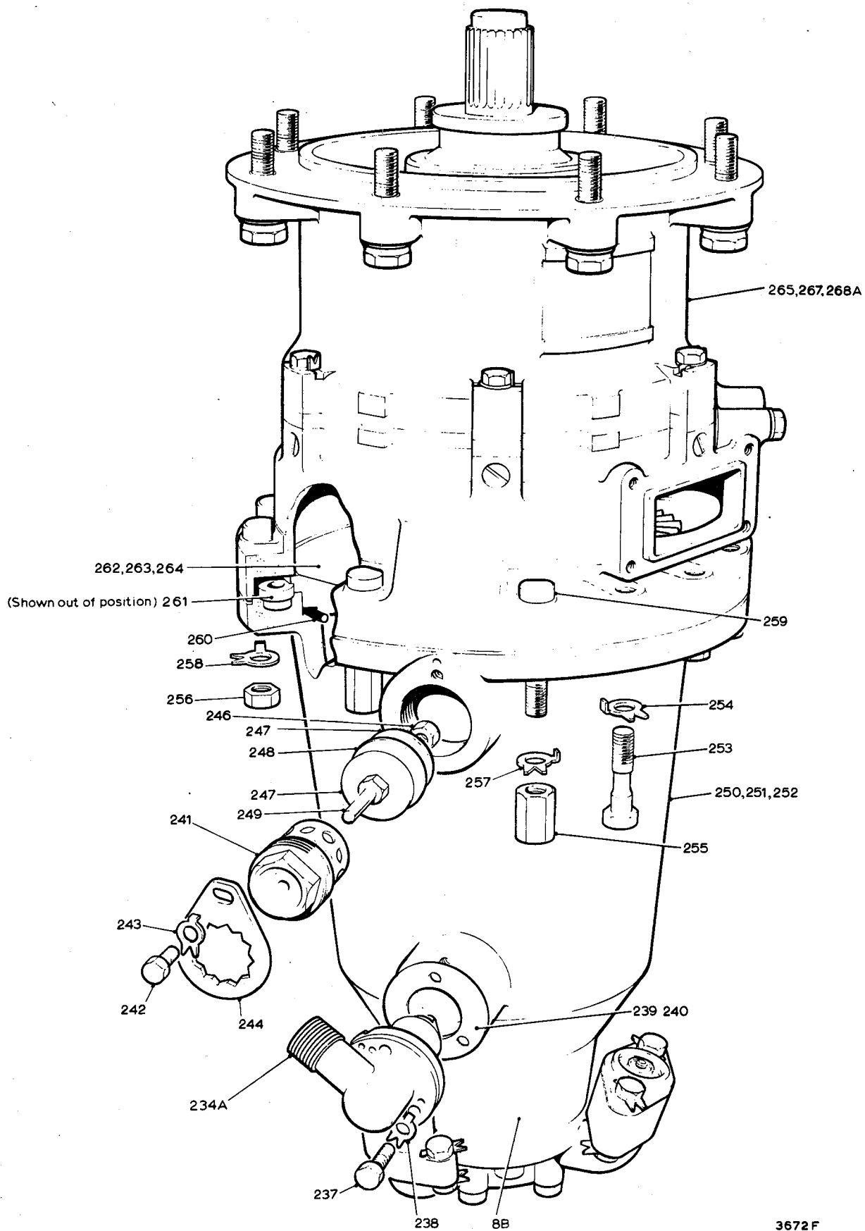
Fig.1 Starter Motor
