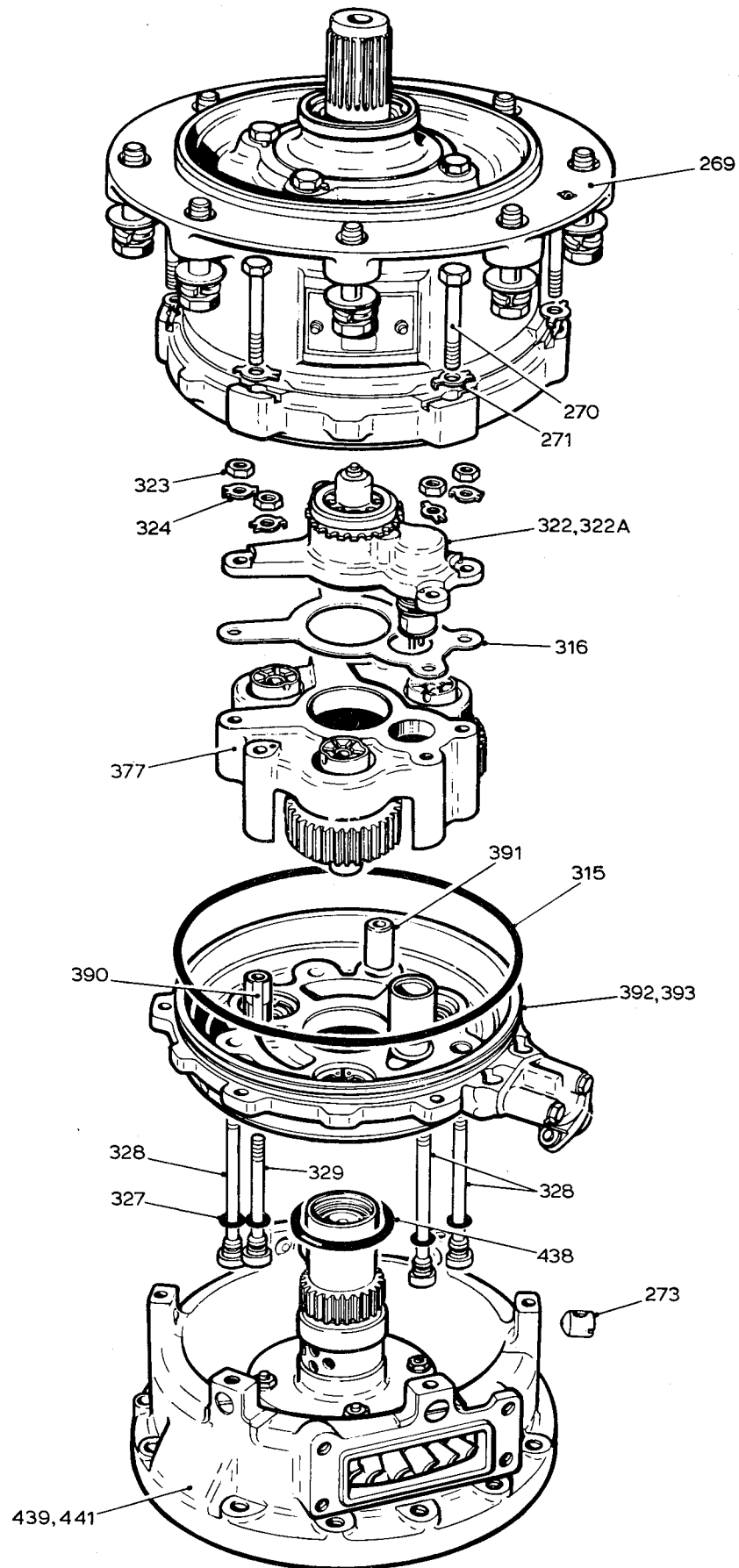
Fig.6 Gearbox assembly
