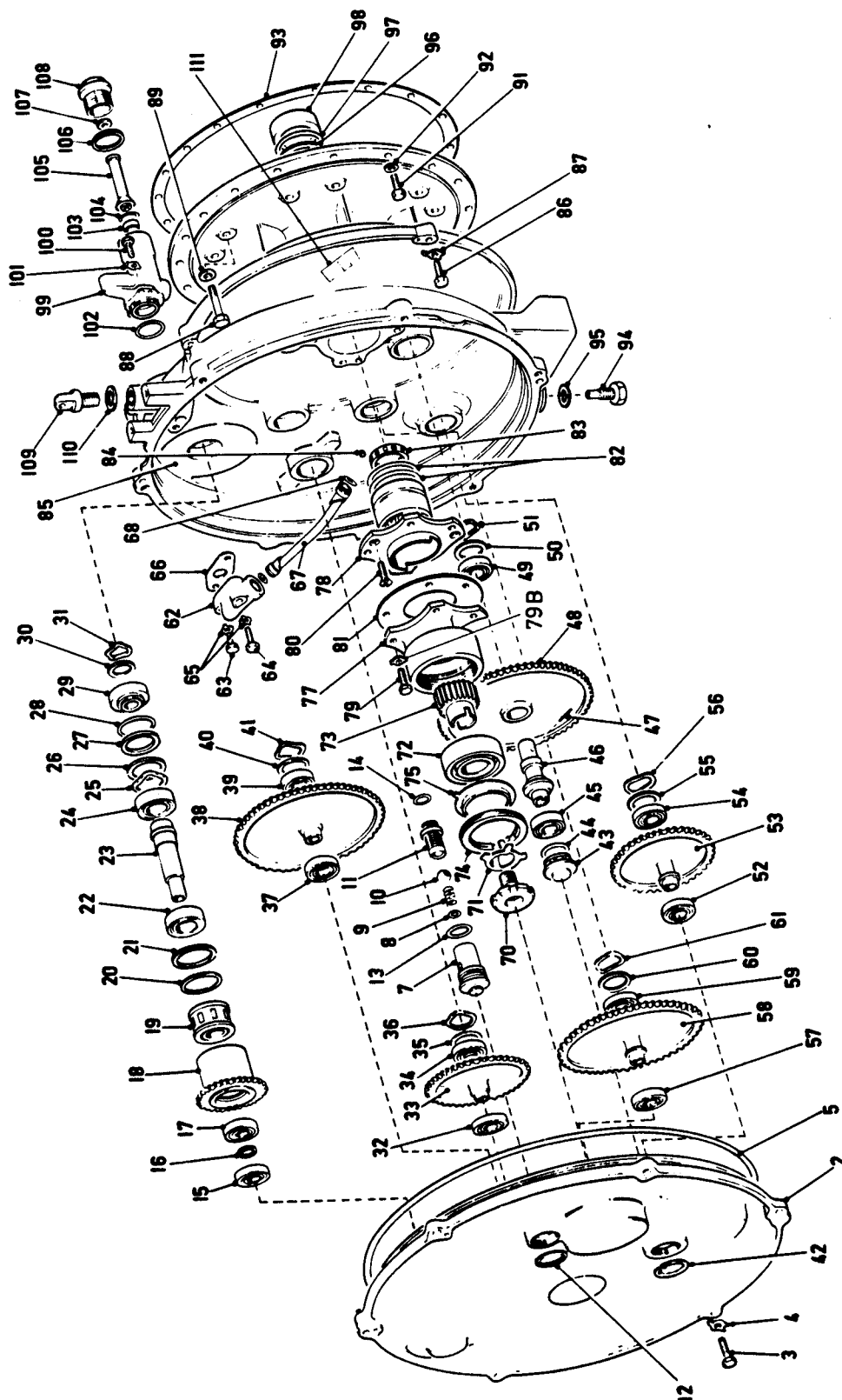
Fig.1 Gearbox, accessory
