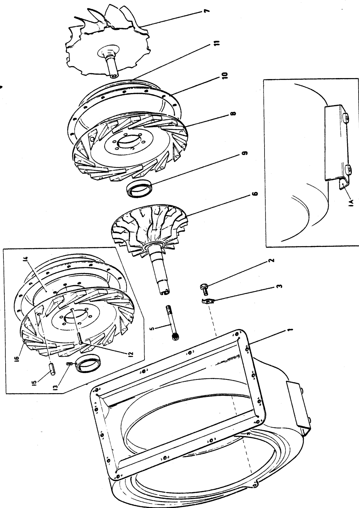
Fig. 2 Duct, air intake, and rotor, compressor
