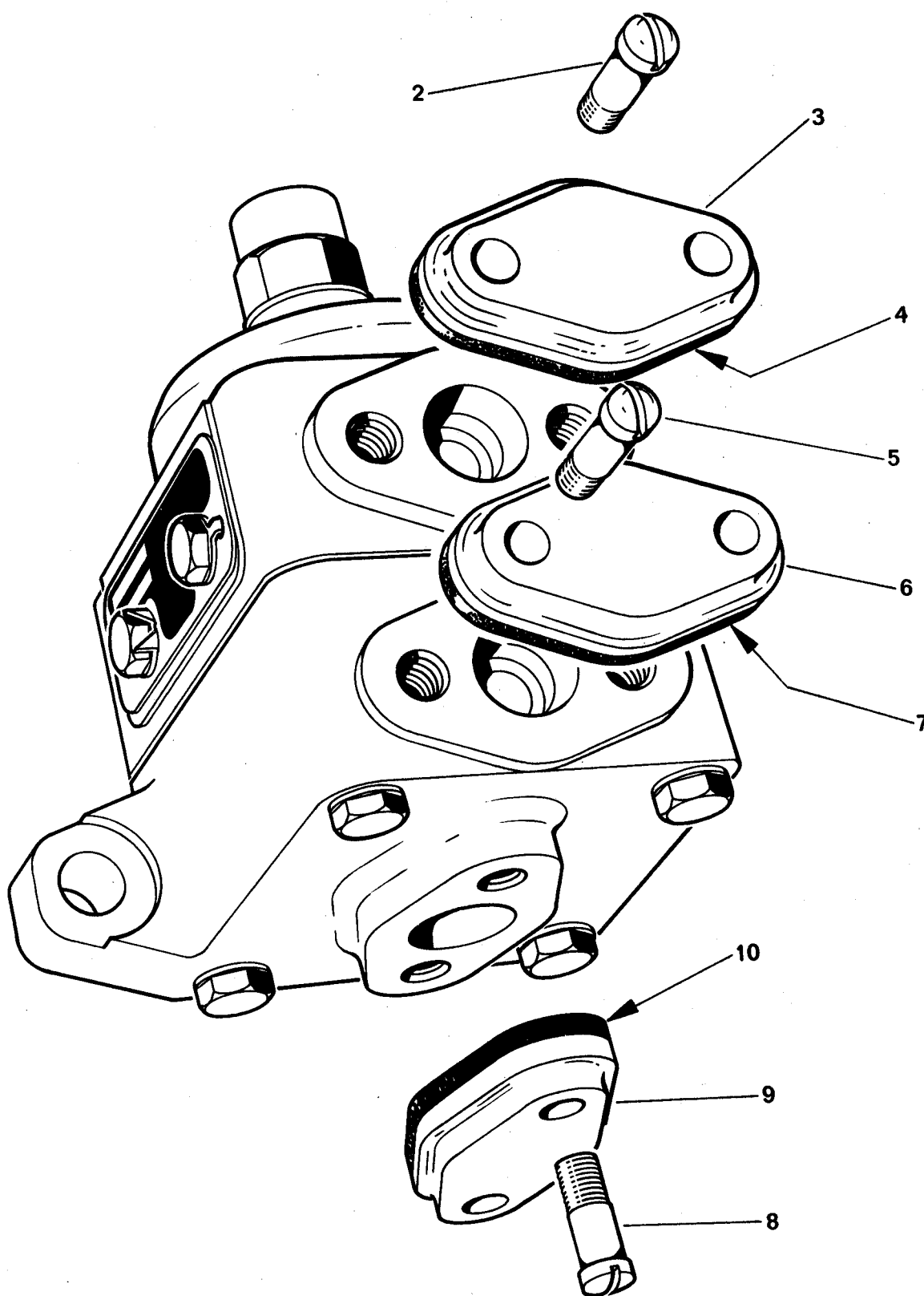
Fig.11 Valve, idling control:- storage items
