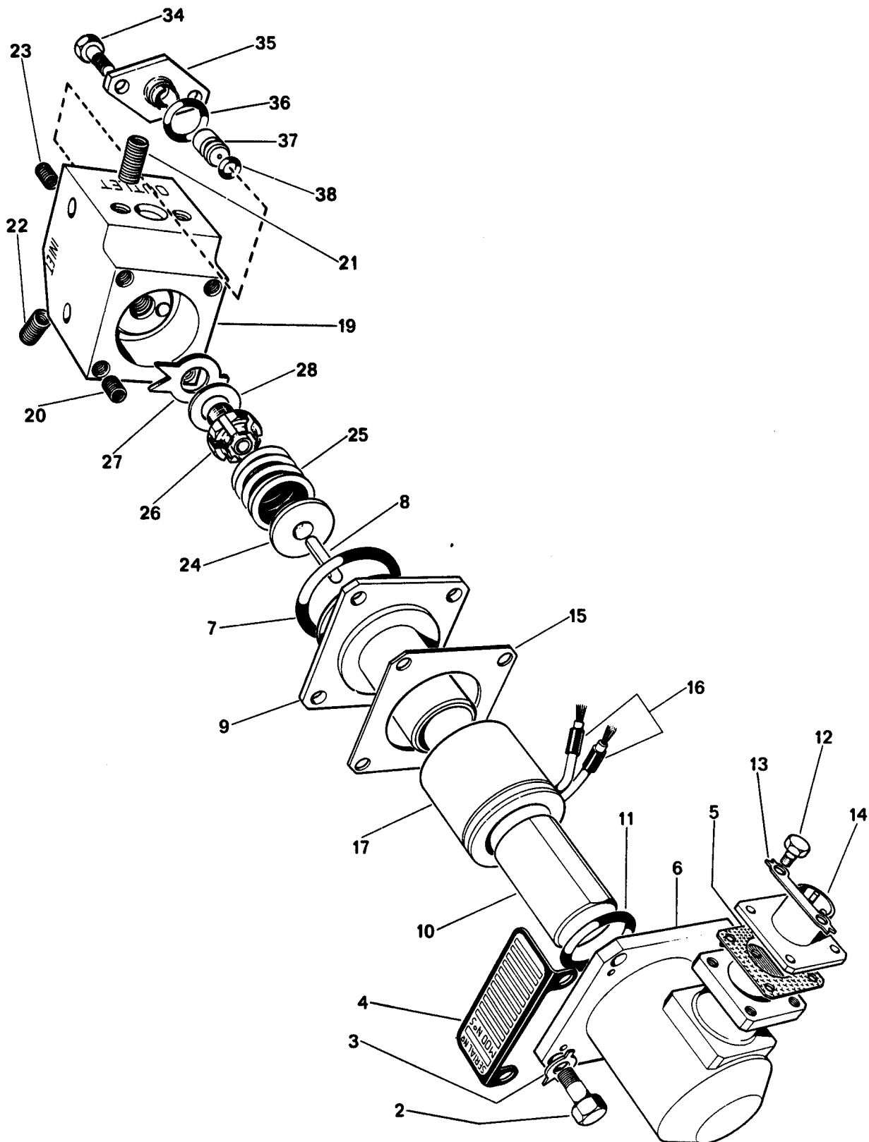
Fig.16 Valve, idle solenoid:- exploded view
