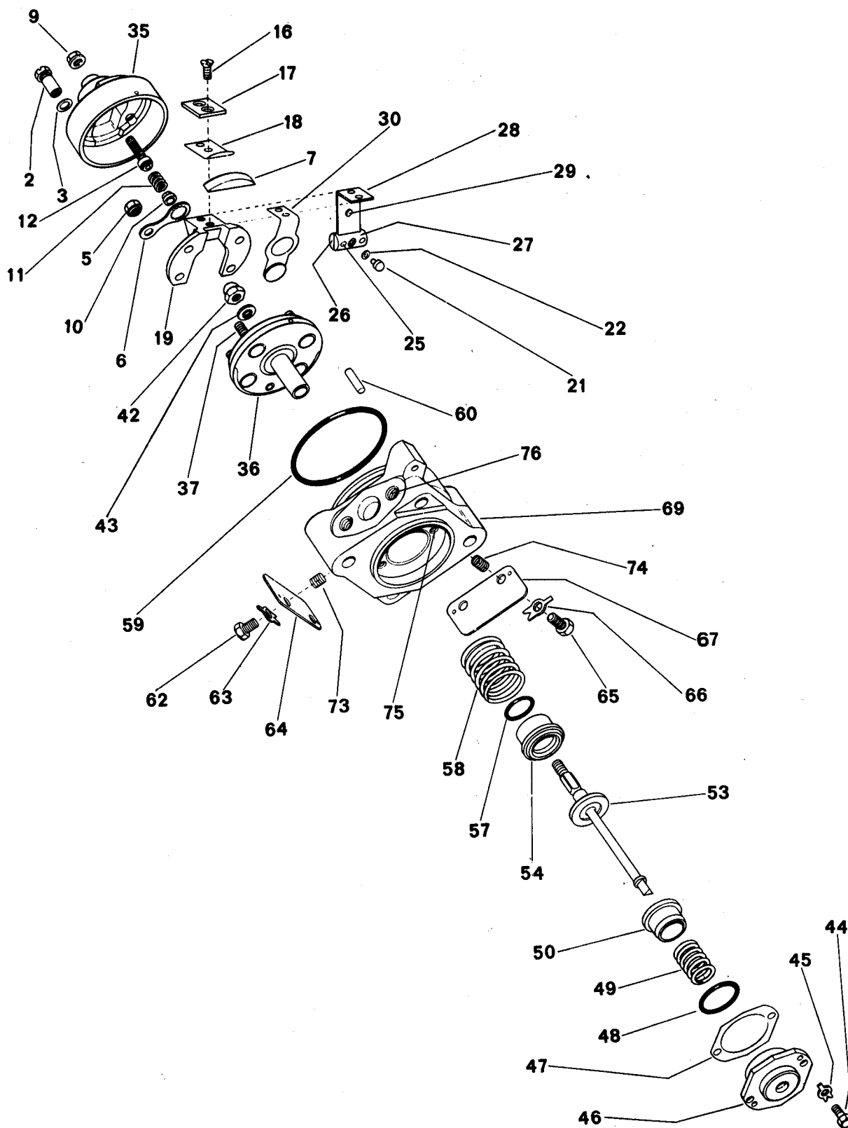
Fig. 9 Weights and shaft, balance
