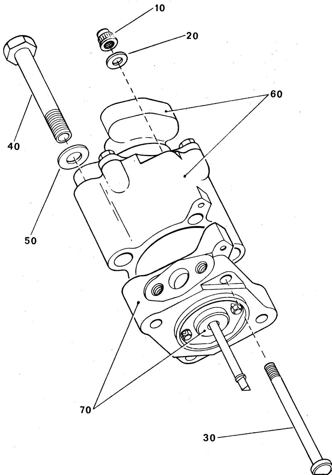
Fig. 7 Governor, APU
