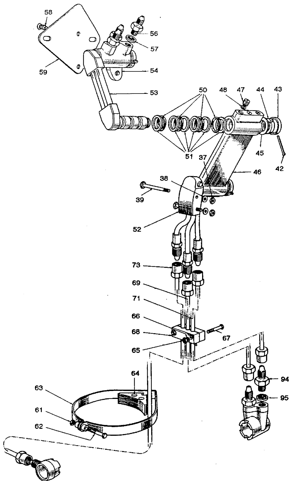
Fig 1 Main undercarriage (Sheet 3 of 6)
