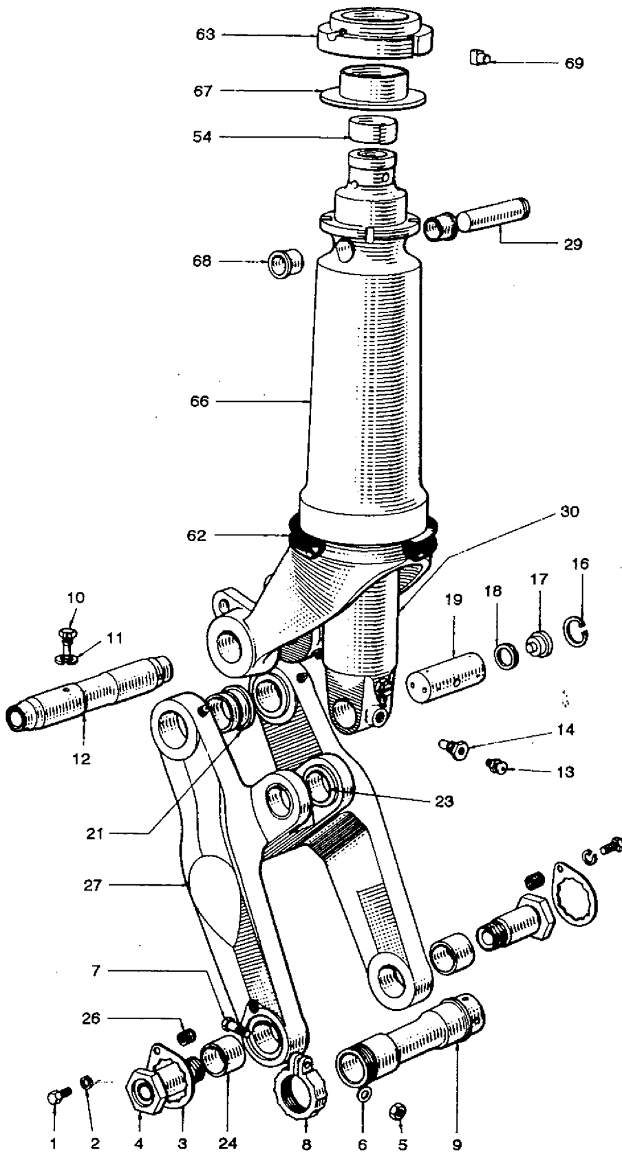
Fig 2 Nose undercarriage (Sheet 1 of 2)
