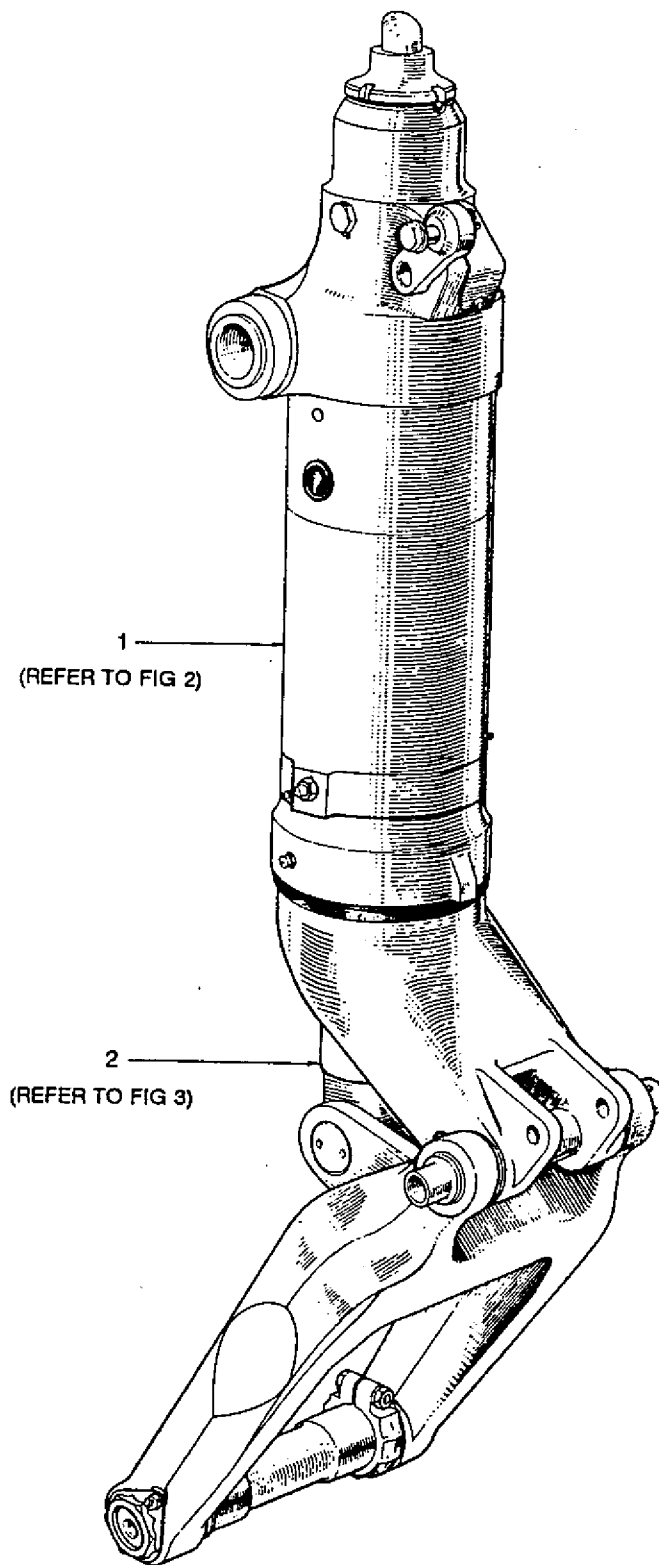
Fig 1 Nose undercarriage
