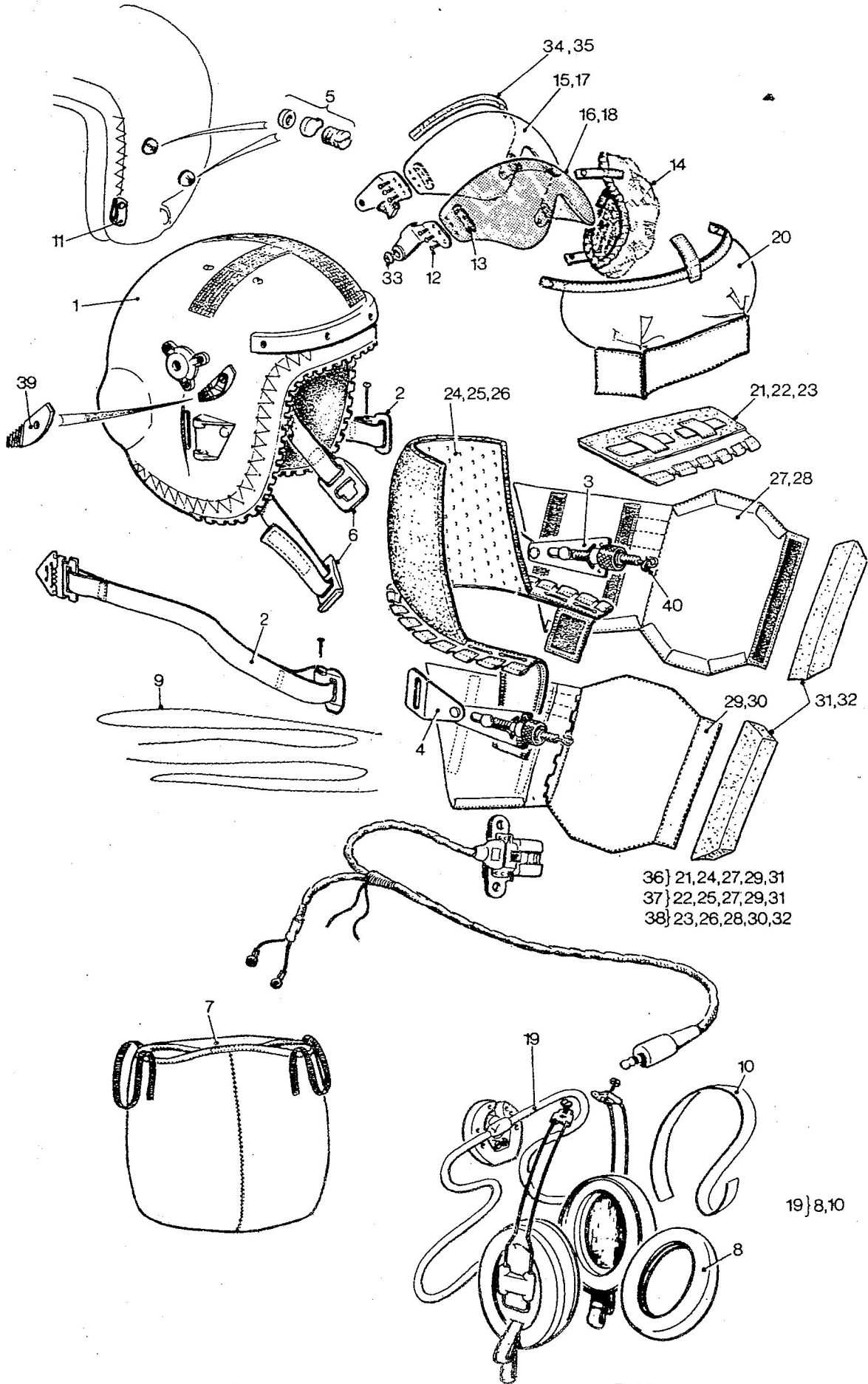
Fig 2 Exploded view of Mk 3C helmet
