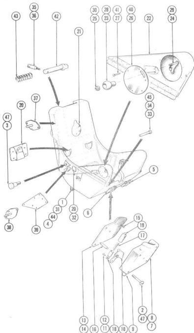
PAN - SEAT ASSY.
