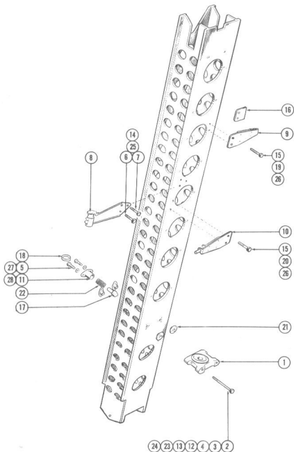
RAIL - GUIDE - ASSY.
