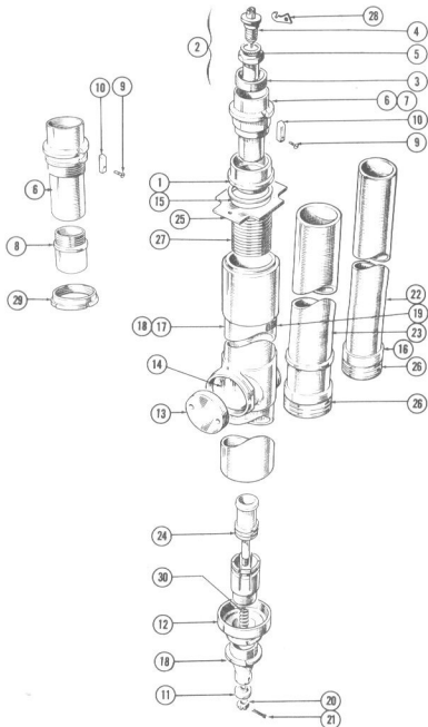
GUN - EJECTION ASSY.
