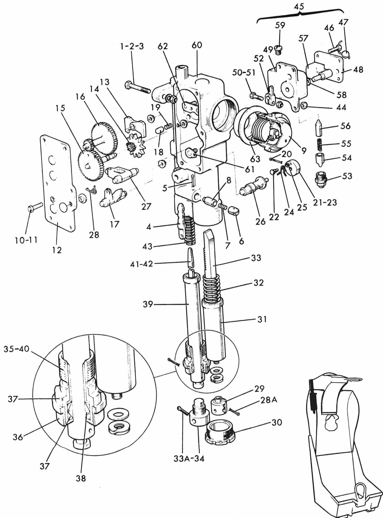
Figure 13. Time Release Assembly
