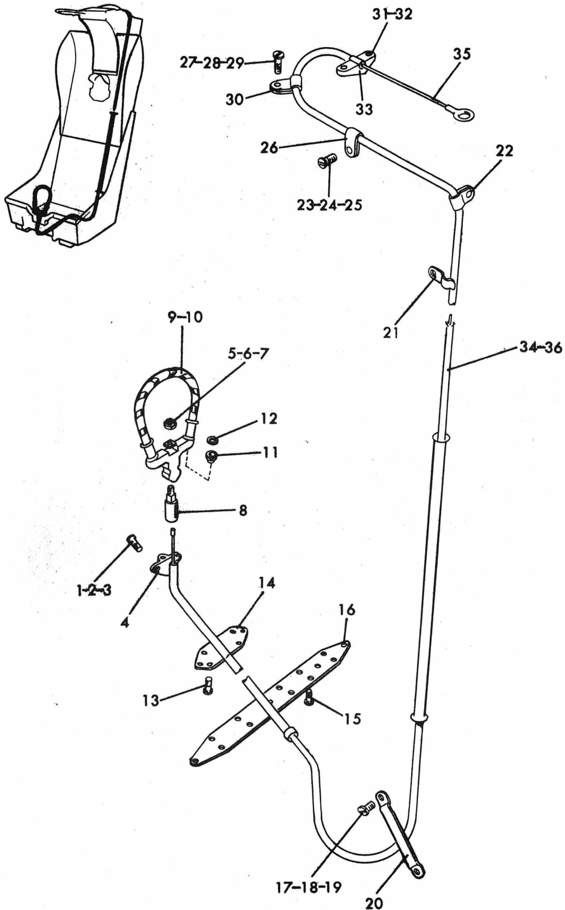
Figure 17. Alternative Firing Cable Assembly
