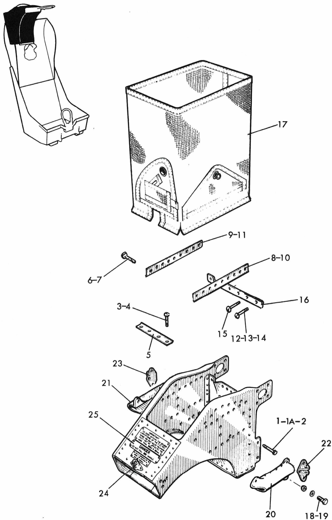
Figure 18. Drogue Container Assembly
