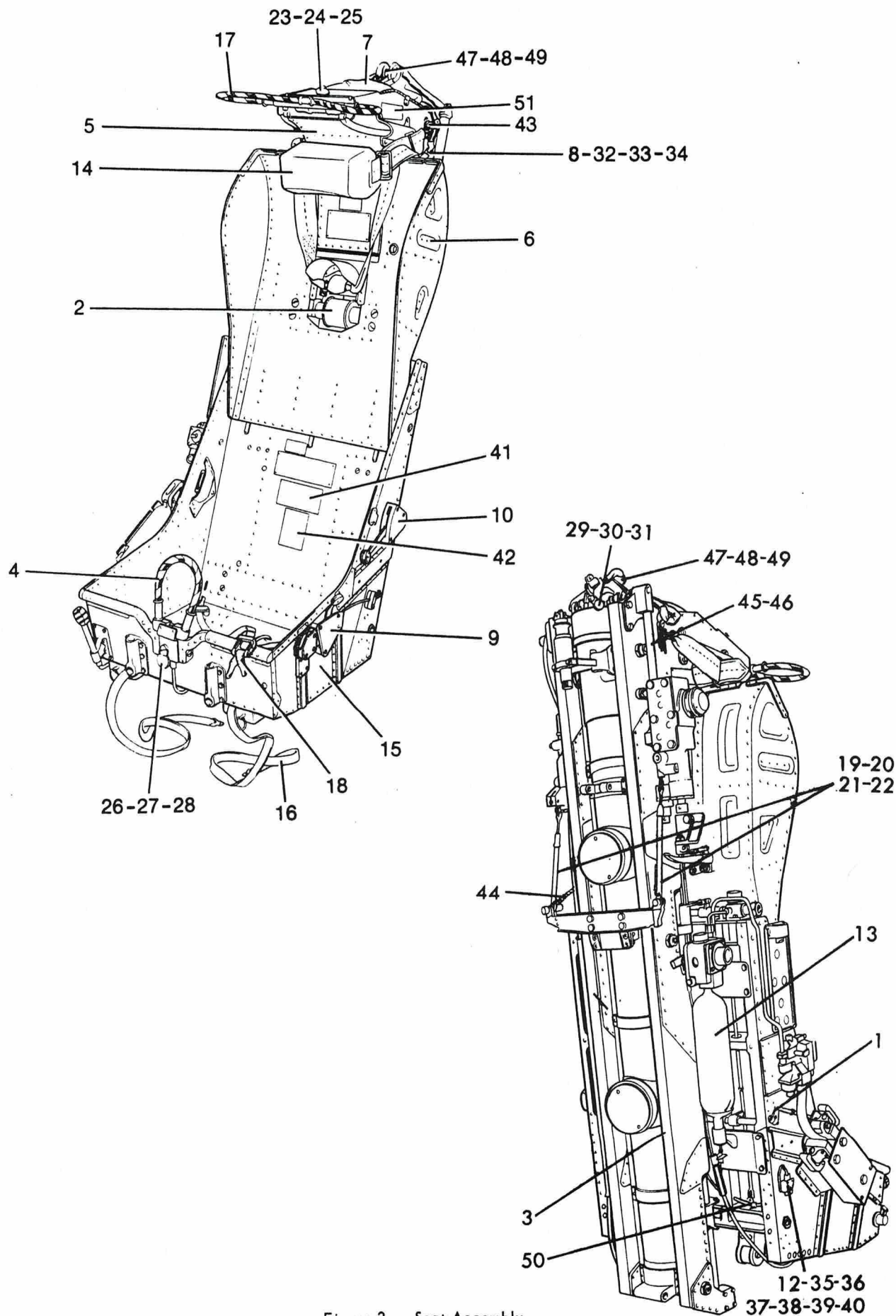
Figure 2. Seat Assembly
