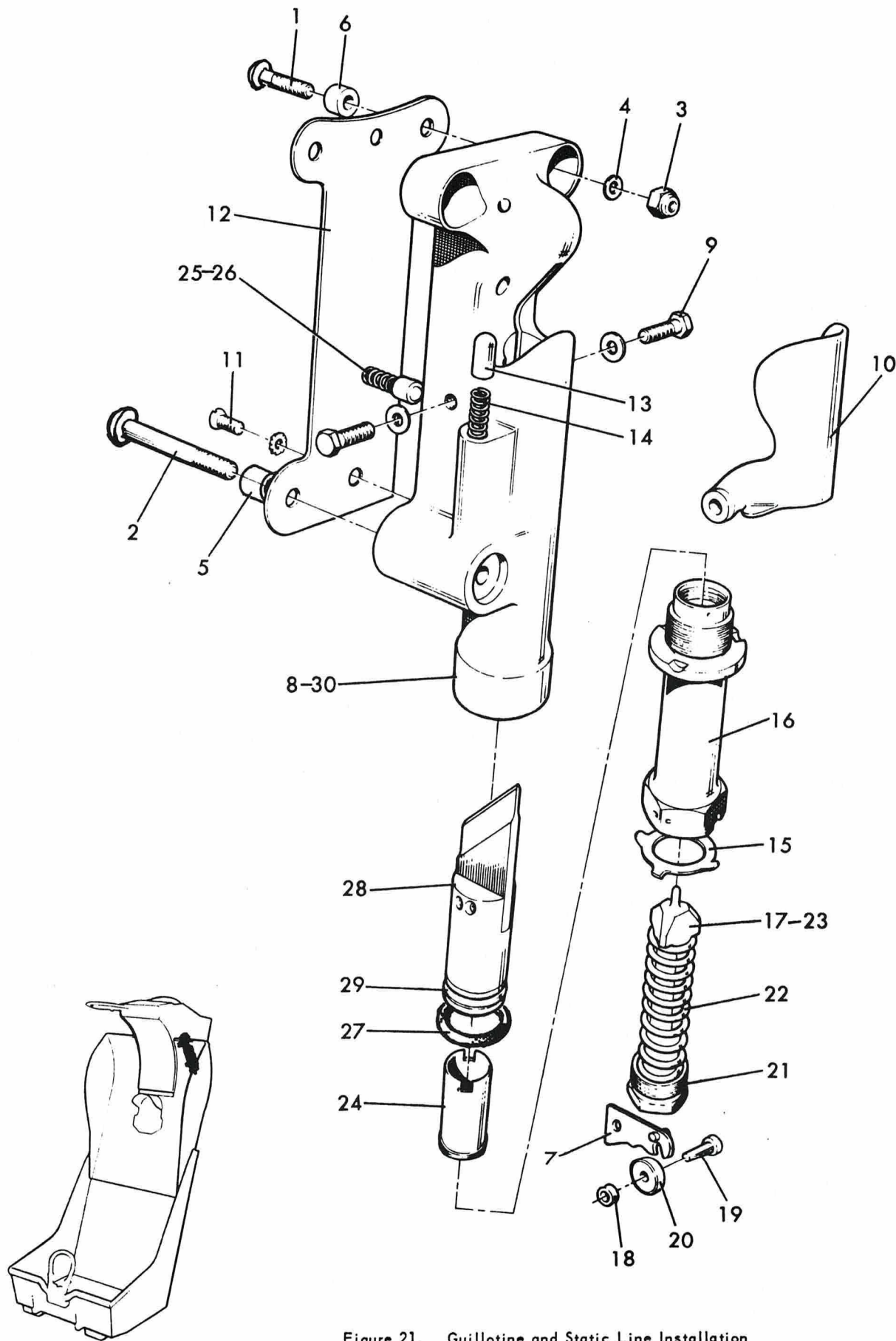
Figure 21. Guillotine and Static Line Installation
