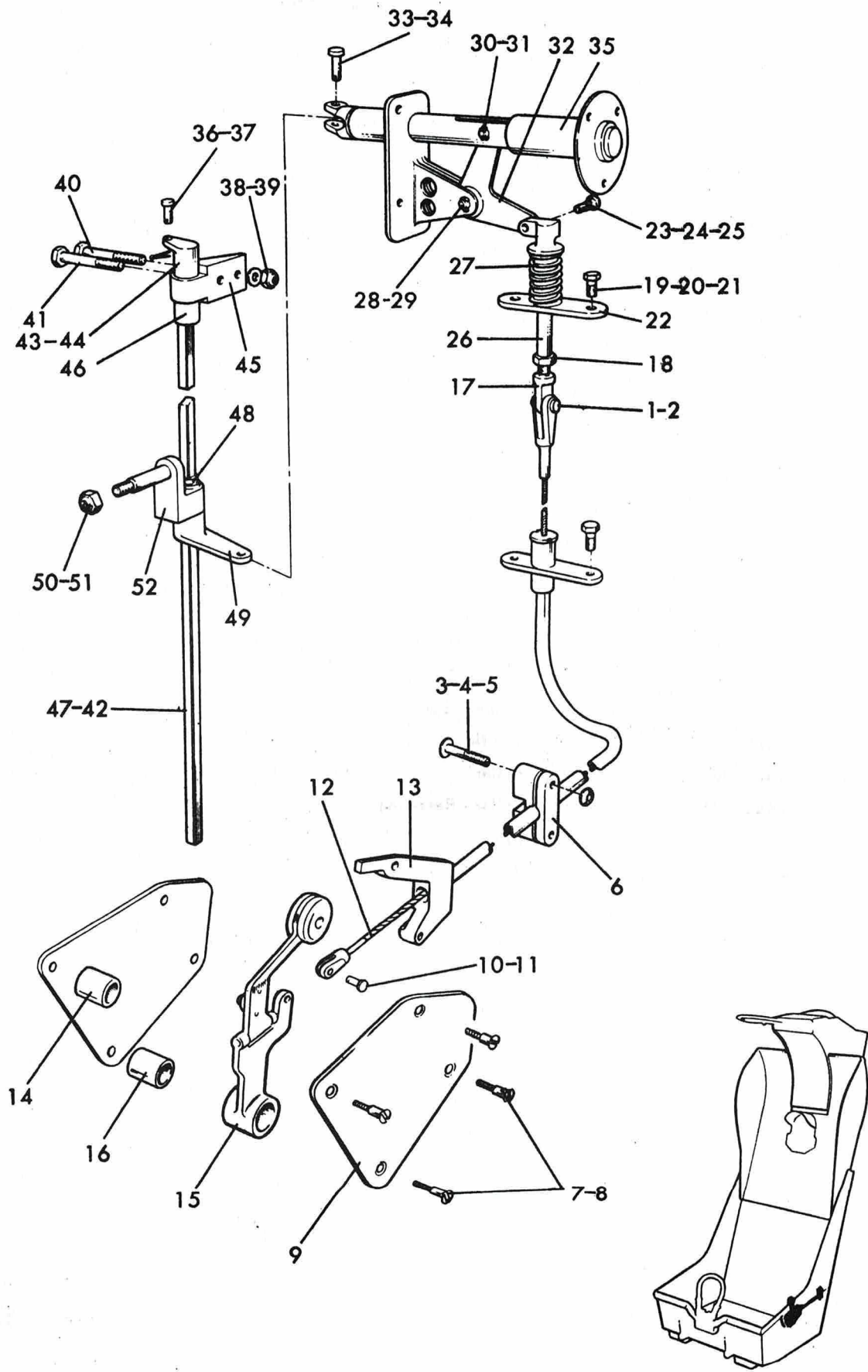
Figure 22. Harness Release Mechanism Assembly
