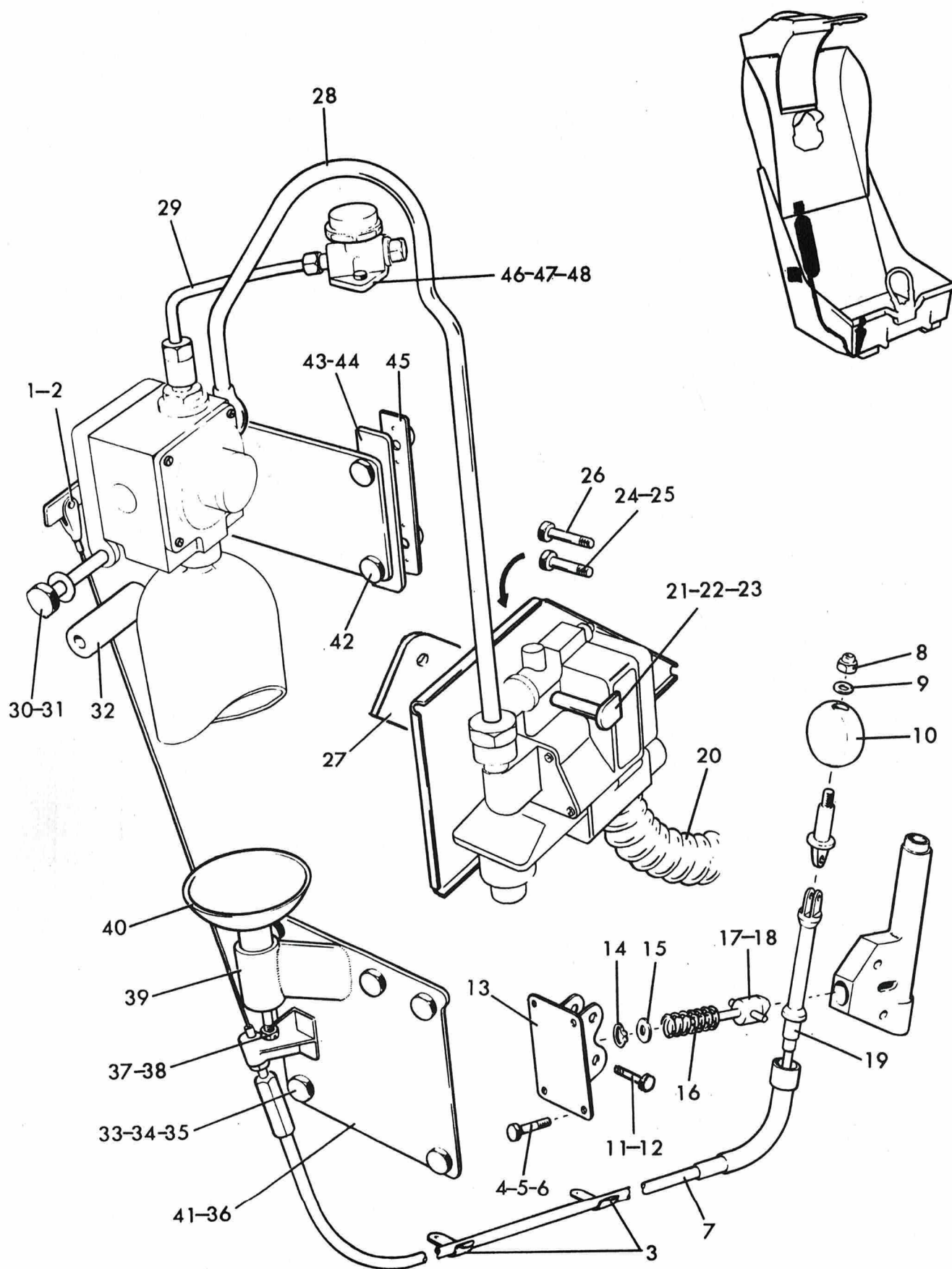
Figure 26. Emergency Oxygen Assembly
