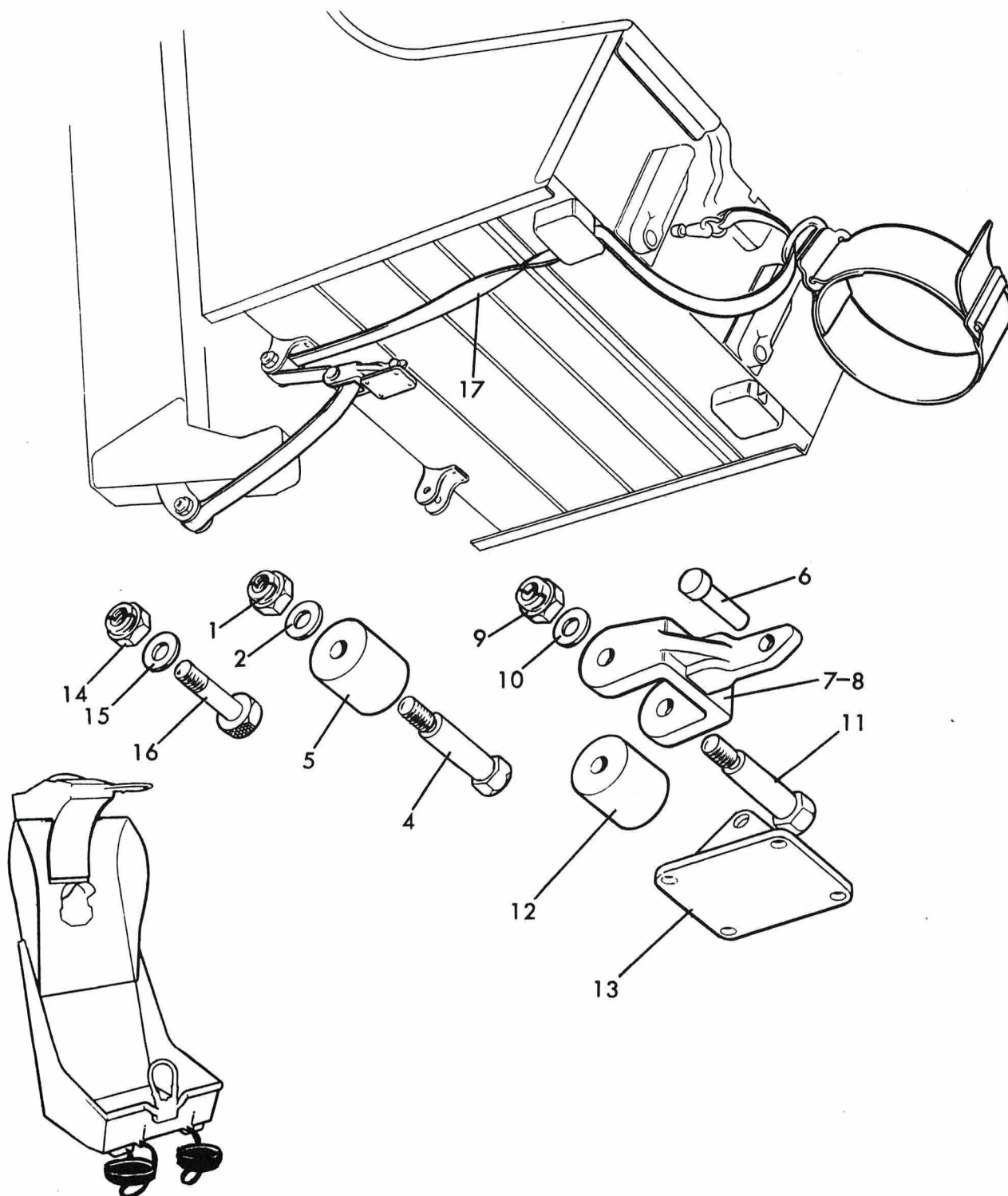
Figure 29. Leg Restraint Assembly
