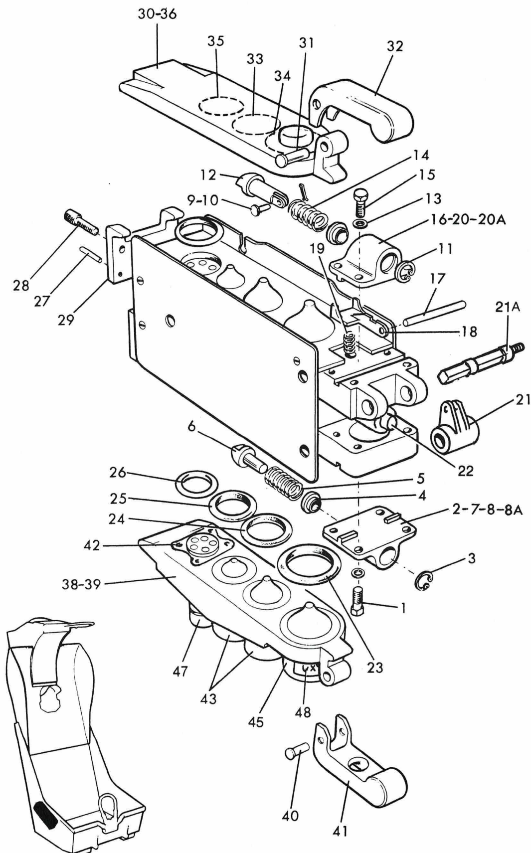
Figure 5. Centre Body Assembly
