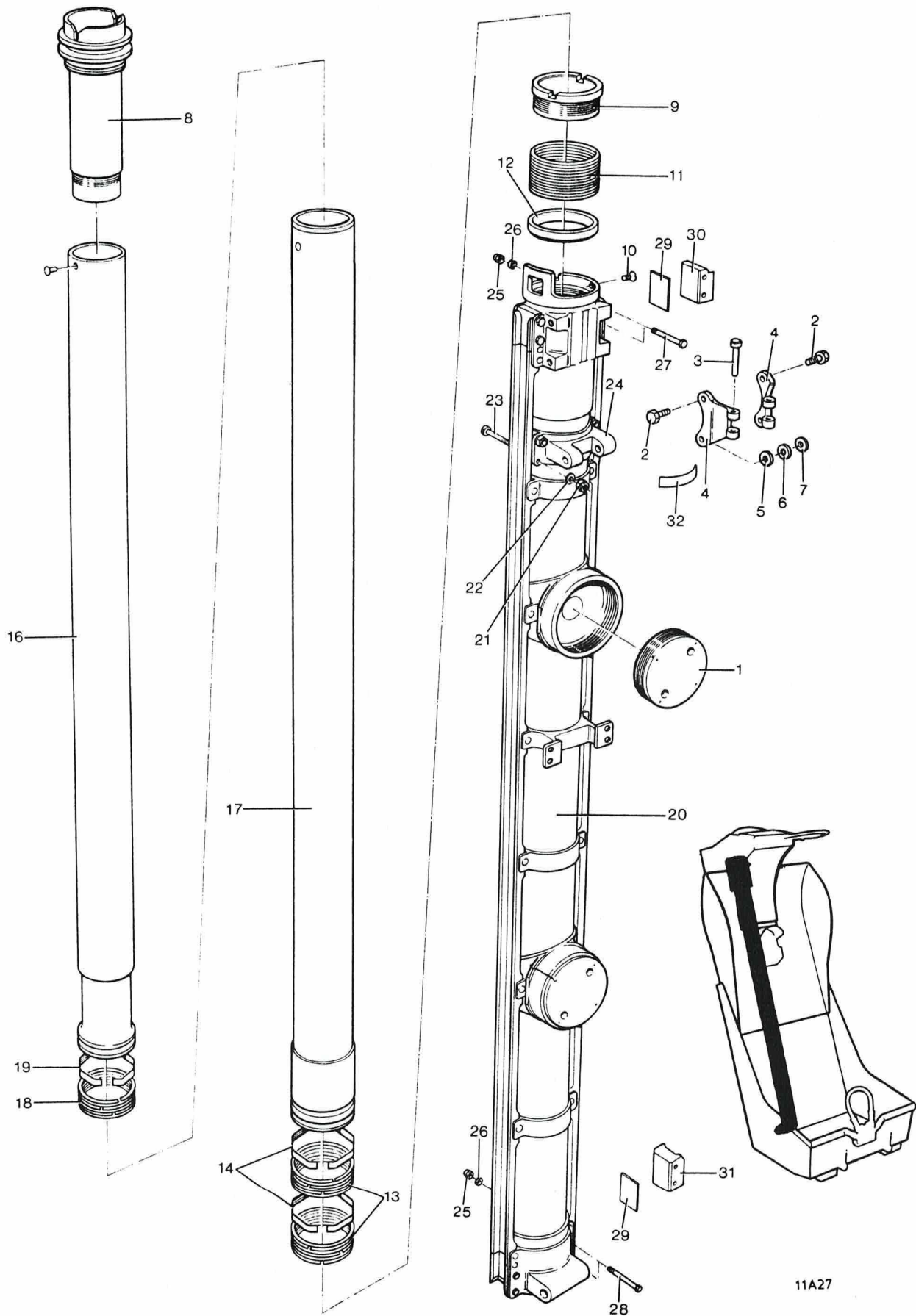
Figure 7 Gun and guide rail assembly
