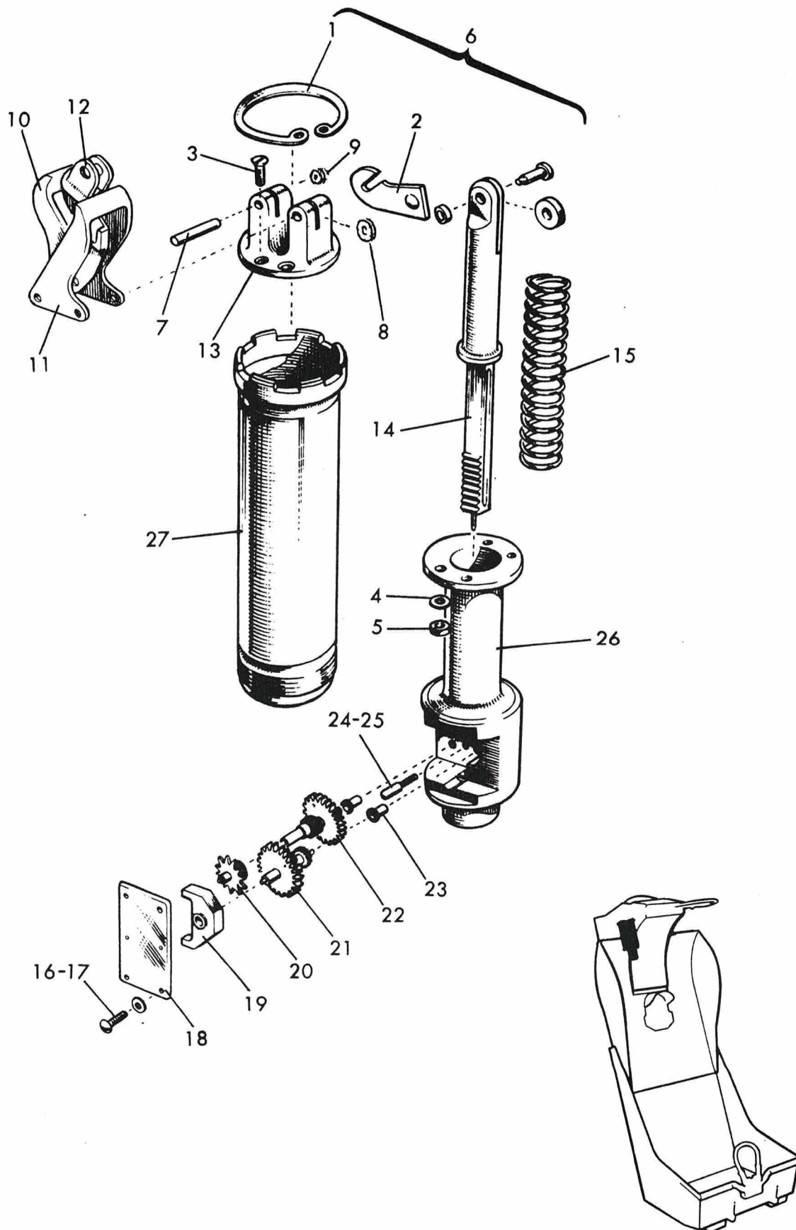
Figure 8. Time Delayed Firing Mechanism
