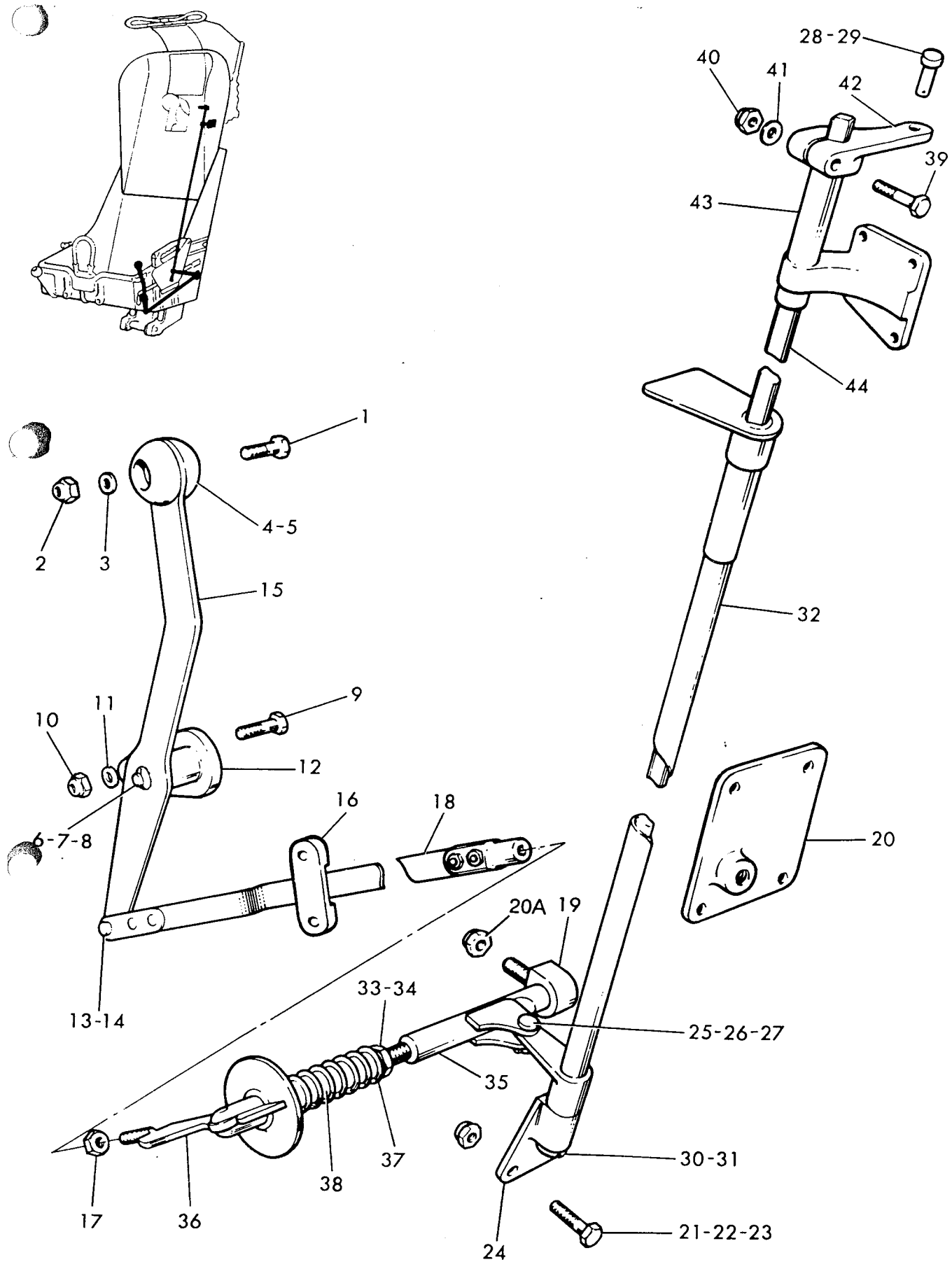
Fig 17 Go-Forward Mechanism Assembly
