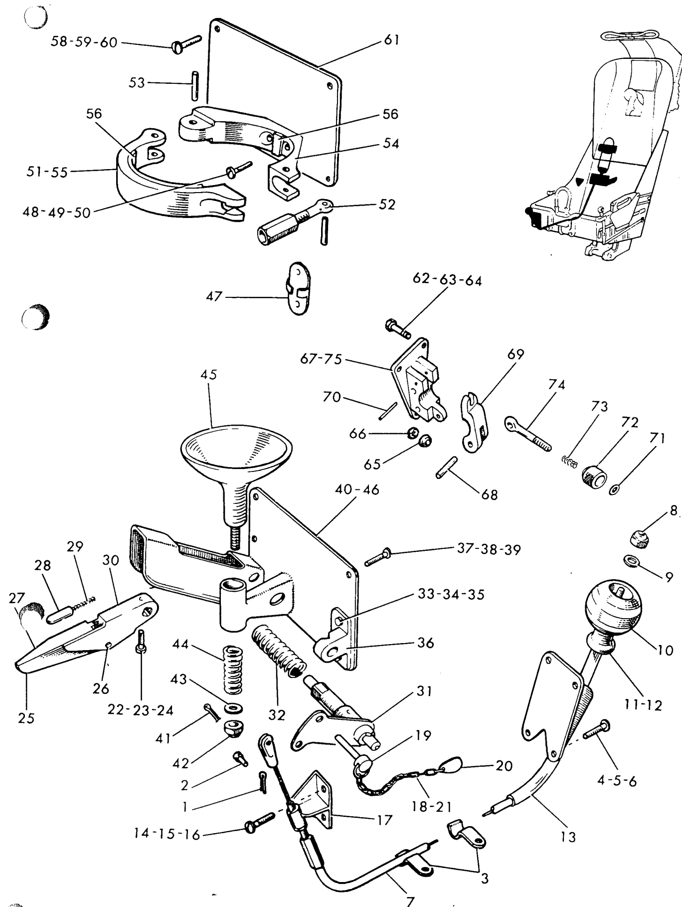
Fig 22 Emergency Oxygen System Assembly
