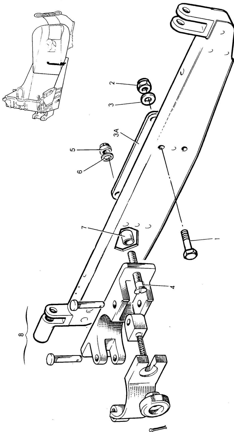
Fig 3 Cross Beam Assembly
