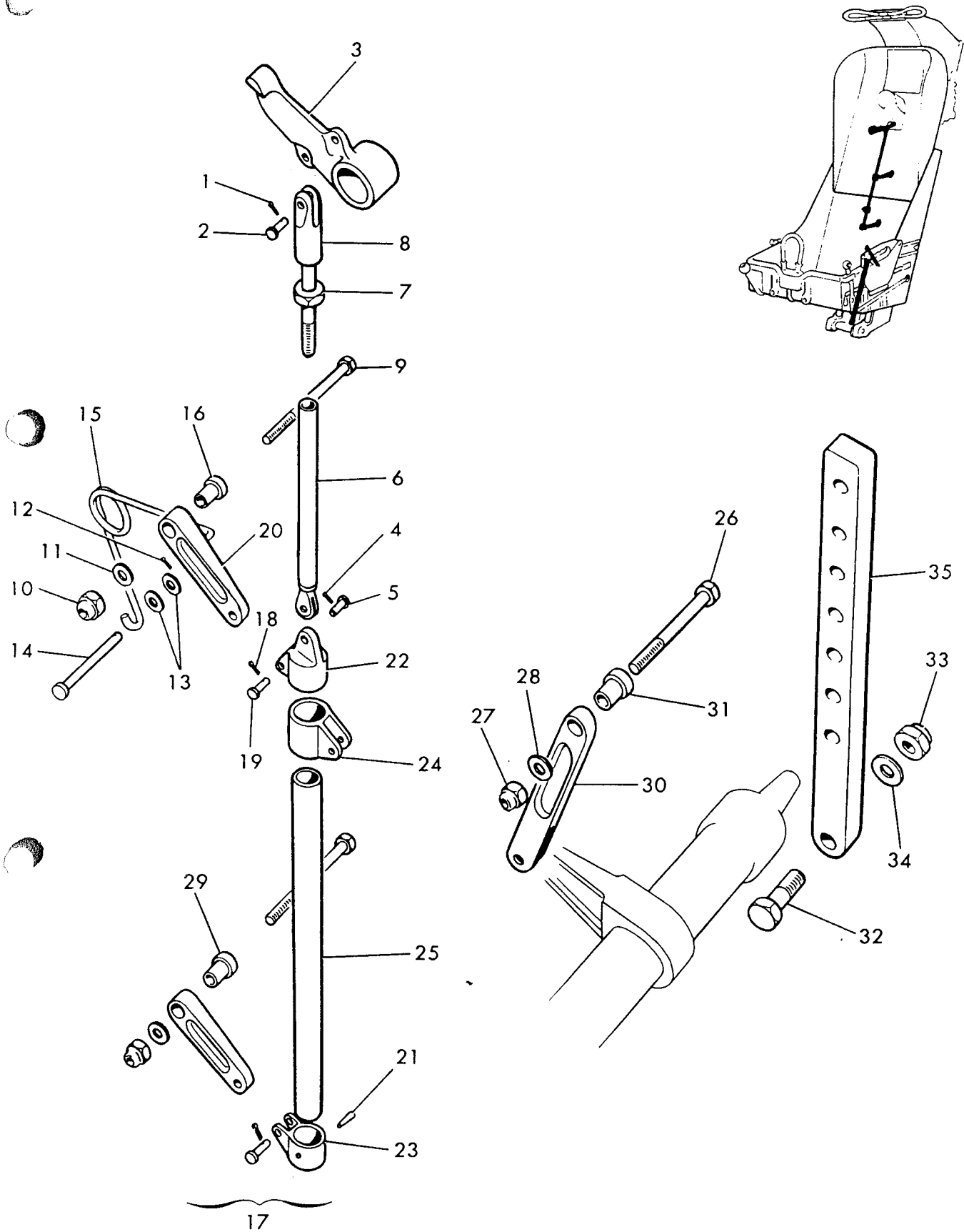
Fig 20 Parallel Motion and 40G Harness Mechanism Assembly
