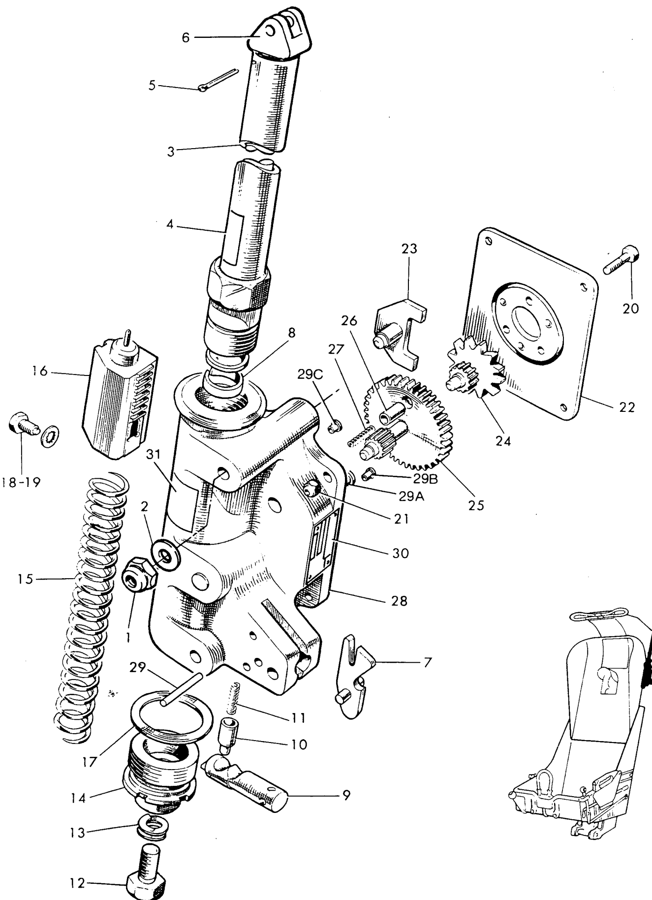
Fig 4 Drogue Gun Assembly
