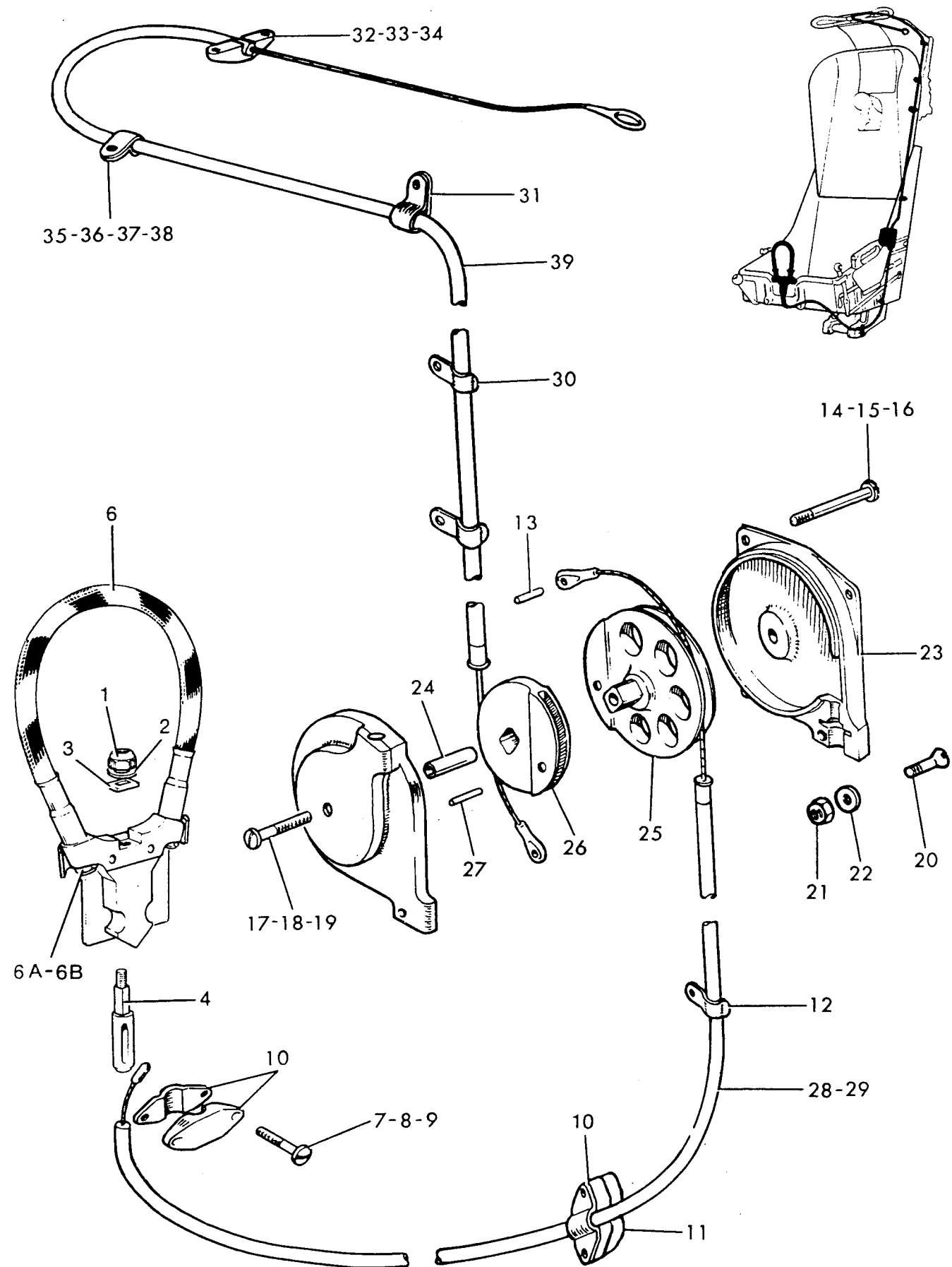
Fig 26 Alternative Firing Run Assembly
