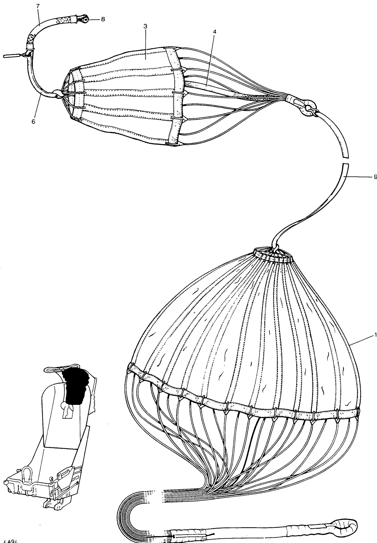
Fig 14 Drogue Duplex Assembly
