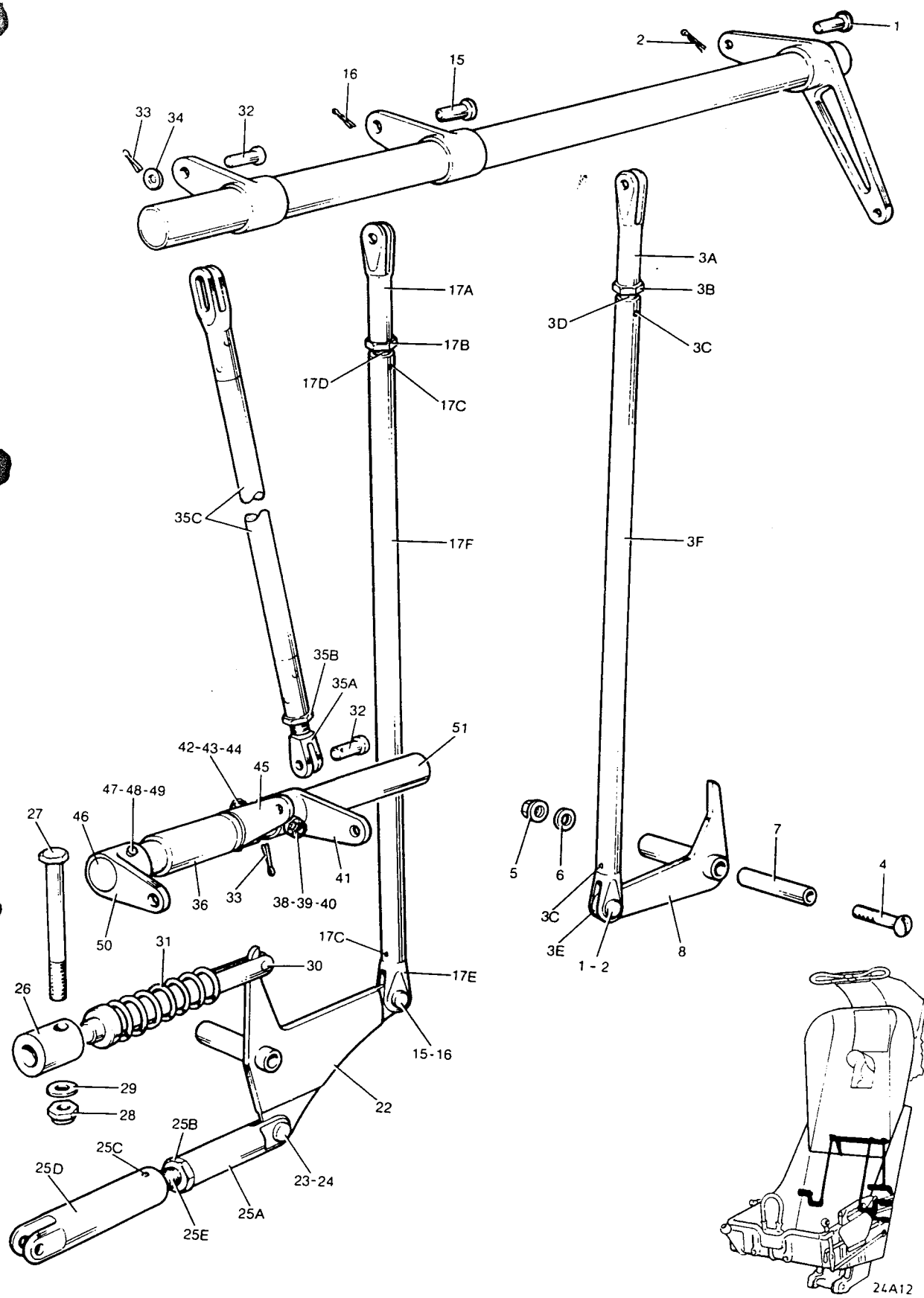
Fig 18 Manual Override & Harness Release Mechanism Assembly
