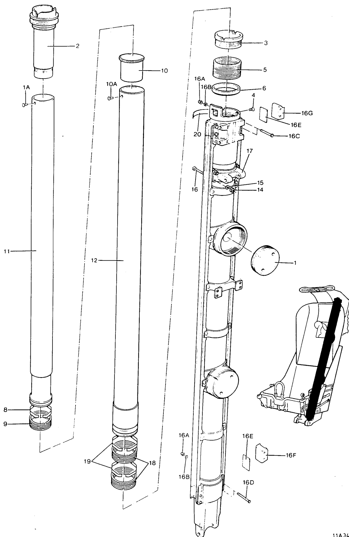
Fig 5 Gun and Guide Rail Assembly
