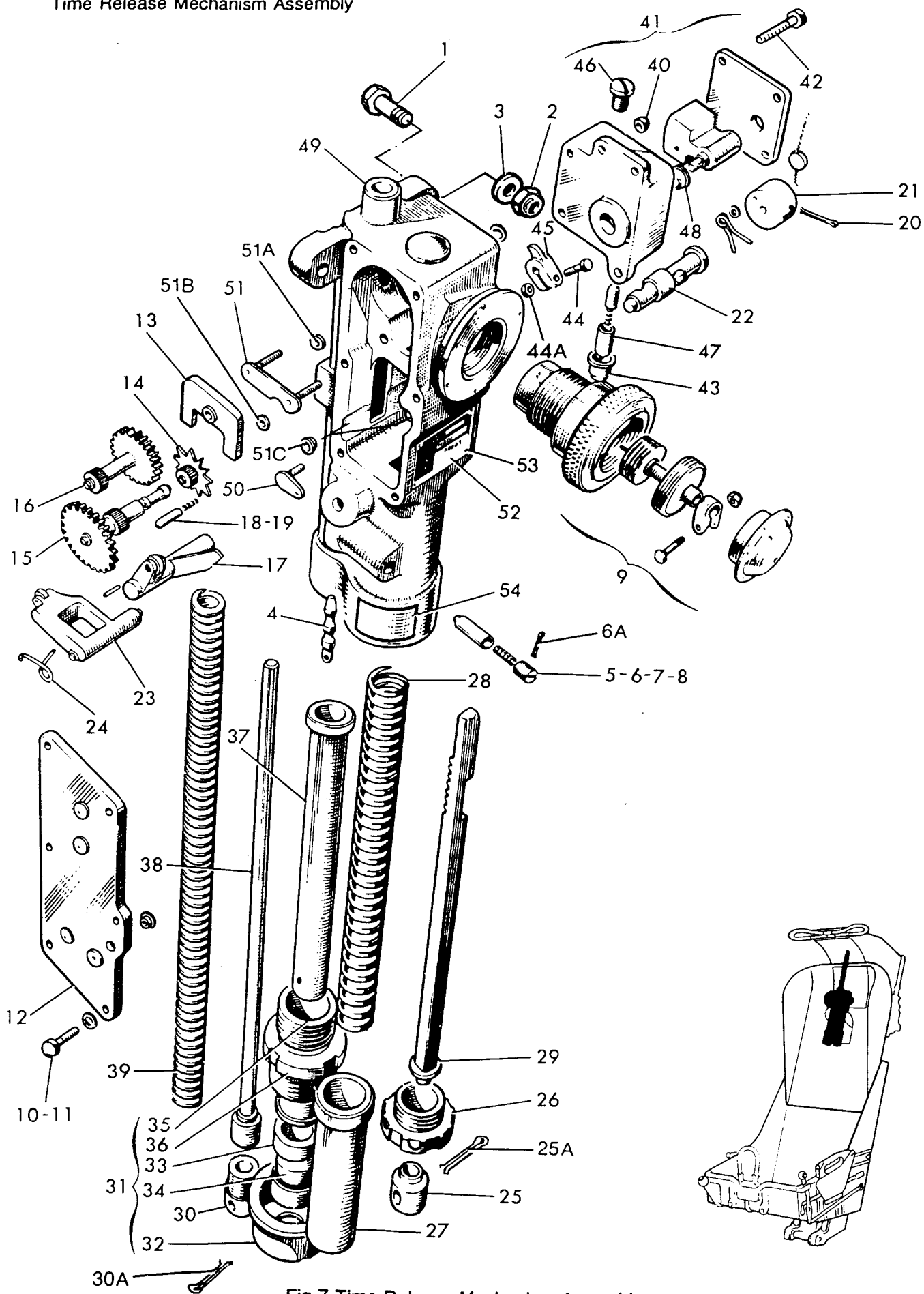
Fig 7 Time Release Mechanism Assembly
