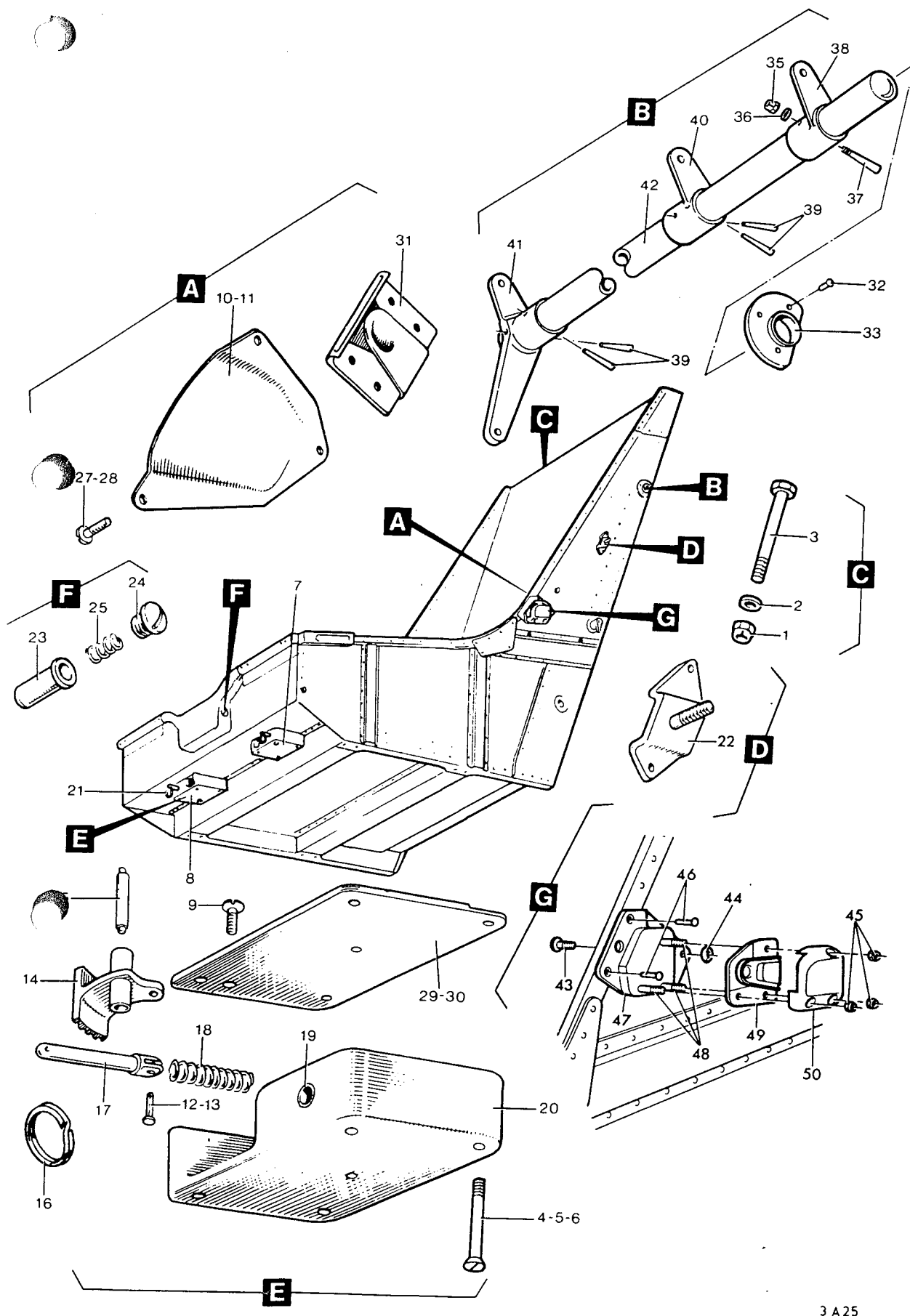
Fig 25 Seat Pan Assembly
