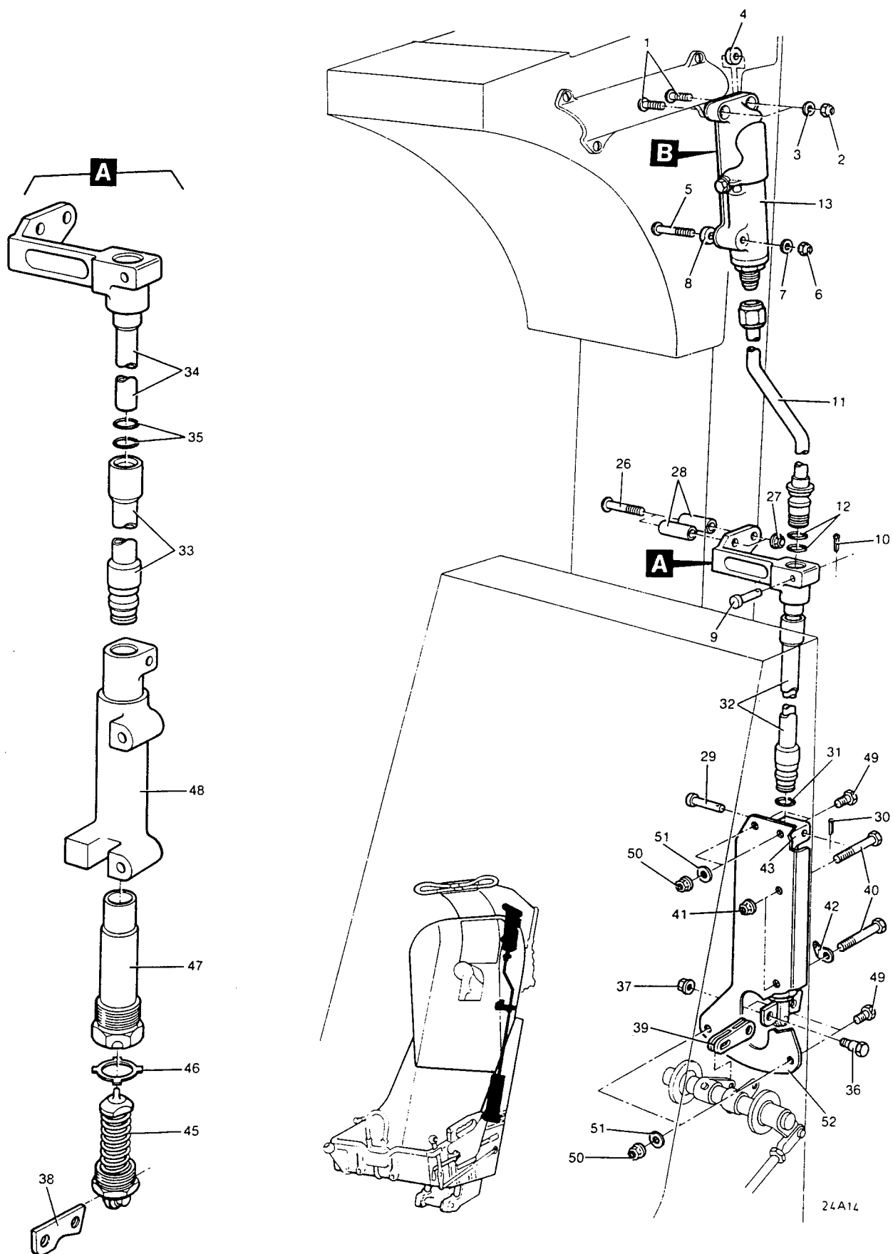
Fig 15 Guillotine Gas Fired Assembly (Sheet 1 of 2)
