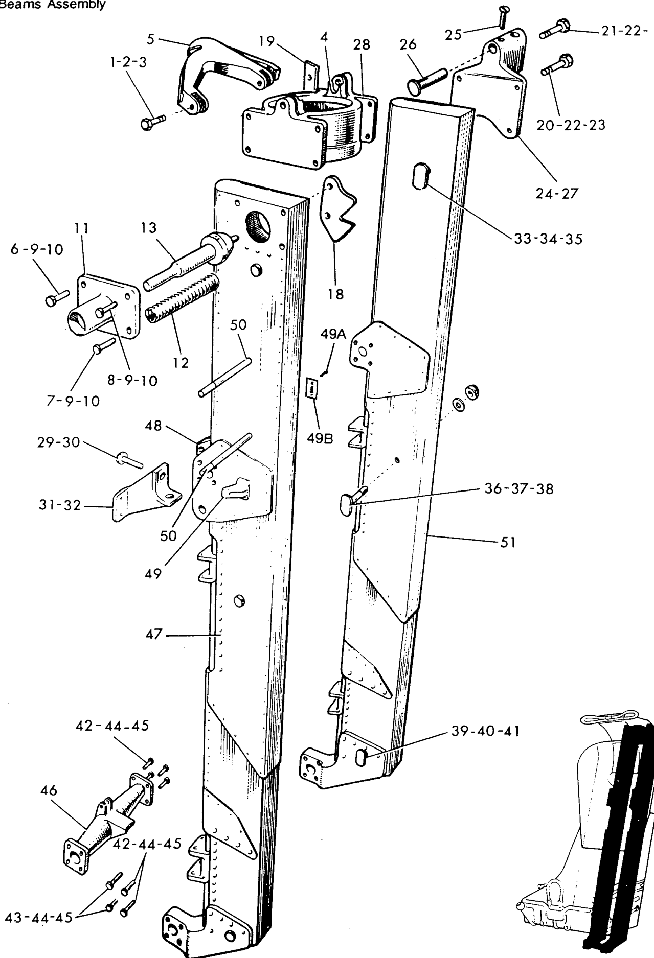
Fig 11 Main Beams Assembly
