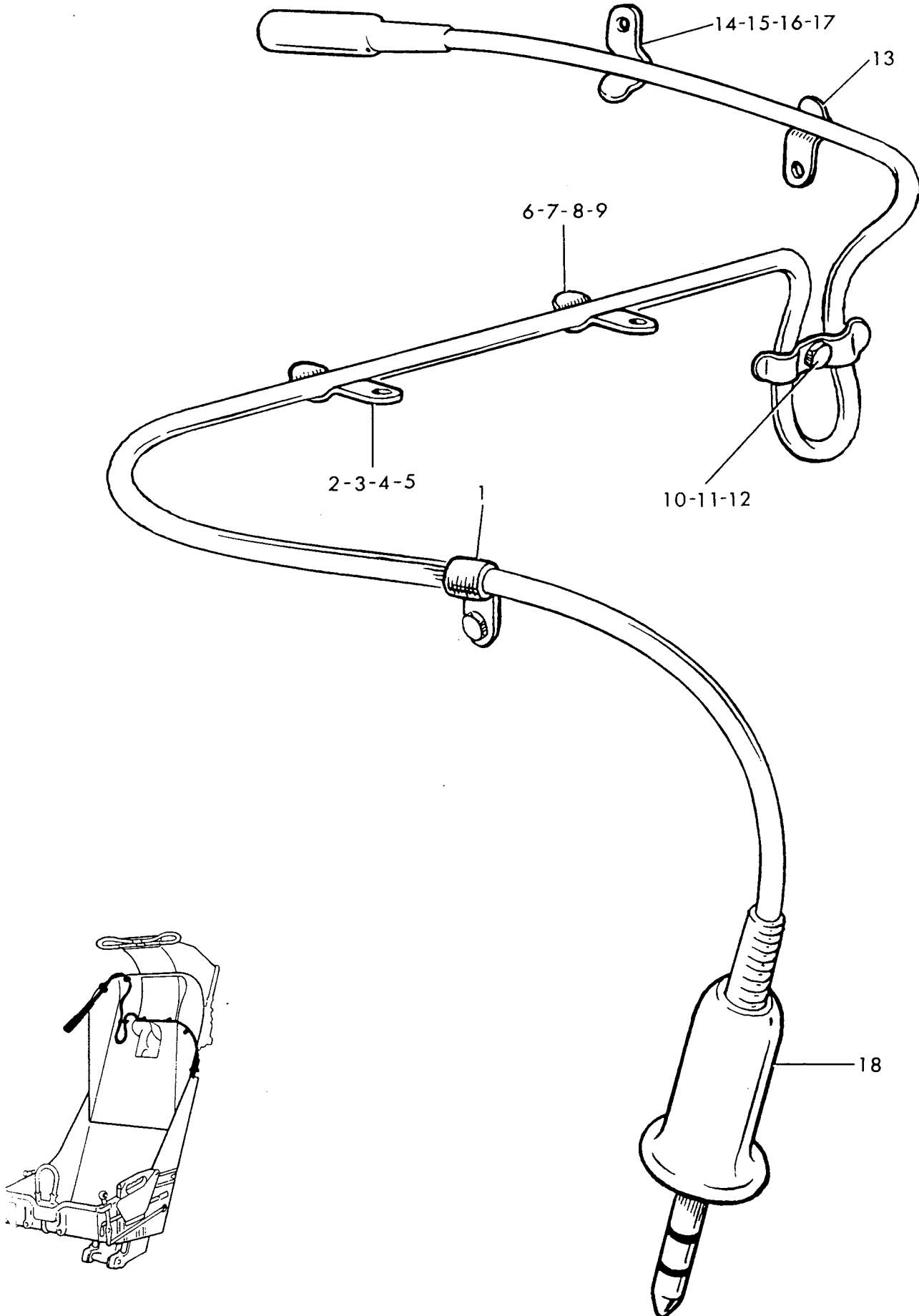
Fig 27 Tele-Mic Run Assembly
