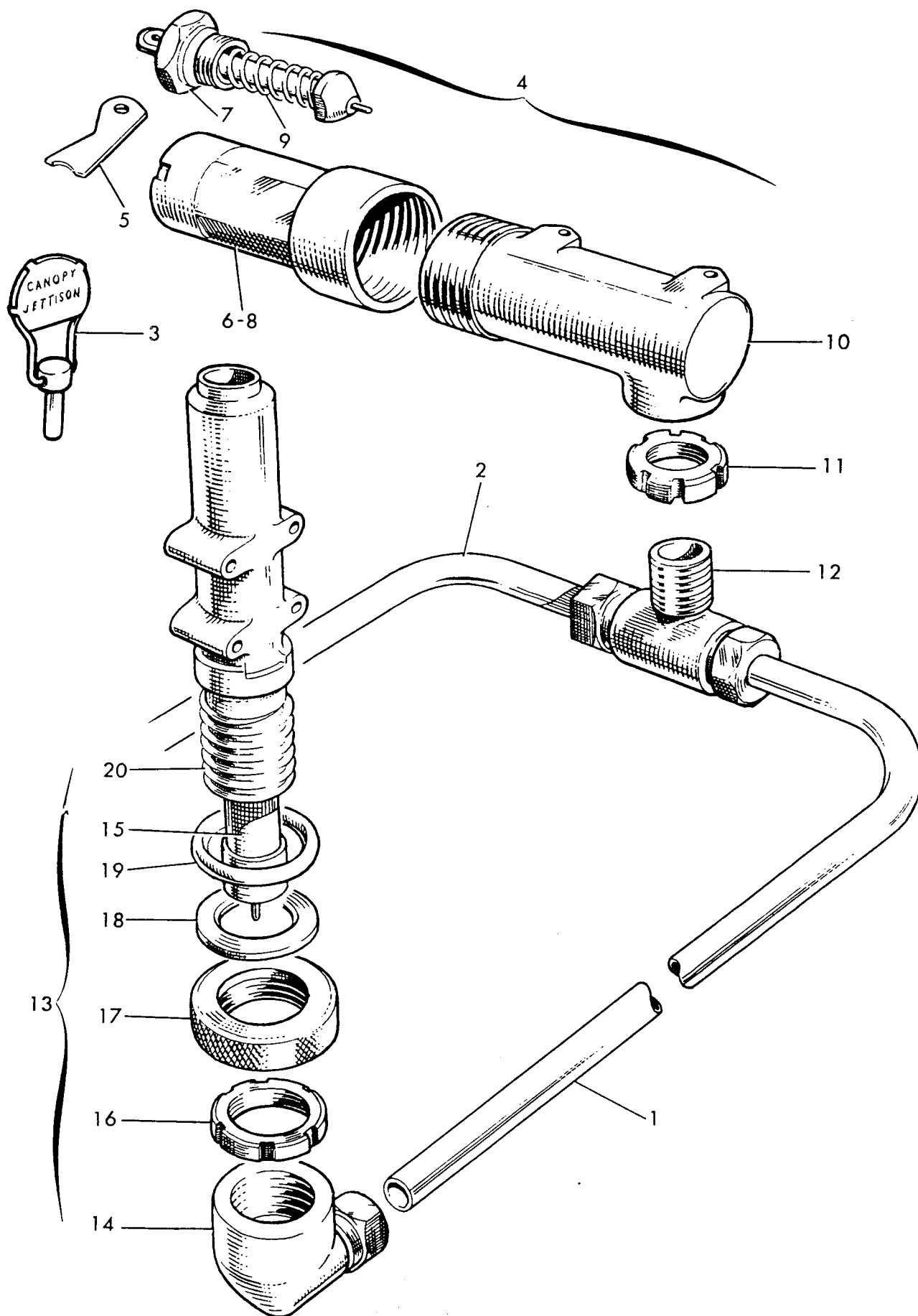
Fig 8 Canopy Jettison System
