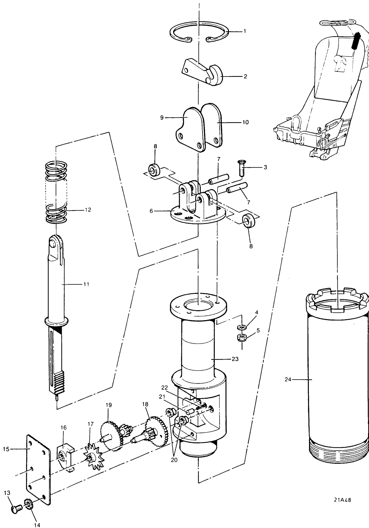
Fig 6 Time Delayed Firing Mechanism Assembly
