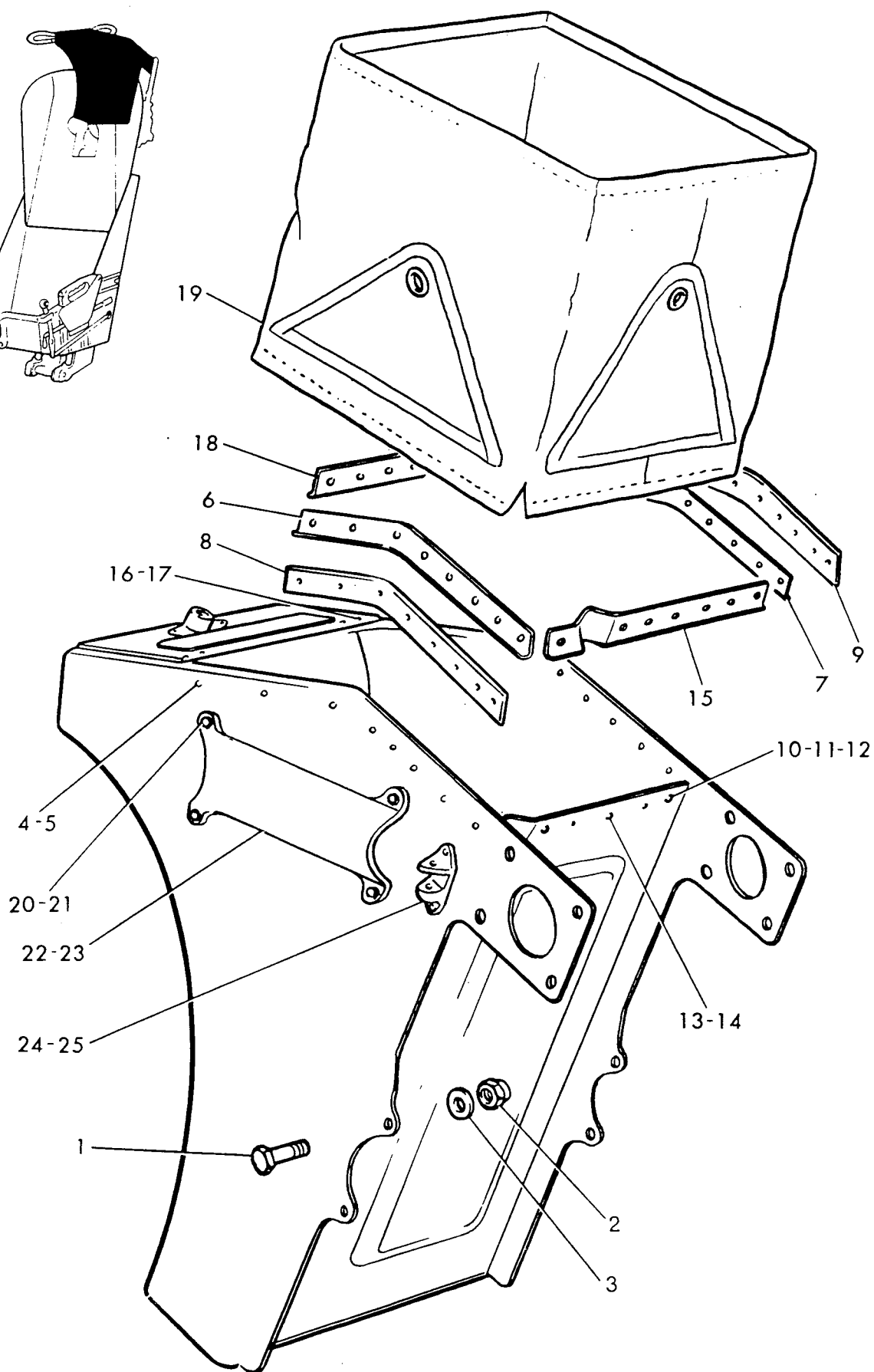
Fig 12 Drogue Container Assembly
