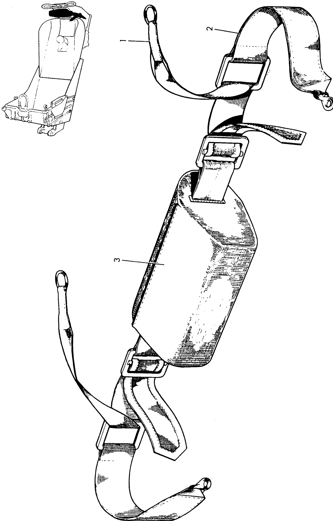
Fig 24 Wedge Pad Assembly
