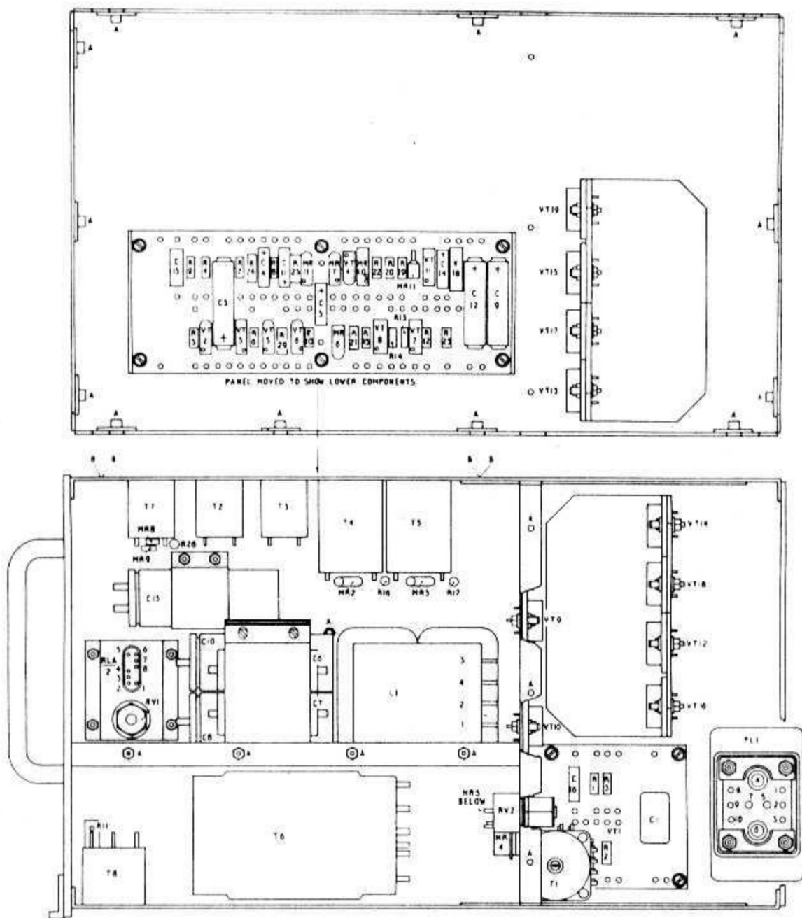
Fig. 2. Inverter, Type E182, Component layout
