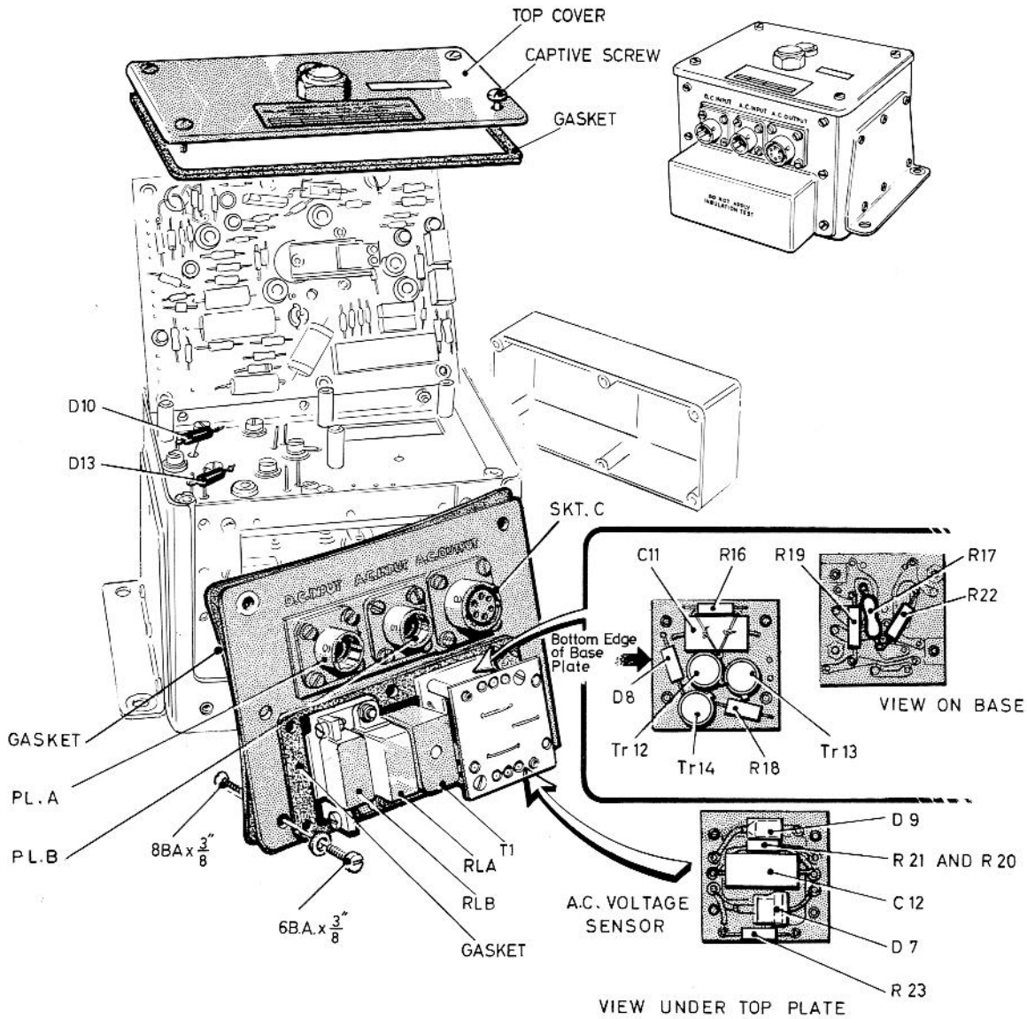
Fig 1 Front panel and general view
