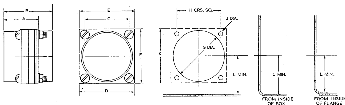
Fig. 23. Panel piercing details, bulkhead unit
