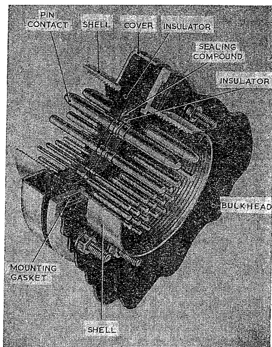
Fig. 11. Pressurised bulkhead unit
