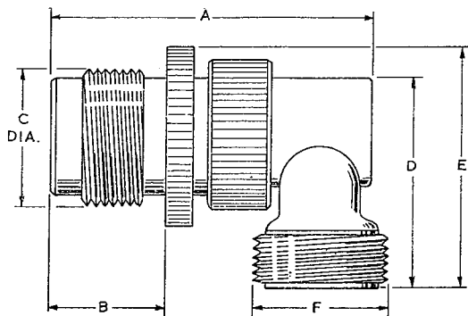
Fig. 29. Dimensions short reach free unit
