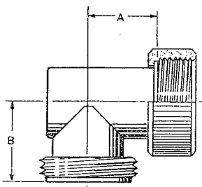
Fig. 40. Elbow assembly
