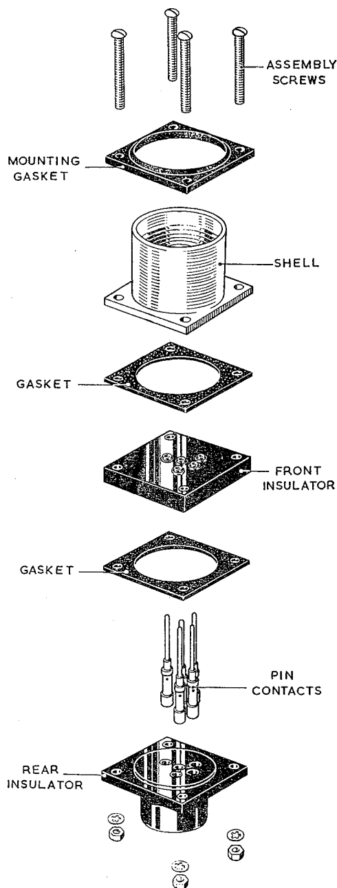
Fig. 4. Fixed unit (exploded)—climatic-proof
