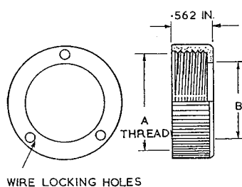
Fig. 32. Coupling unit
