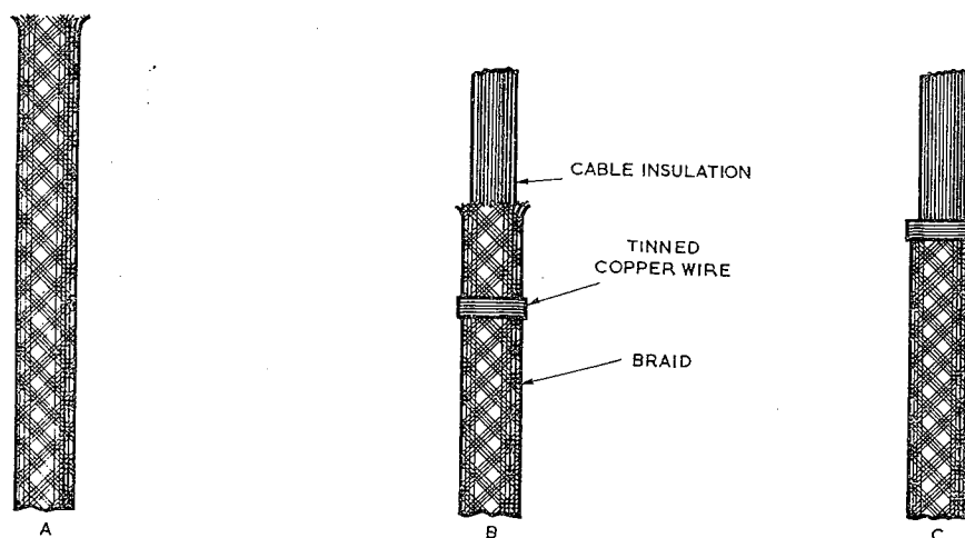
Fig. 18. Preparation of ends of screened cable
