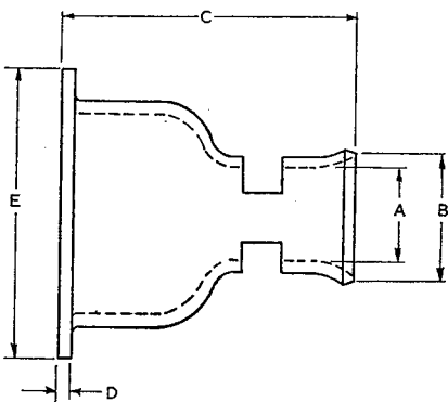
Fig. 43. Cut ferrule square base
