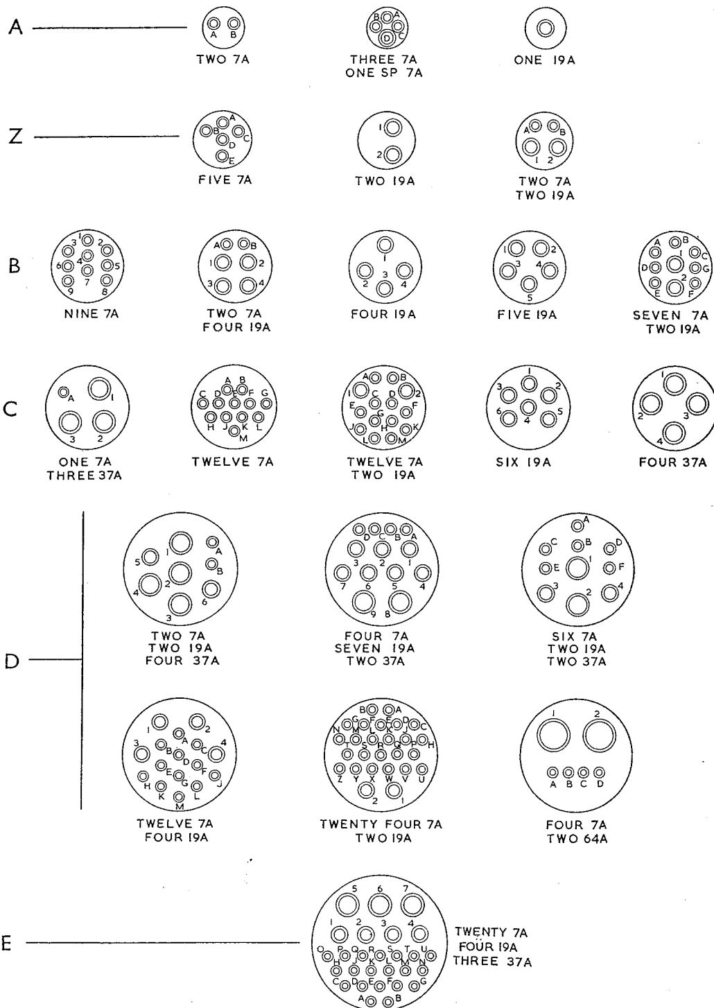
Fig. 20. Contact arrangements
