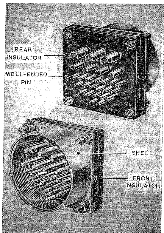
Fig. 2. Fixed unit—loose pins version
