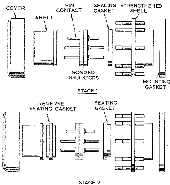
Fig. 12. Pressurised bulkhead unit, stages of development
