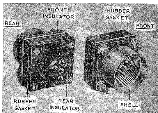
Fig. 3. Fixed unit—climatic-proof
