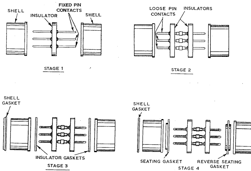
Fig. 10. Bulkhead unit, stages of development
