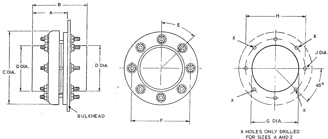
Fig. 24. Panel piercing details, pressurized unit
