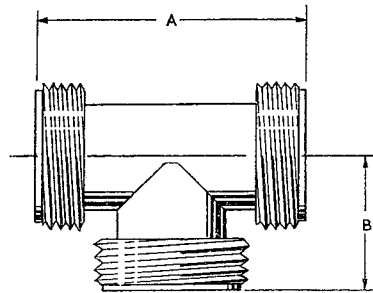
Fig. 41. Tee connector
