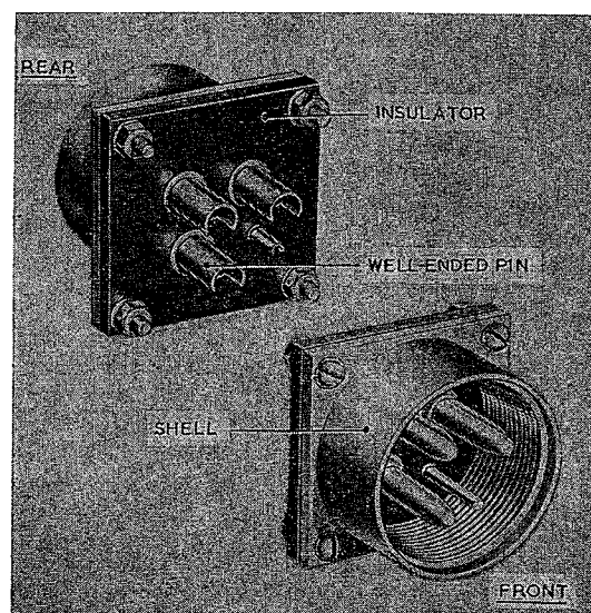
Fig. 1. Fixed unit—fixed pins version
