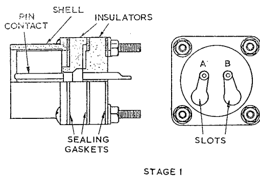
Fig. 13. Fixed unit (detachable leads), stages of development
