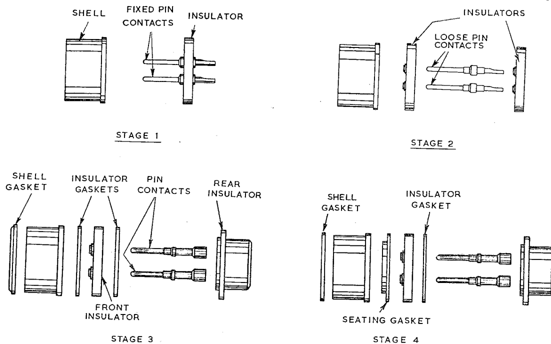
Fig. 5. Fixed unit, stages of development
