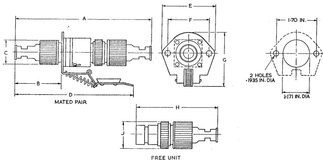
Fig. 26. Panel piercing details, quick release unit
