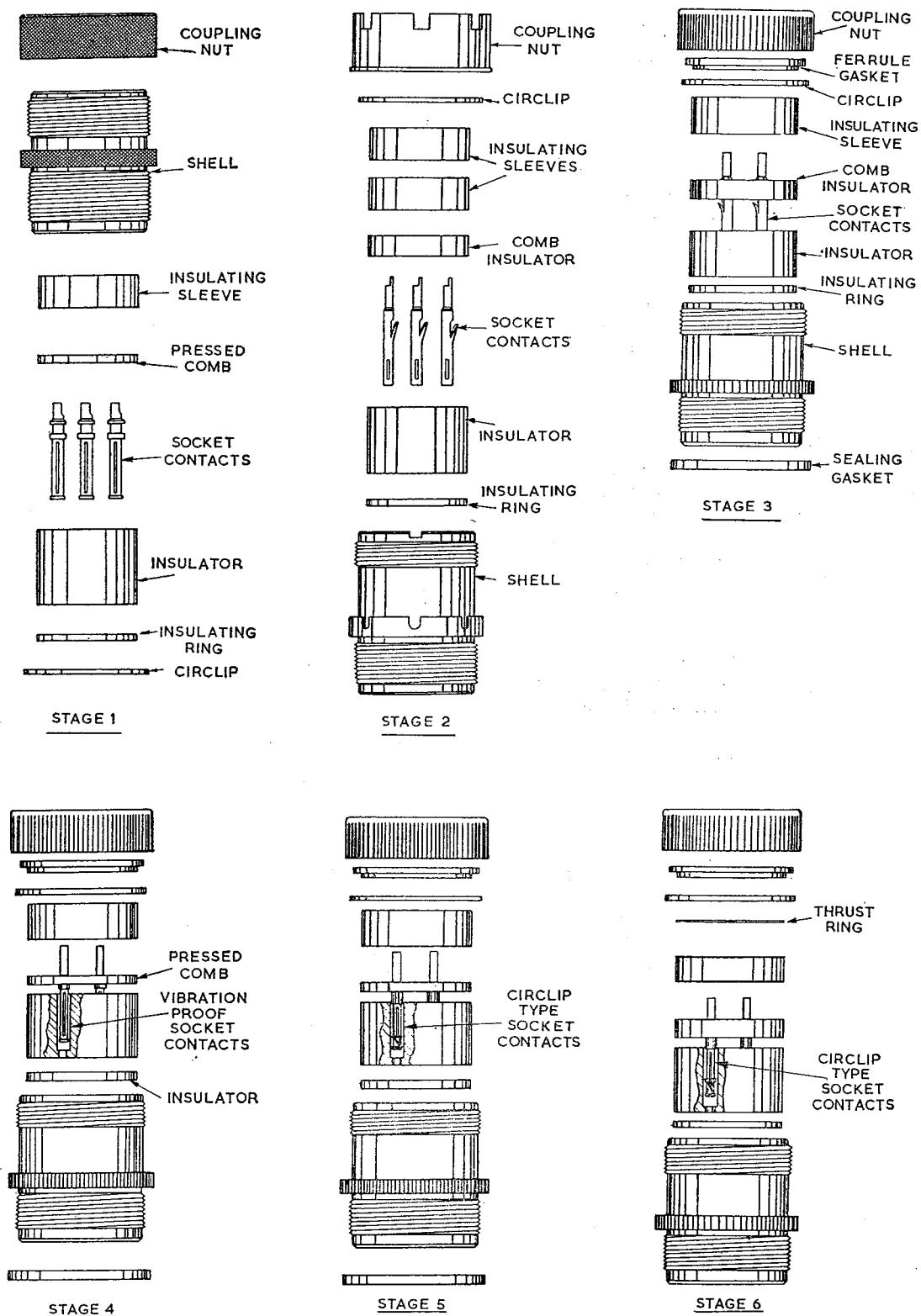
Fig. 8. Free unit, stages of development
