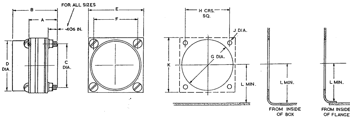
Fig. 22. Panel piercing details, fixed unit
