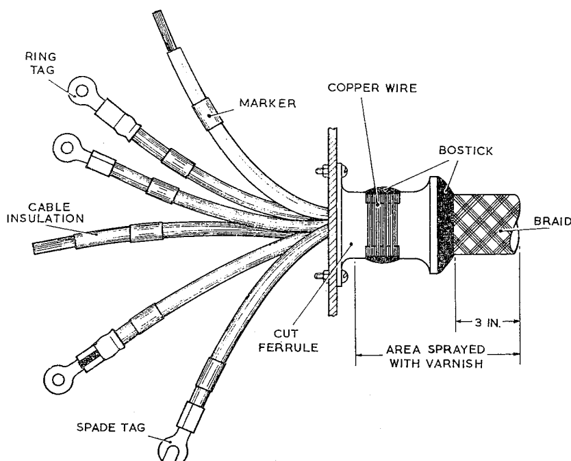
Fig. 17. Cut ferrule used with screened cable
