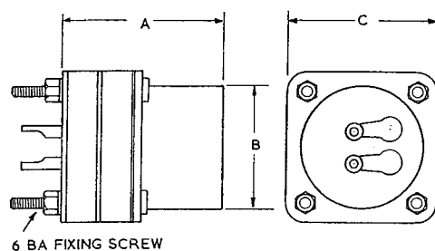
Fig. 27. Dimensions fixed unit detachable leads
