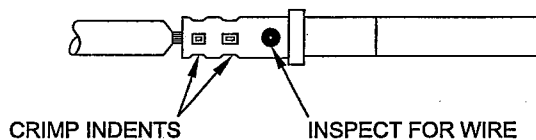
Fig 3 Inspection of contact after crimp
