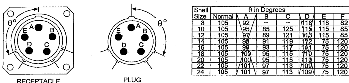
Fig 3 Keyway orientations
