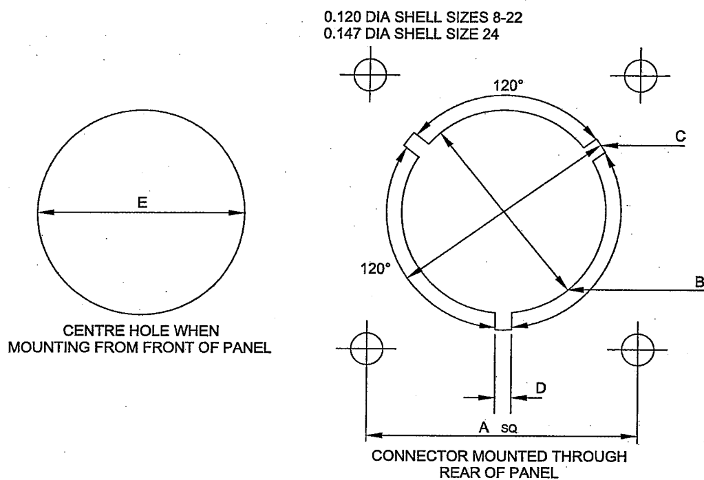
Fig 10 460 Square flange receptacle, panel cut-out dimensions
