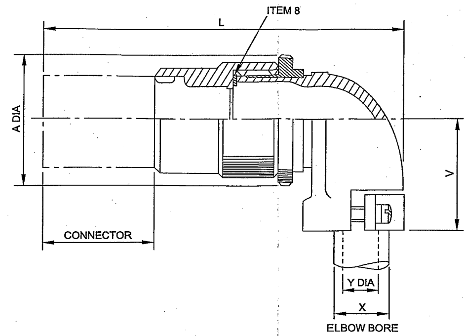
Fig 37 90 degree outlet clamp, dimensions
