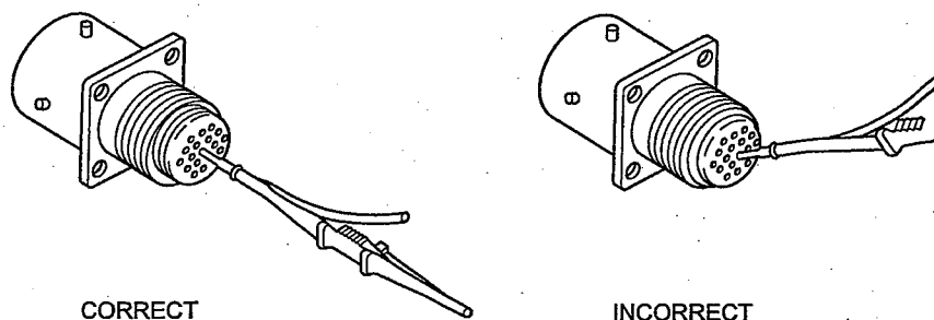
Fig 5 Contact insertion into rear insert
