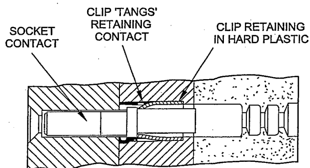
Fig 4 Contact retention
