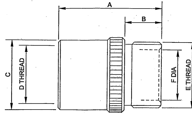
Fig 39 MS3057 Cable clamp adapter, dimensions
