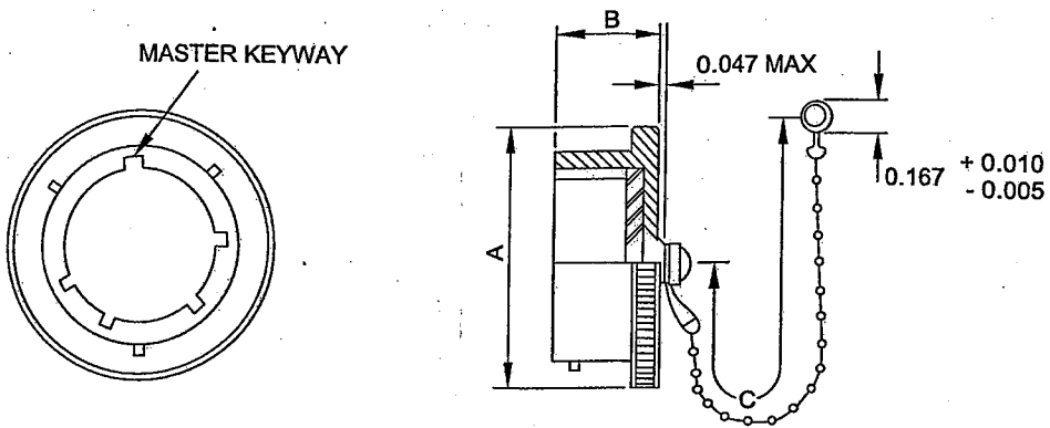
Fig 32 MS3180 Type C plug protective cap, dimensions
