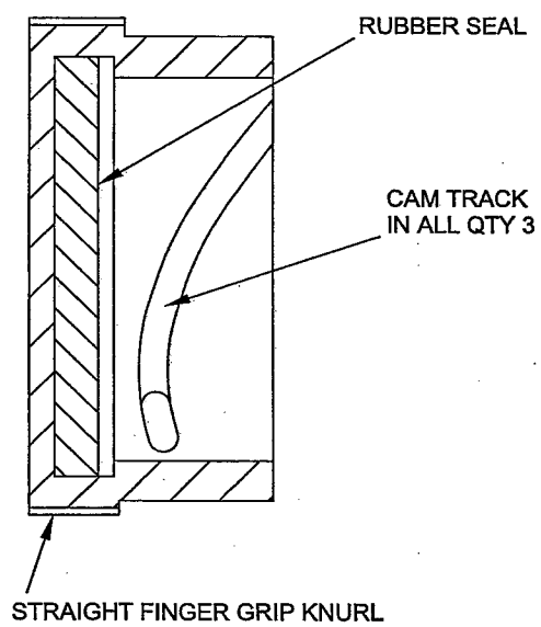
Fig 30 Receptacle plastic protective cap, sectional view
