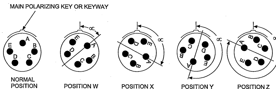
Fig 2 Insert orientations
