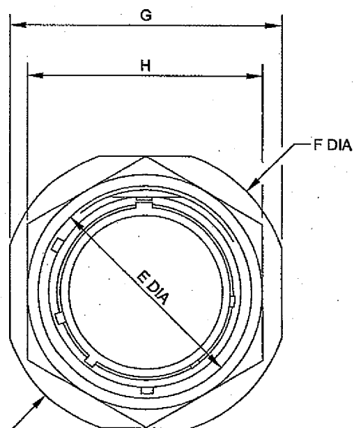
Fig 26 467HTB through bulkhead
