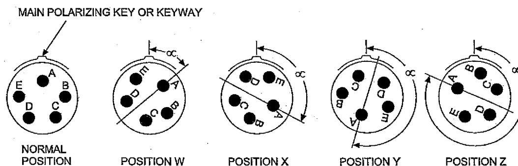
Fig 2 Insert orientations
