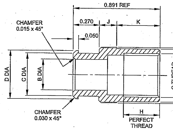
Fig 40 Sleeving adapter, 460
