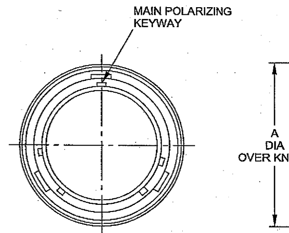
Fig 13 466 Straight plug
