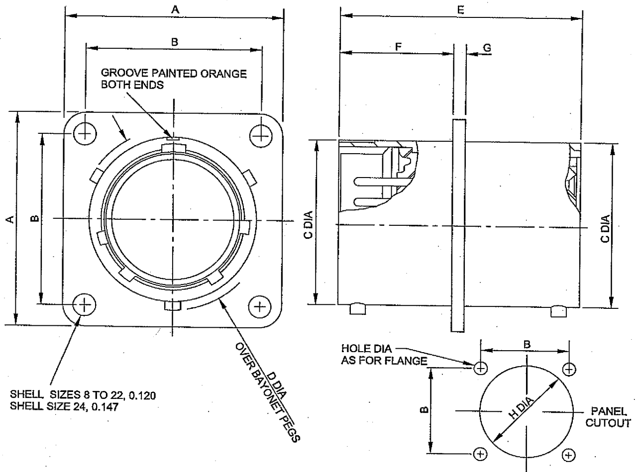
Fig 25 460HTB through bulkhead receptacle, dimensions
