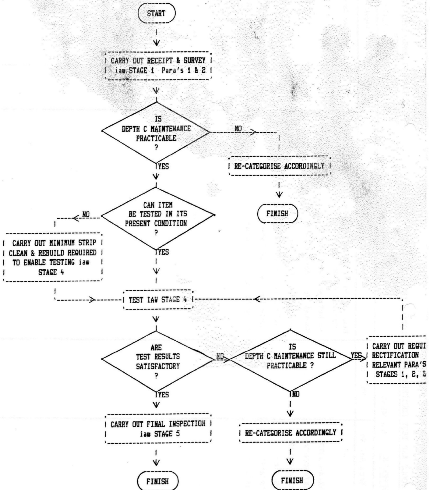
Fig 1. OVERALL MAINTENANCE FLOWCHART
