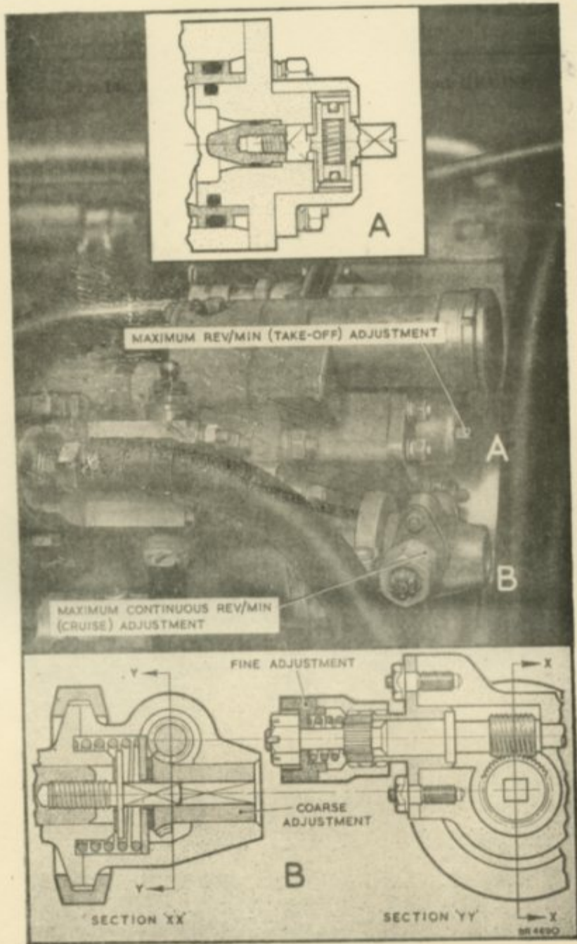
Fig. 14. Maximum rev/min. TAKE-OFF and CRUISE adjustments
