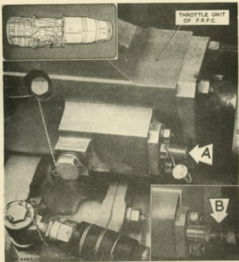
Fig. 15. Idling by-pass adjustment
