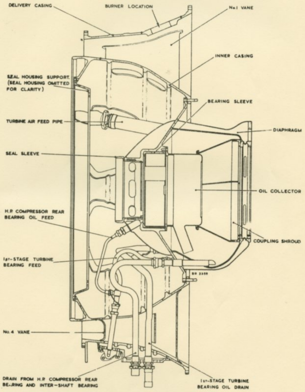
Delivery casing details
