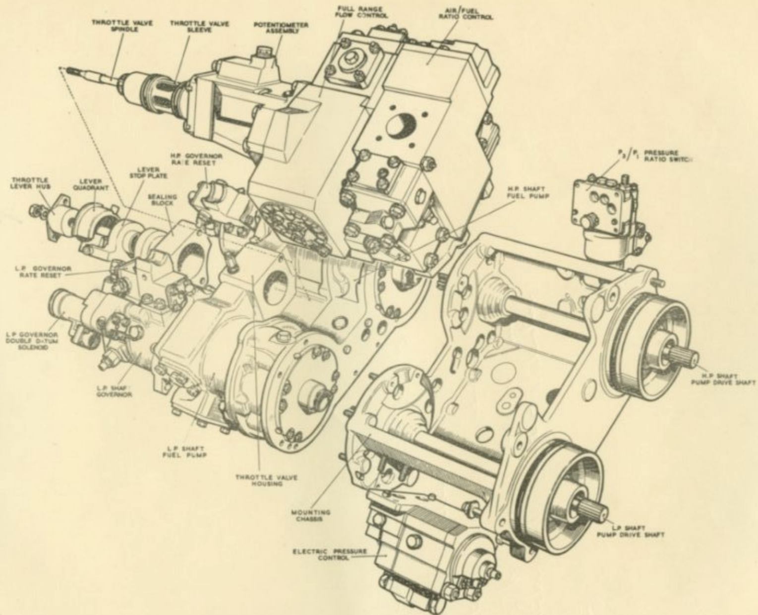
EXPLODED VIEW OF MAIN UNITS CHASSIS MOUNTED FUEL SYSTEM. TYPE C.M.F.S.
