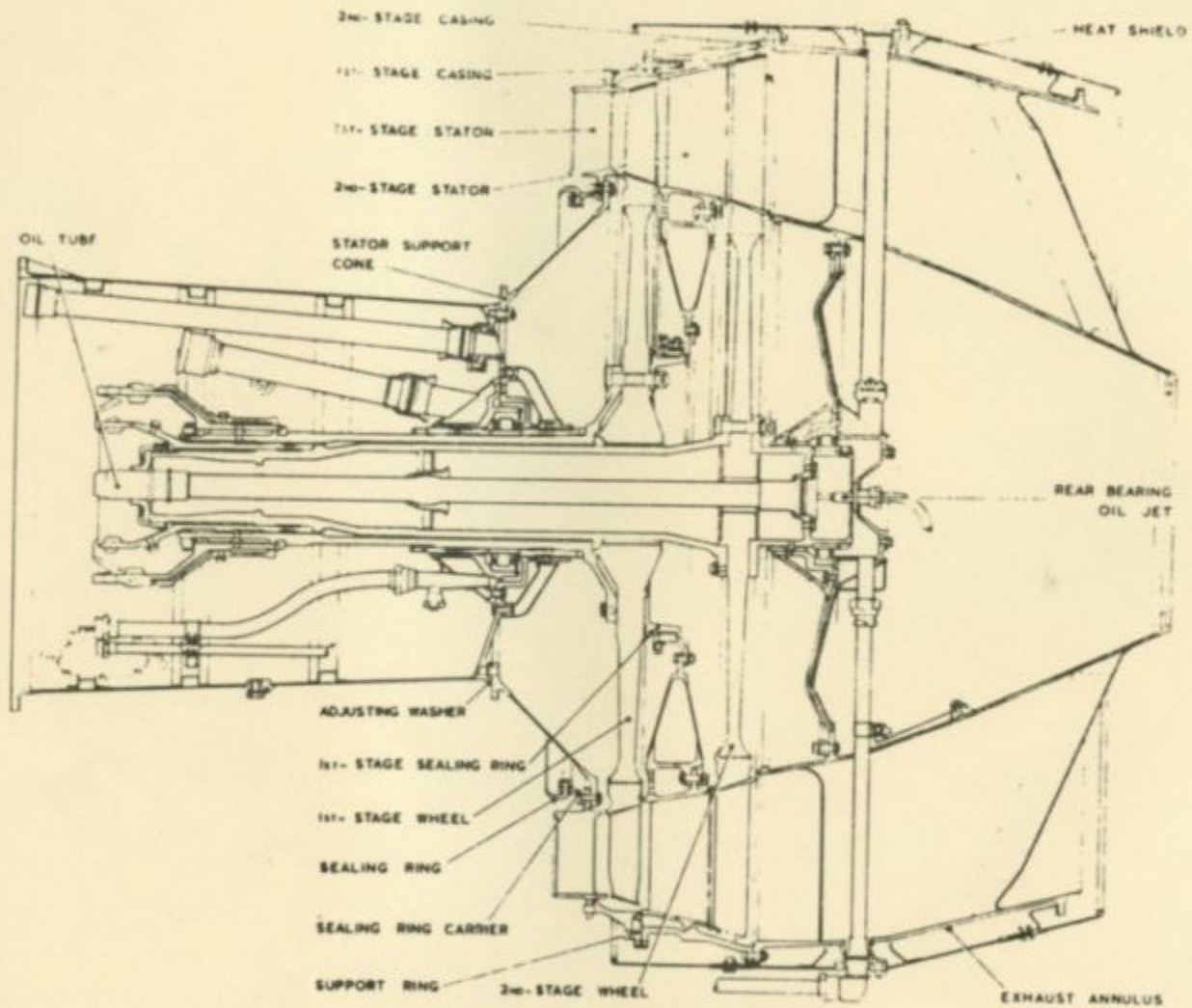
Turbine—general arrangement
