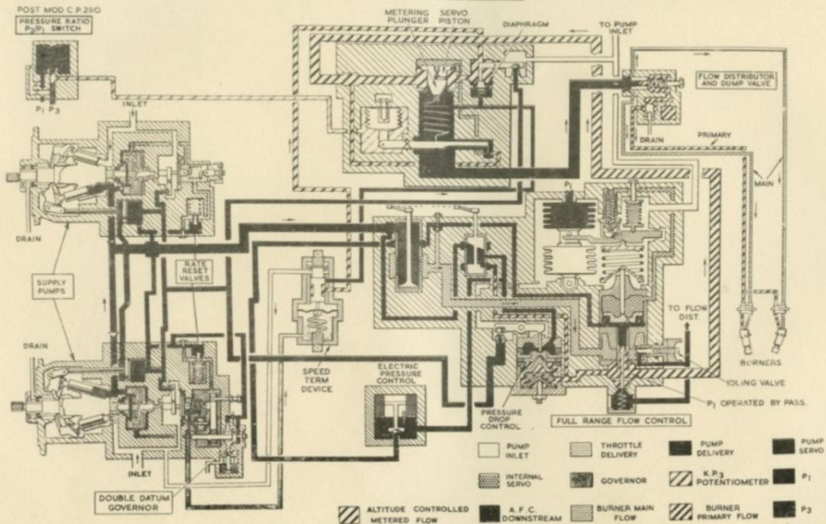
FIG. 3 FUNCTIONAL DIAGRAM
