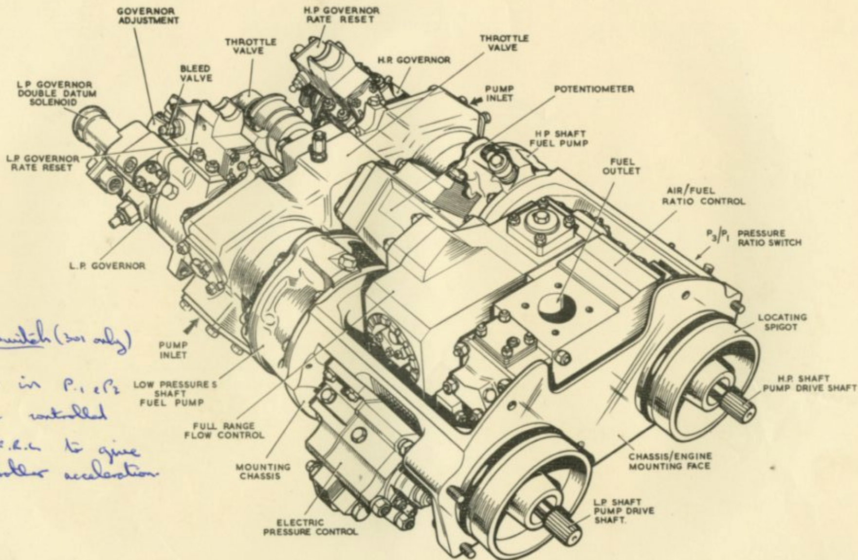
CHASSIS MOUNTED FUEL SYSTEM, TYPE C.M.F.S.
