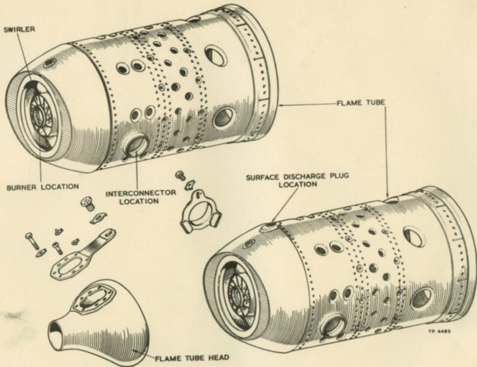
COMBUSTION CHAMBER
