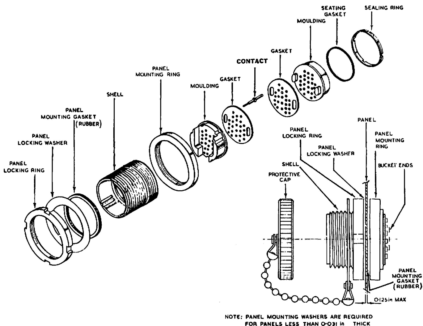
Fig 7 - Exploded and assembled views of a panel mounted component
