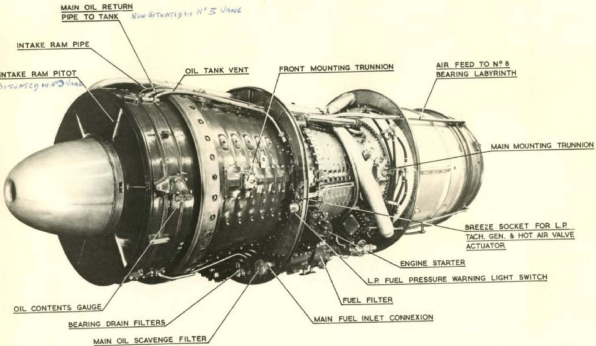
OLYMPUS 101 ENGINE
