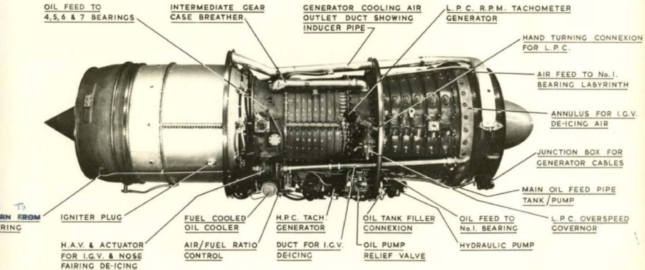
OLYMPUS 101 ENGINE
