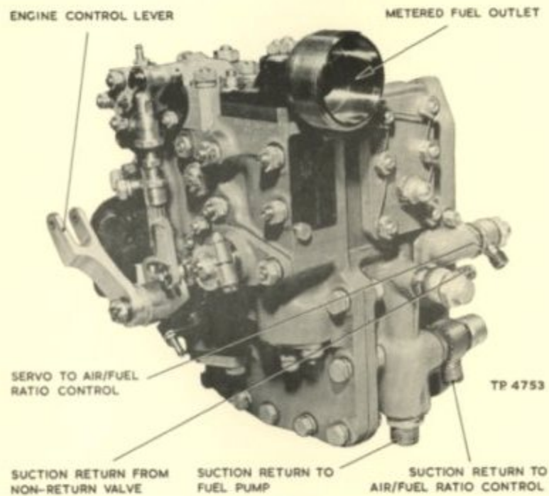
FULL RANGE FLOW CONTROL.
