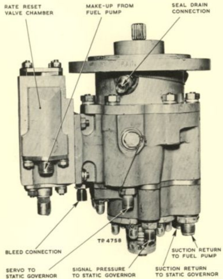
L.P. COMPRESSOR DRIVEN GOVERNOR.
