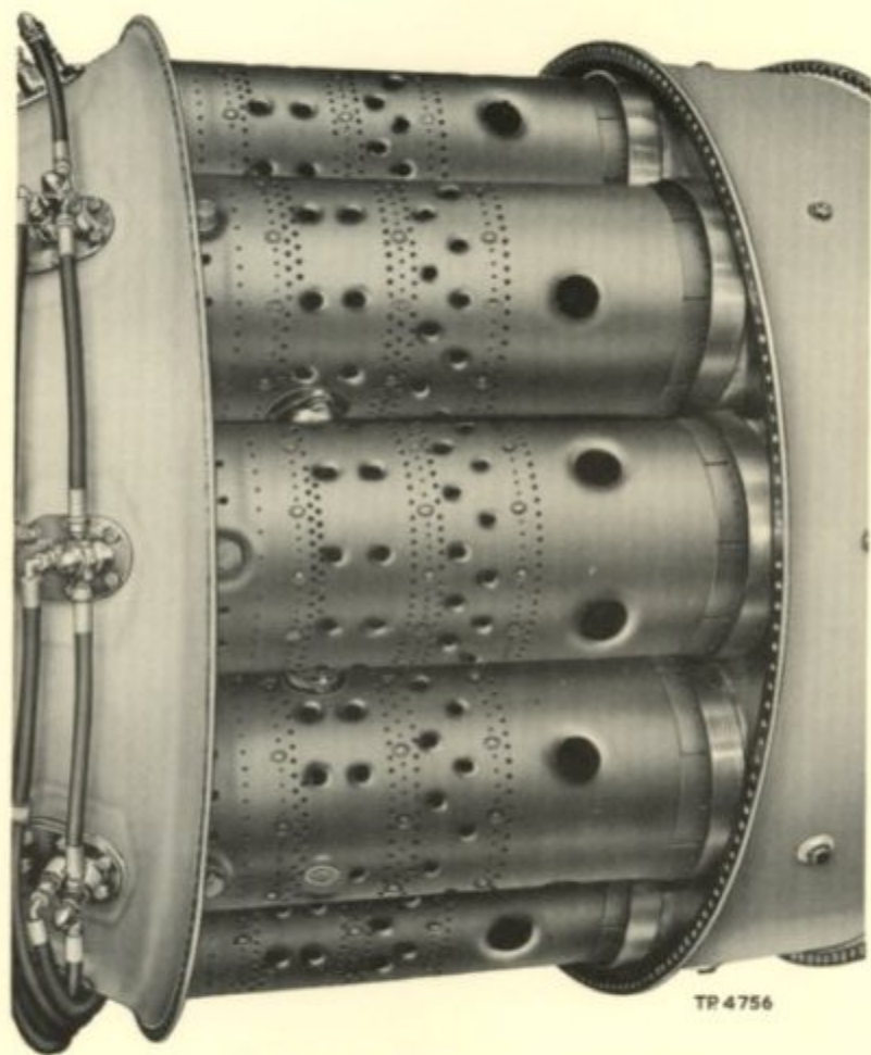
FLAME TUBES IN POSITION.
