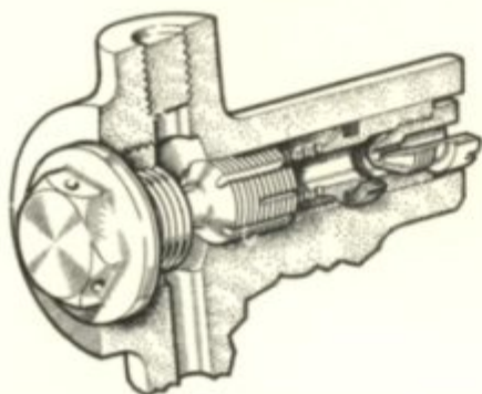
OIL JET FOR L.P. COMPRESSOR REAR BEARING
