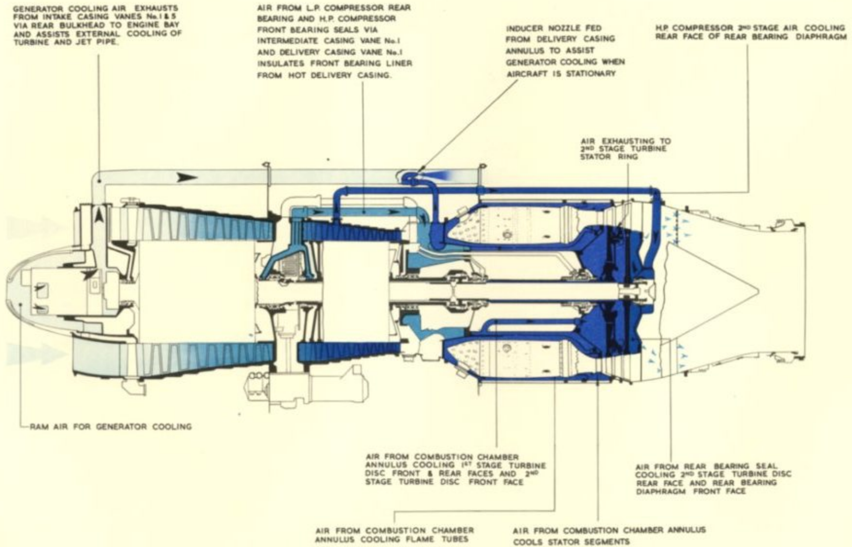
COOLING DIAGRAM - OLYMPUS 104.
