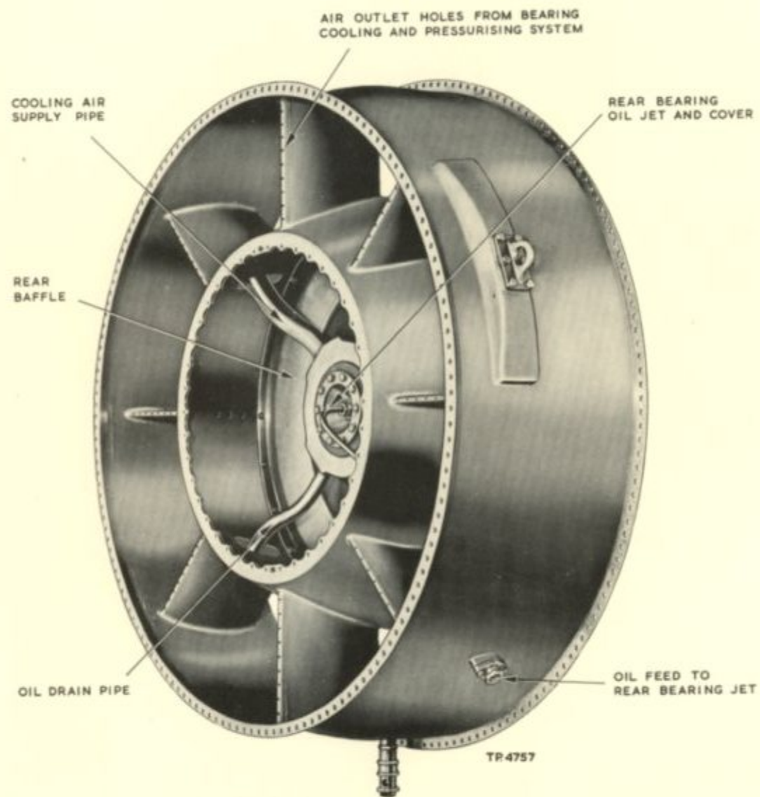
EXHAUST ANNULUS - REAR VIEW.
