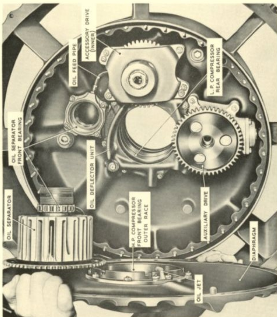
INTERMEDIATE CASING (DIAPHRAGM REMOVED.)
