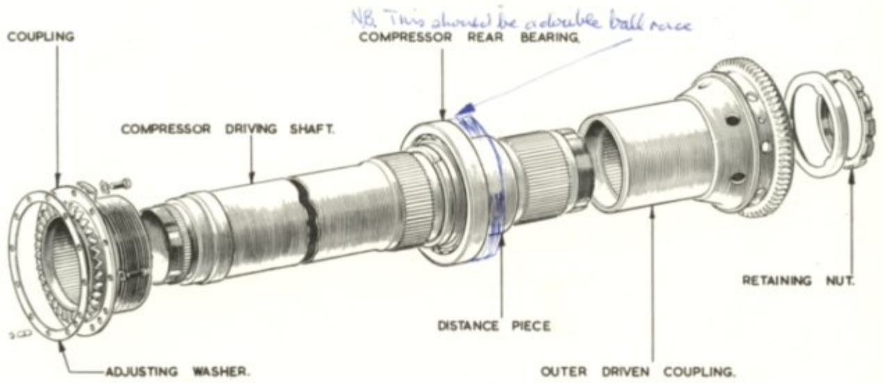
OLYMPUS 101. H.P. COMPRESSOR ROTOR.
