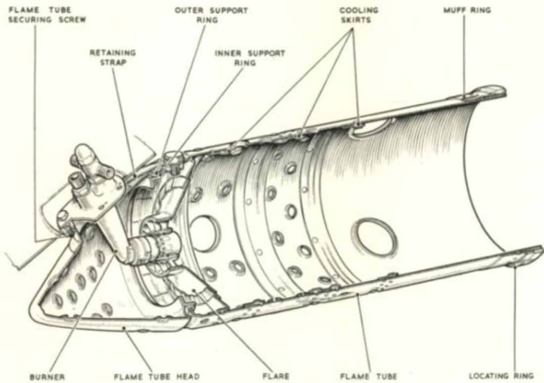
FLAME TUBE.
