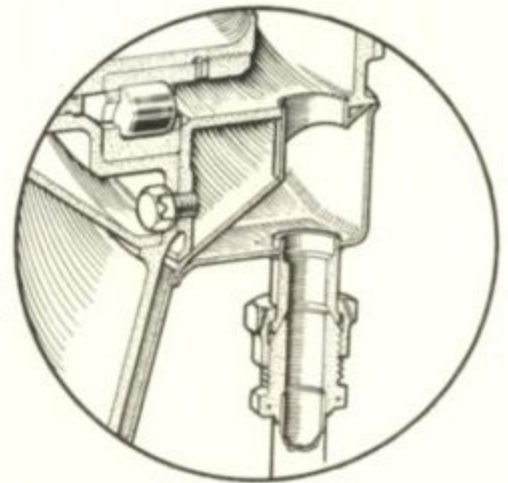
VIEW OF OIL DRAIN LOCATED AT ARROW.
