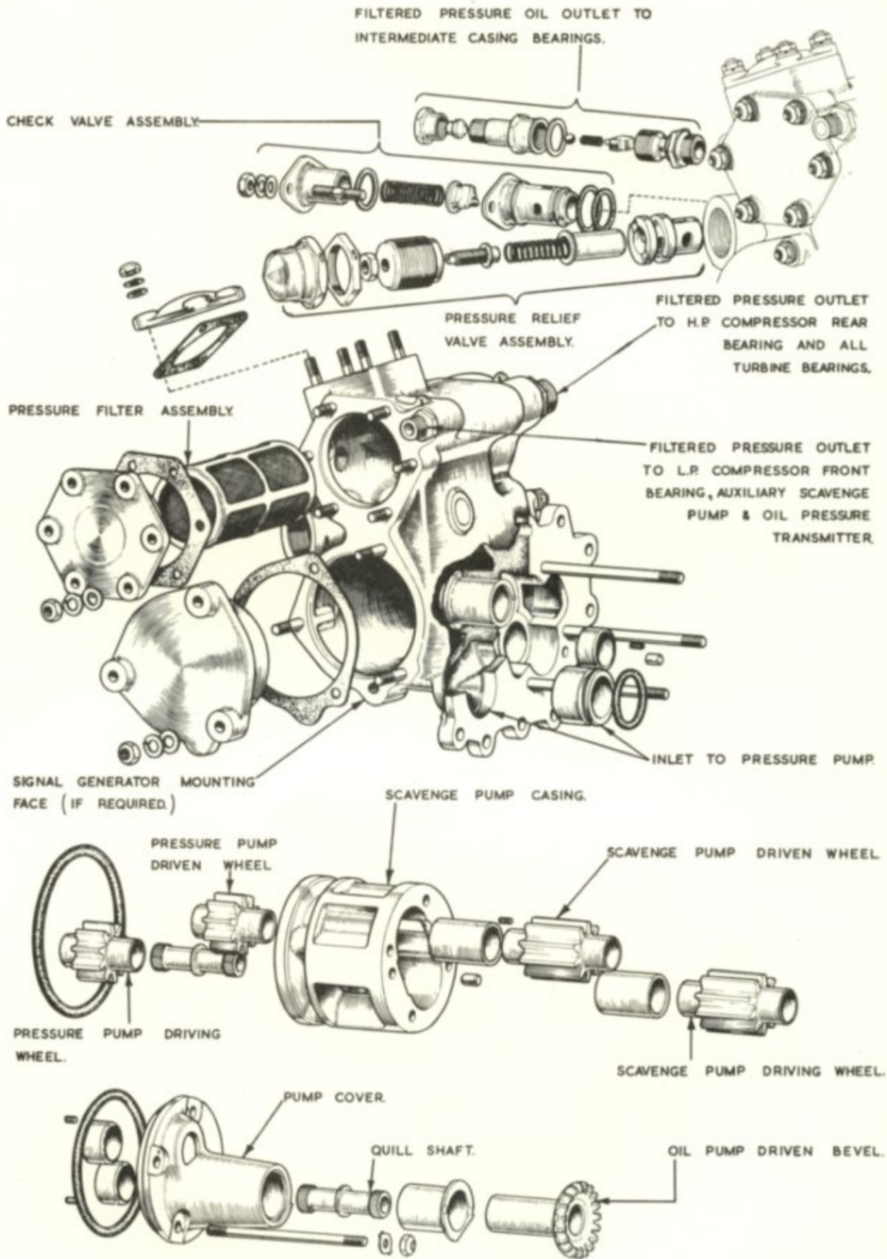
OLYMPUS 101. OIL PUMP & DRIVE HOUSING UNIT.
