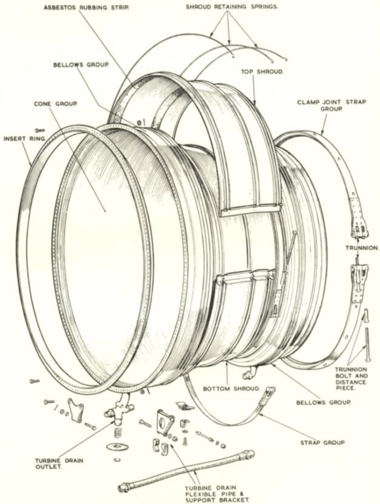
EXHAUST CONE GROUP (OUTER)
