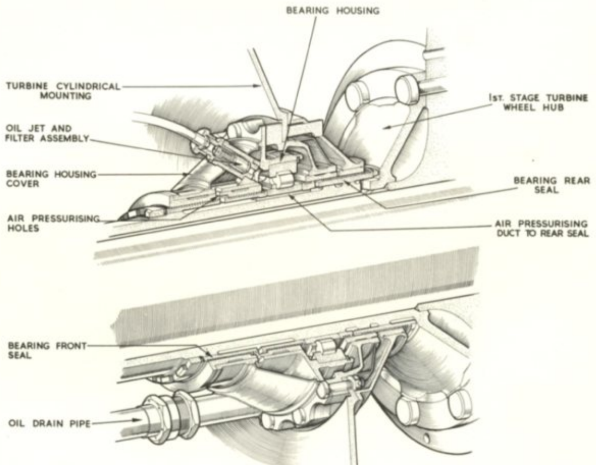
1 ST STAGE TURBINE REAR BEARING HOUSING TP. 3050
