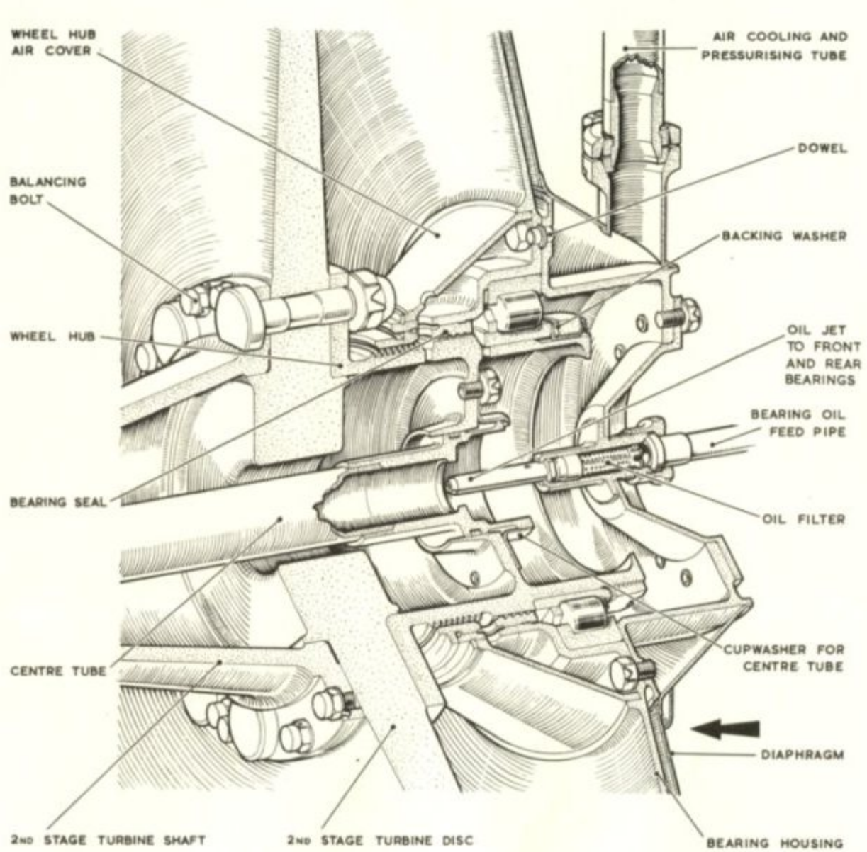
2ND STAGE TURBINE REAR BEARING HOUSING
