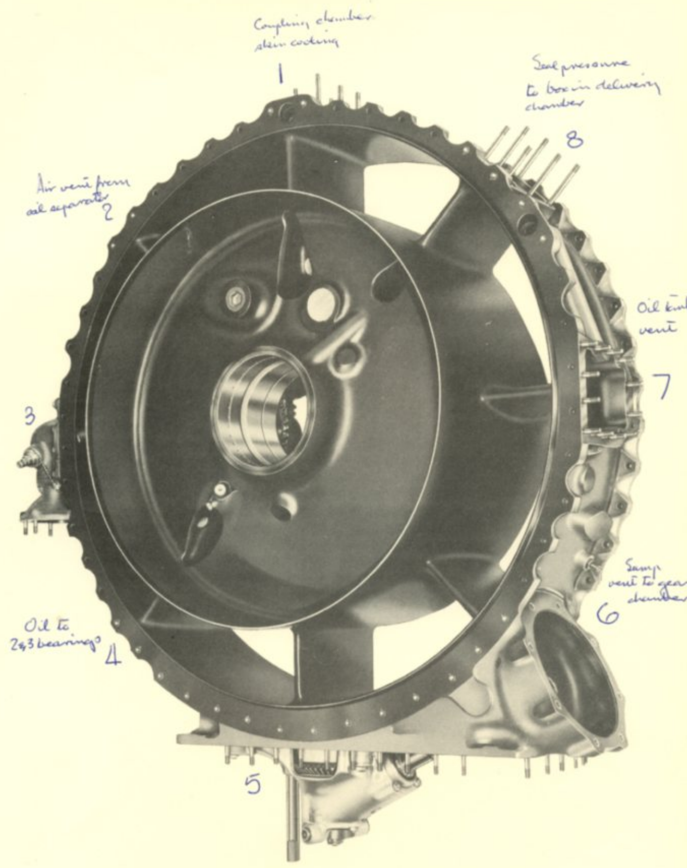
OLYMPUS 10101 E.C.U. INTERMEDIATE CASING 3/4 FRONT.
