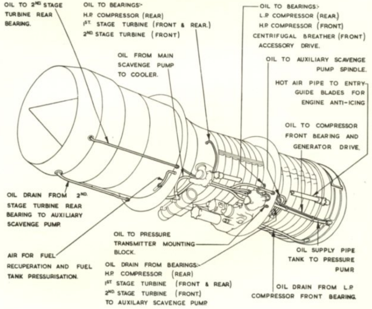
OLYMPUS 101. COOLING AND LUBRICATION SYSTEM.
