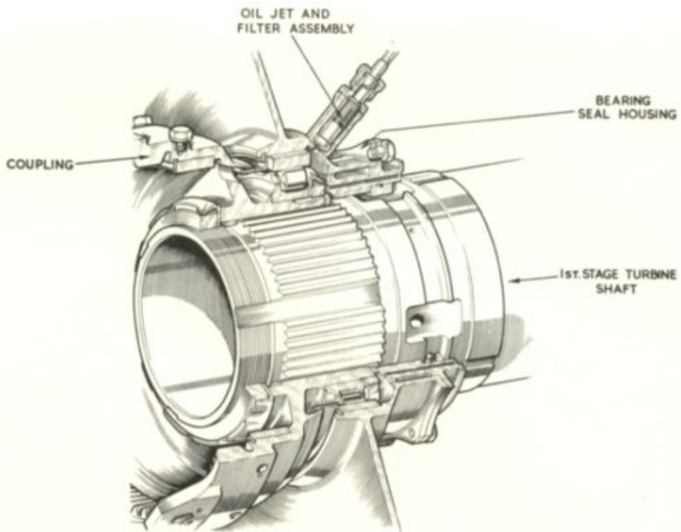
1 ST STAGE TURBINE FRONT BEARING HOUSING
