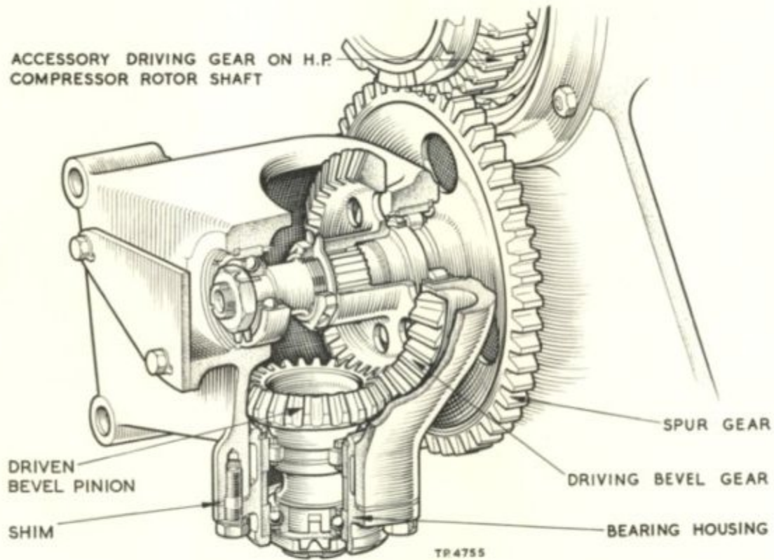
AUXILIARY DRIVE ASSEMBLY.
