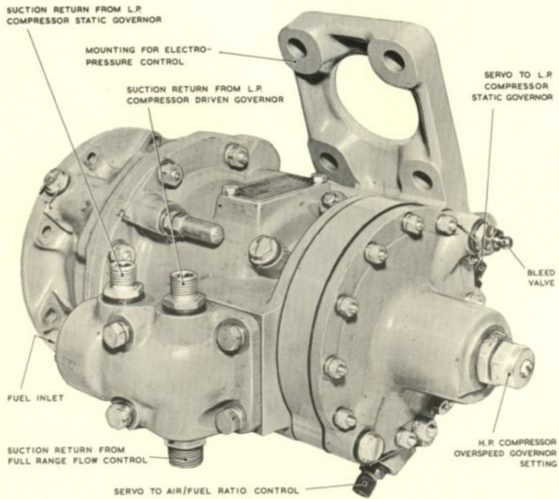
FUEL PUMP
