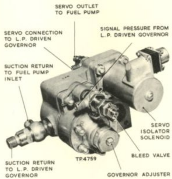
L.P. COMPRESSOR STATIC GOVERNOR.
