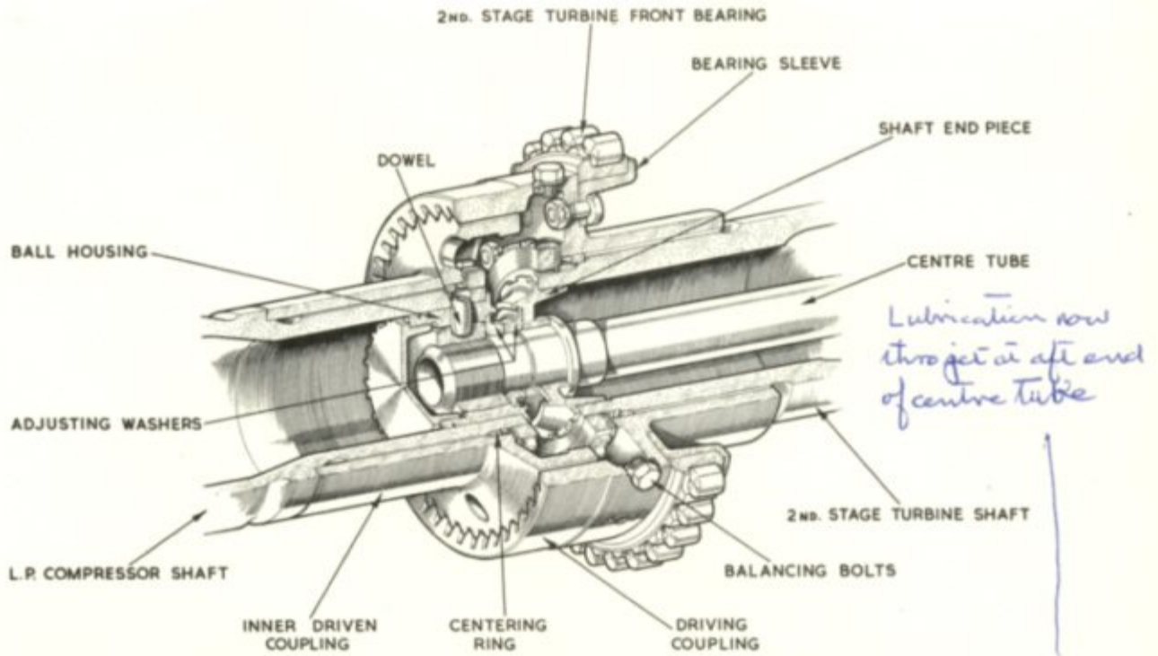
TURBINE INNER COUPLING
