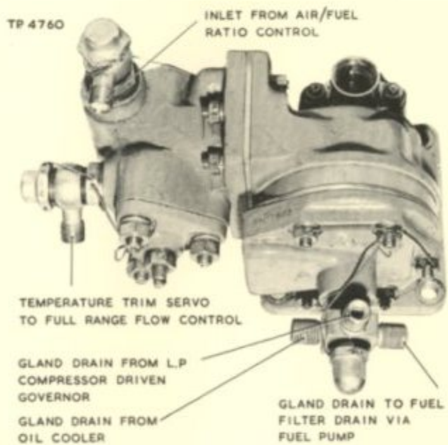
ELECTRO-PRESSURE CONTROL.
