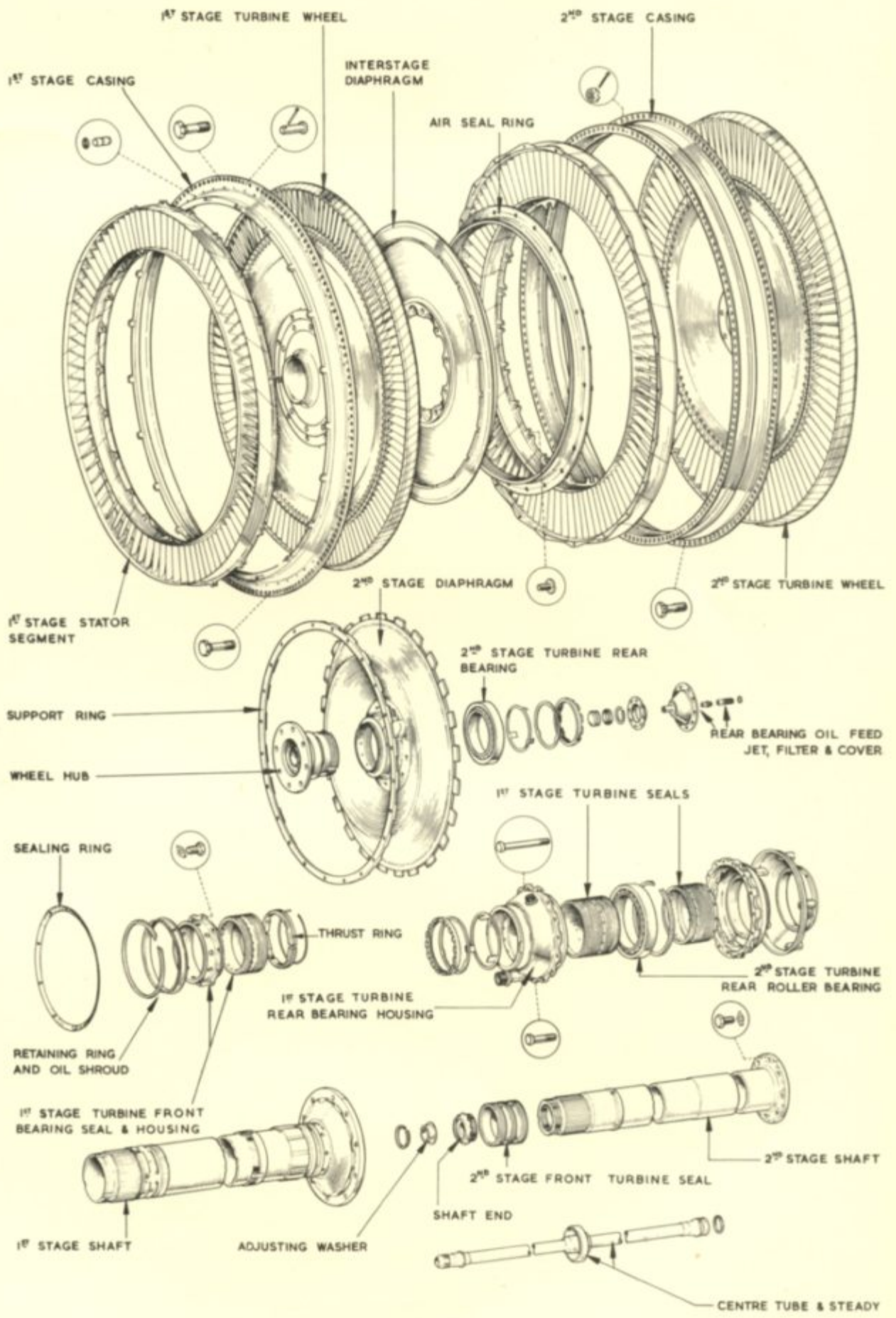
OLYMPUS 101 TURBINE ASSEMBLY (PART I)
