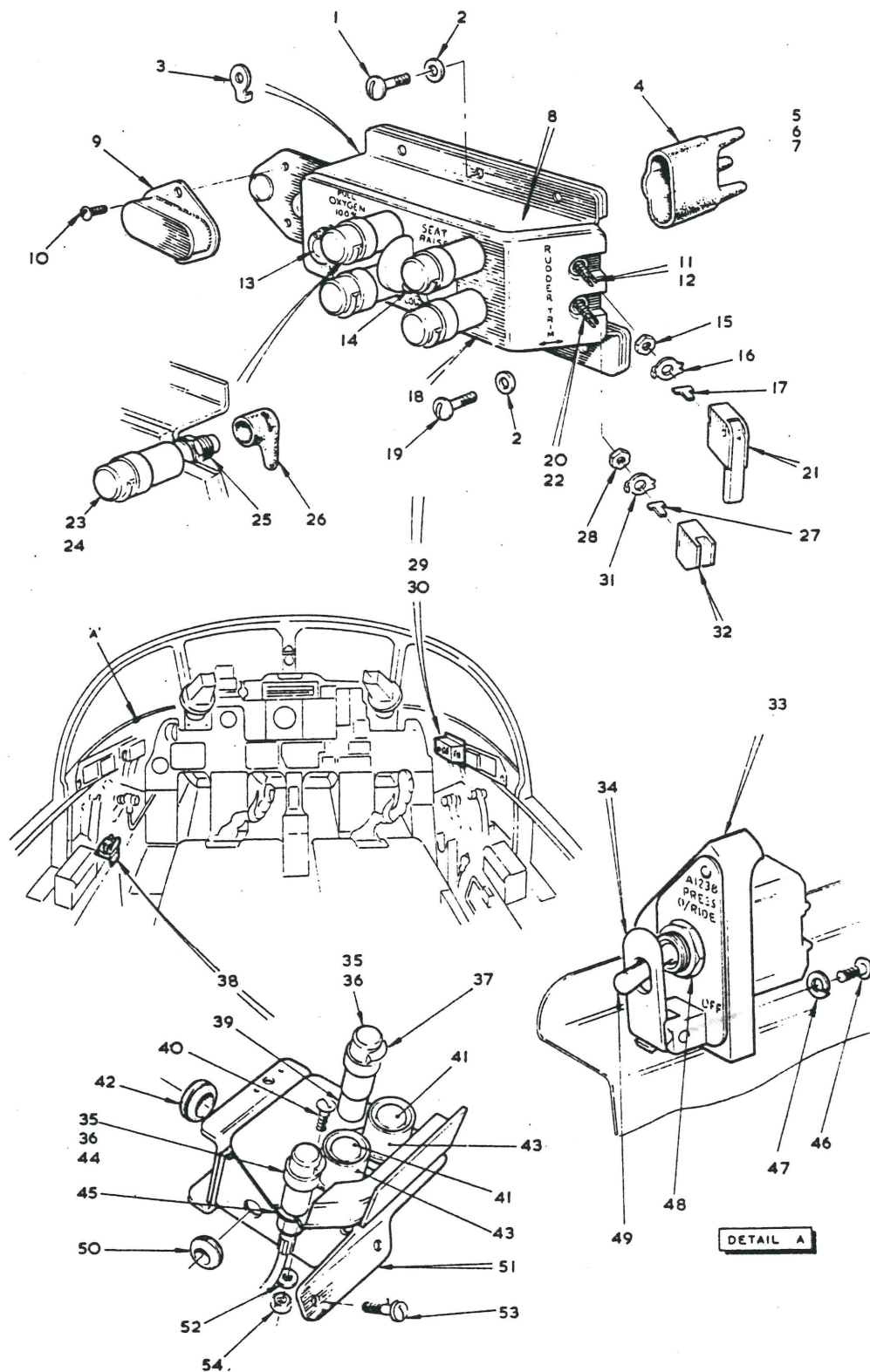
FIG.16 PILOT'S INSTRUMENT. AND CONTROLS Restricted
