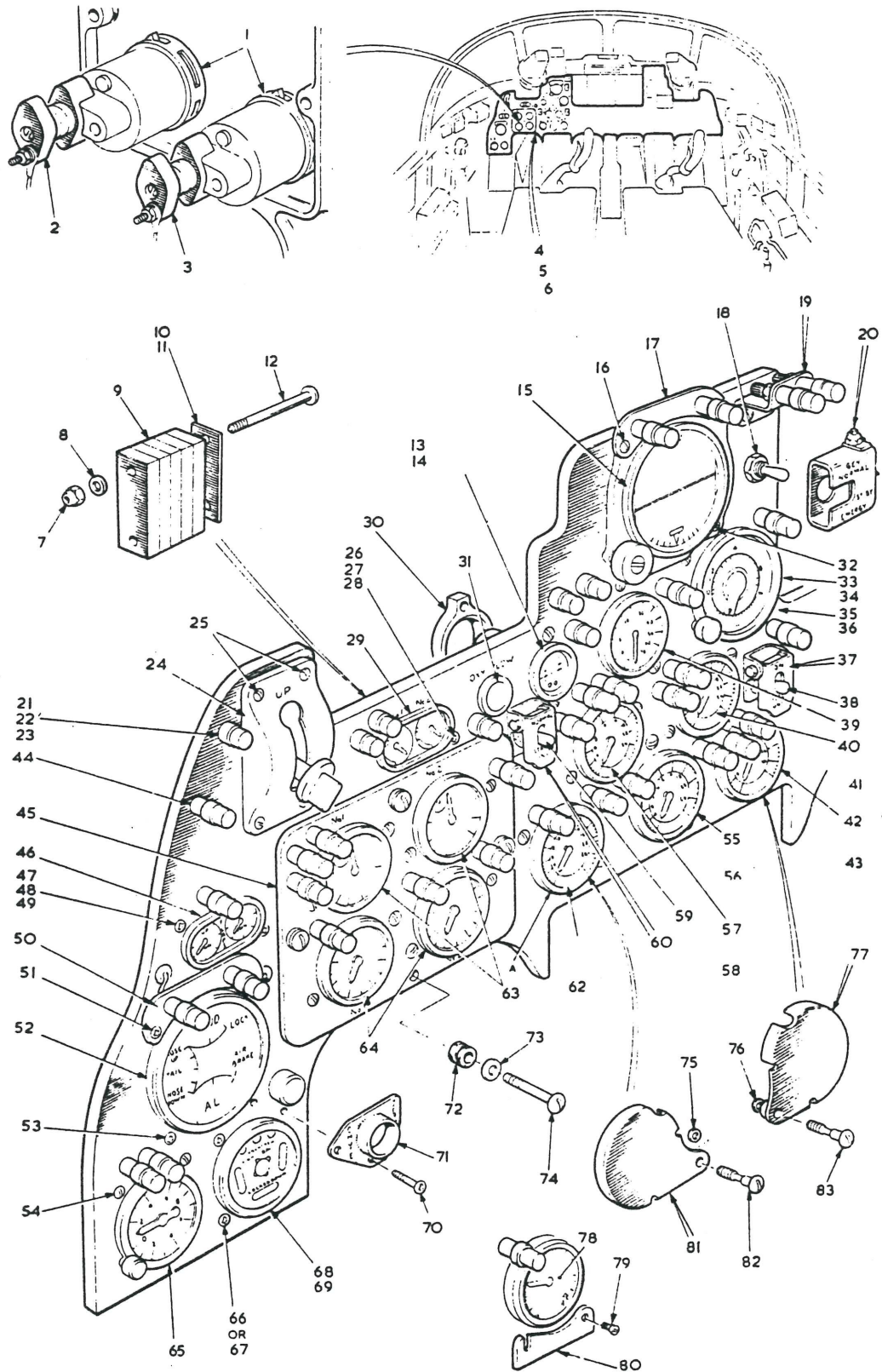
FIG. 7 PILOTS INSTRUMENTS AND CONTROLS Restricted
