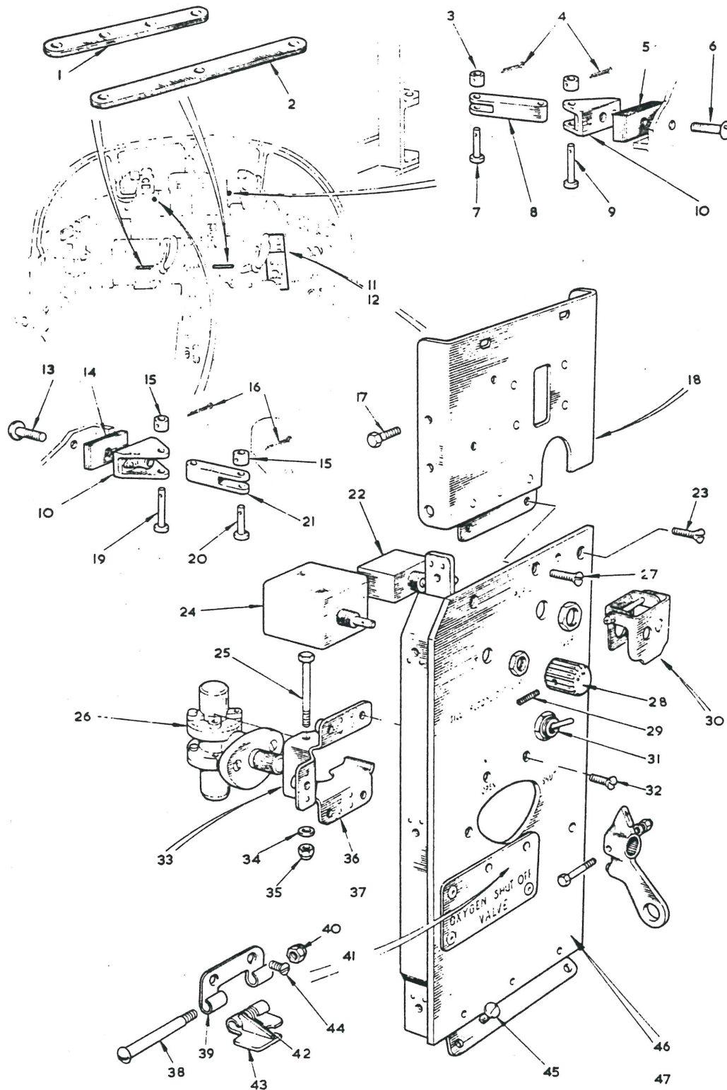
FIG 4. PILOT'S INSTRUMENTS AND CONTROLS Restricted
