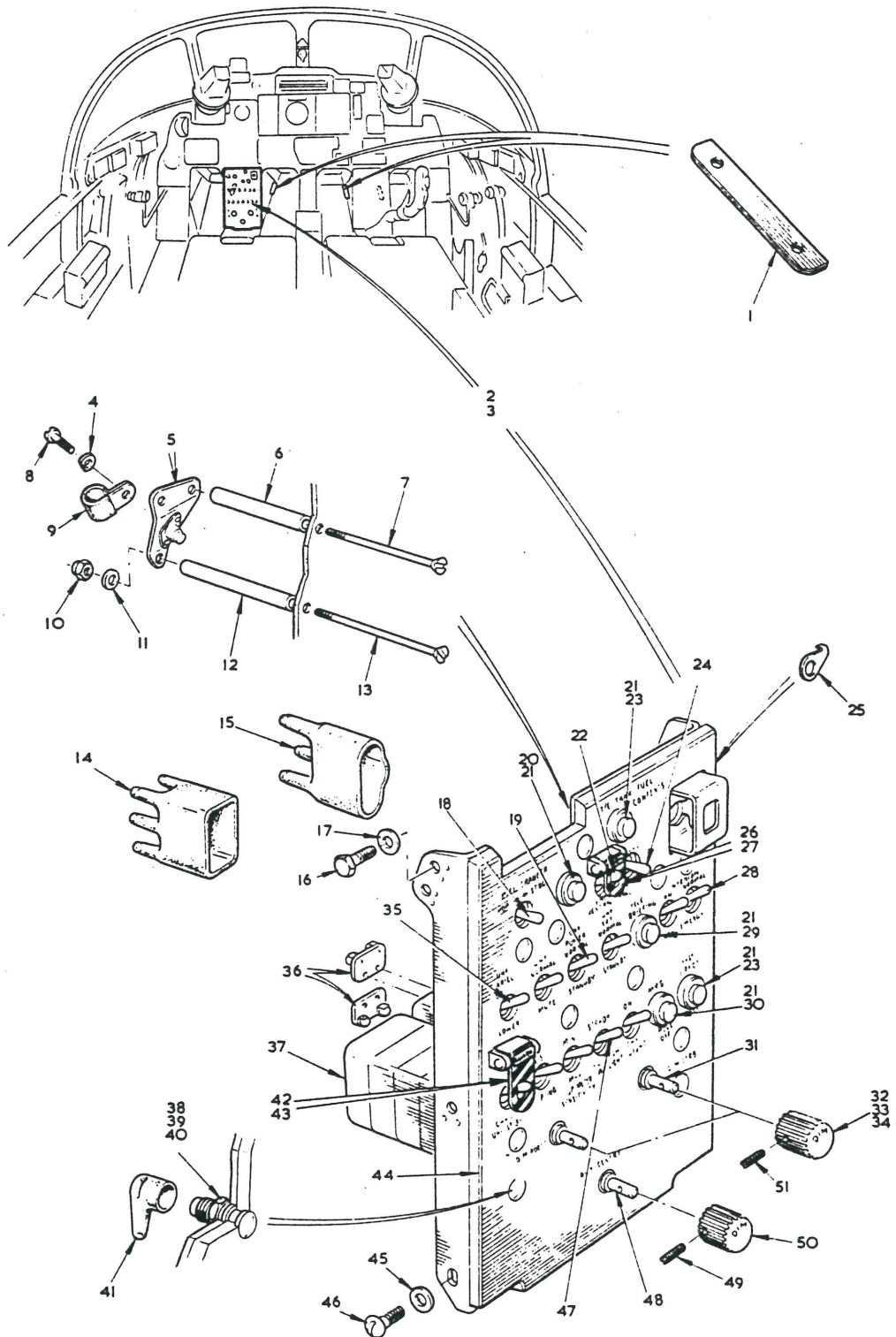
FIG. 11 PILOT'S INSTRUMENTS AND CONTROLS
