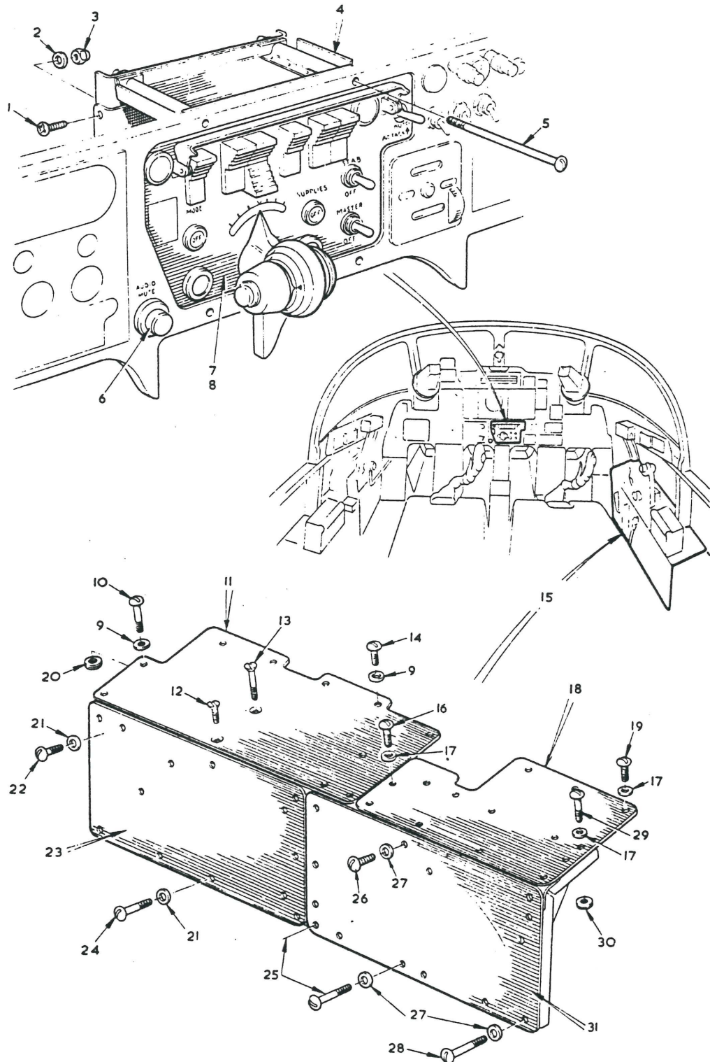
FIG. 6 PILOT'S INSTRUMENTS AND CONTROLS
