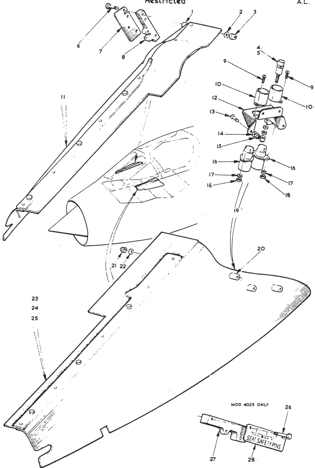
FIG 13 PILOT'S INSTRUMENTS AND CONTROLS Restricted
