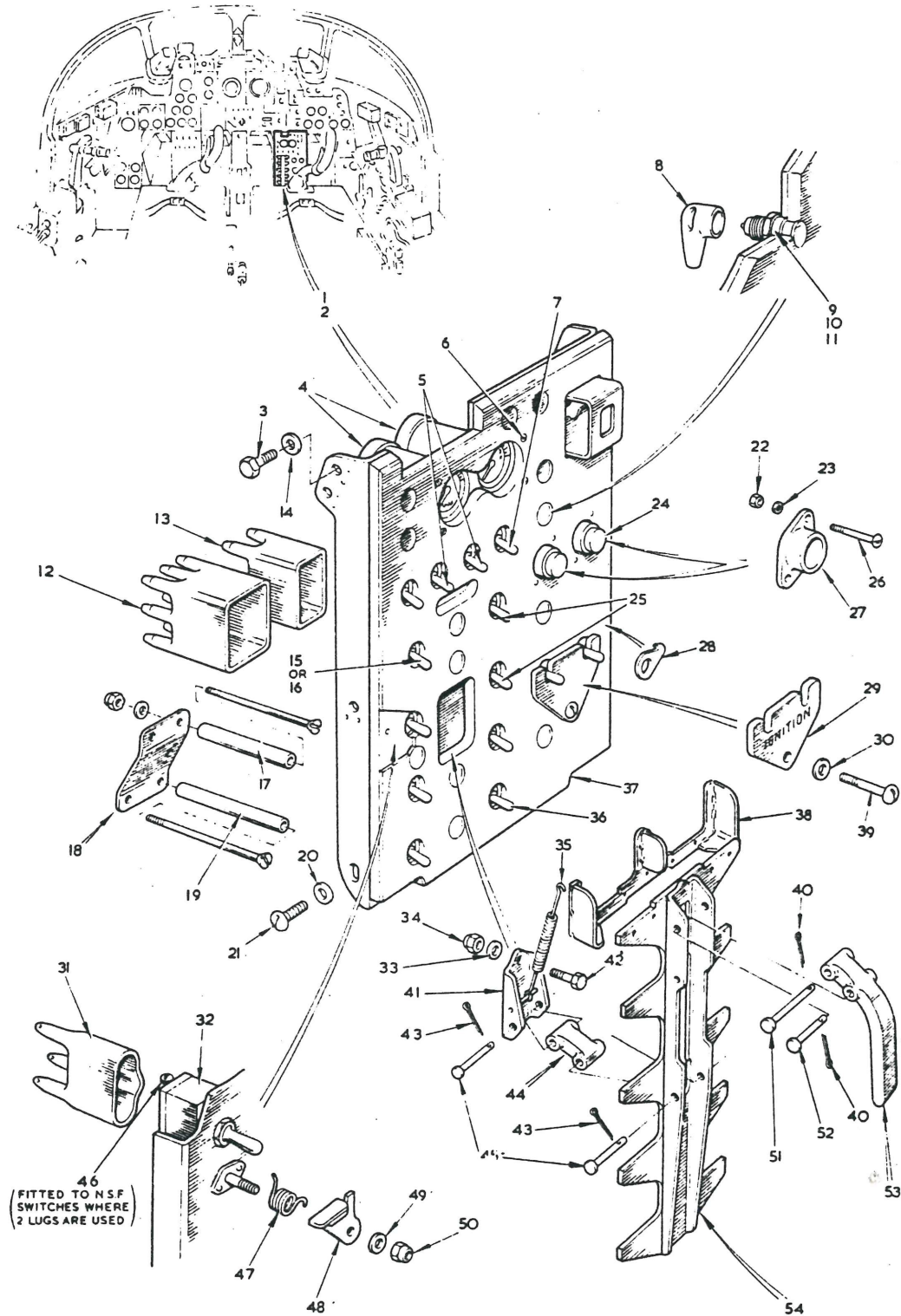
FIG. 3 PILOT'S INSTRUMENTS AND CONTROLS Restricted
