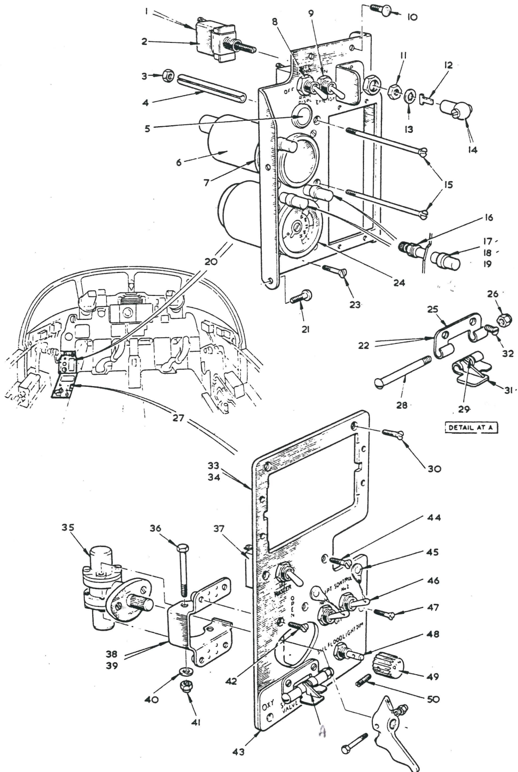
FIG 10. PILOT'S INSTRUMENTS AND CONTROLS Restricted
