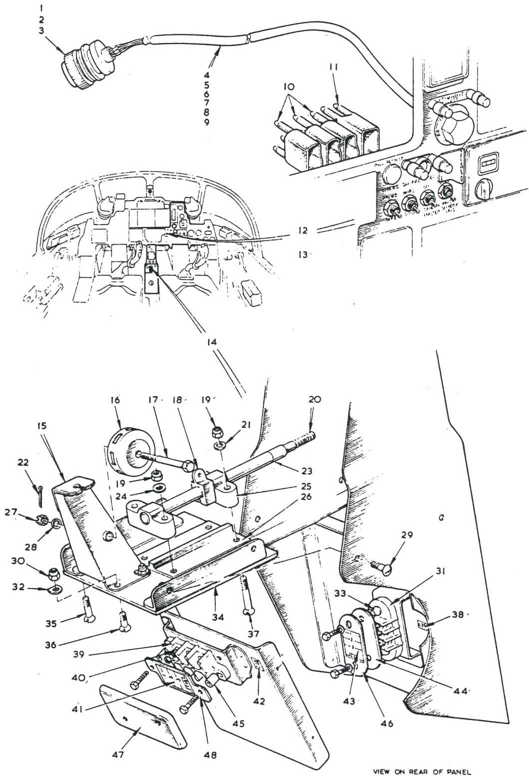
FIG.8 PILOT'S INSTRUMENTS AND CONTROLS Restricted
