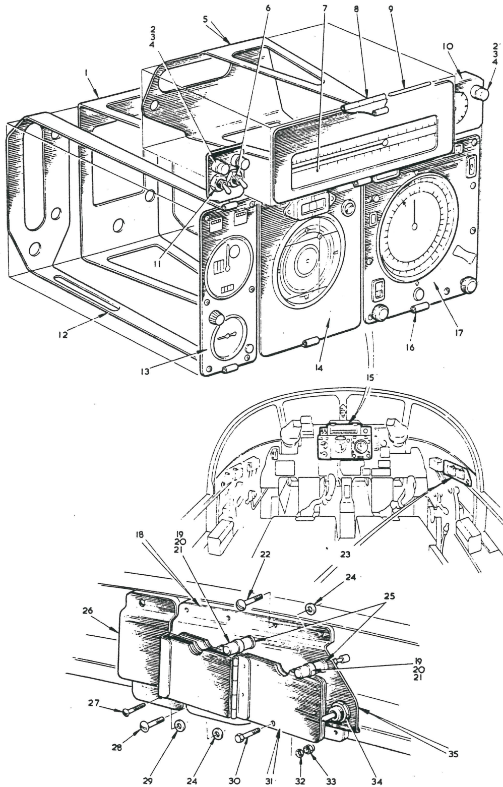
FIG. 2 PILOT'S INSTRUMENTS AND CONTROLS
