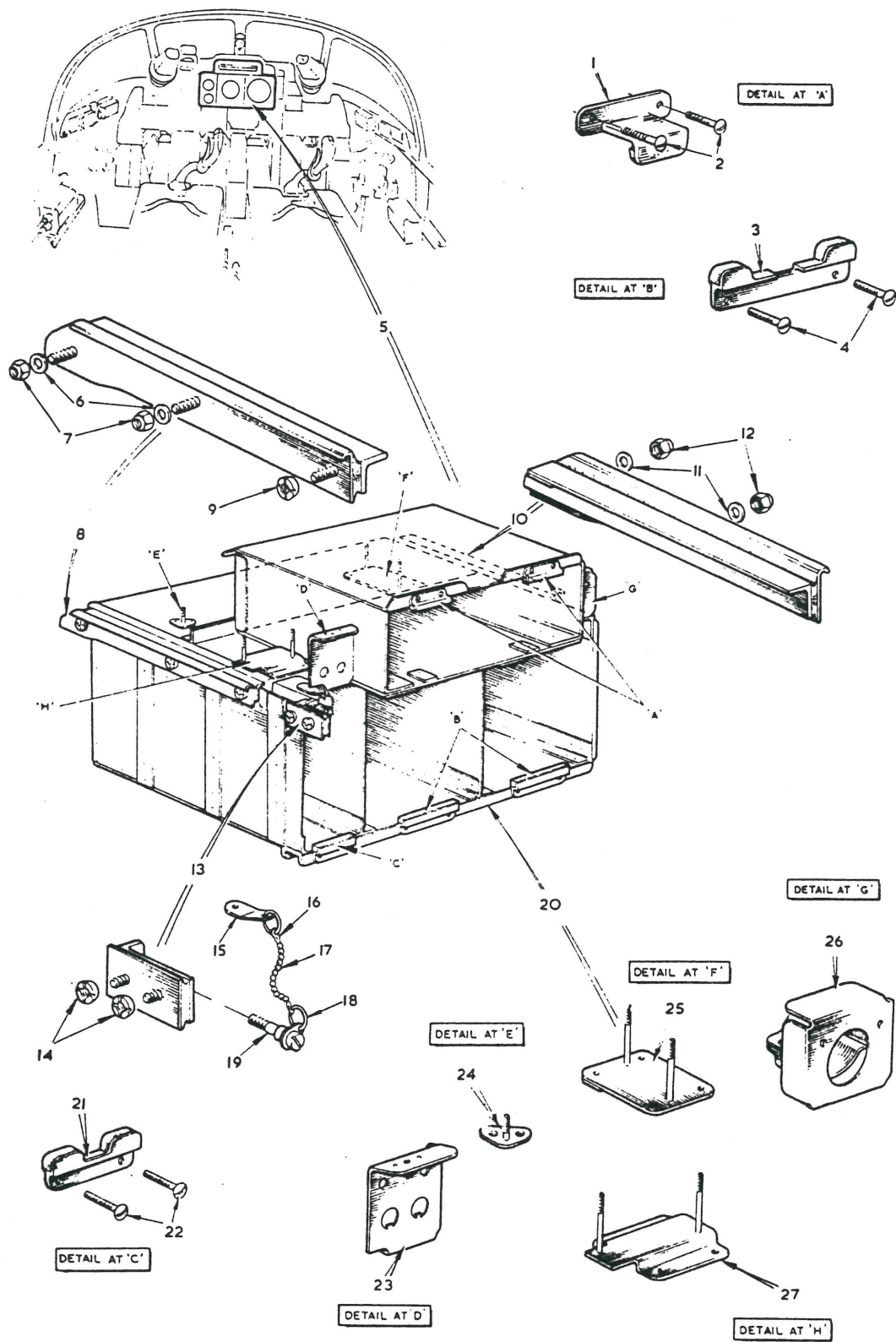
FIG. 5 PILOTS INSTRUMENTS AND CONTROLS Restricted
