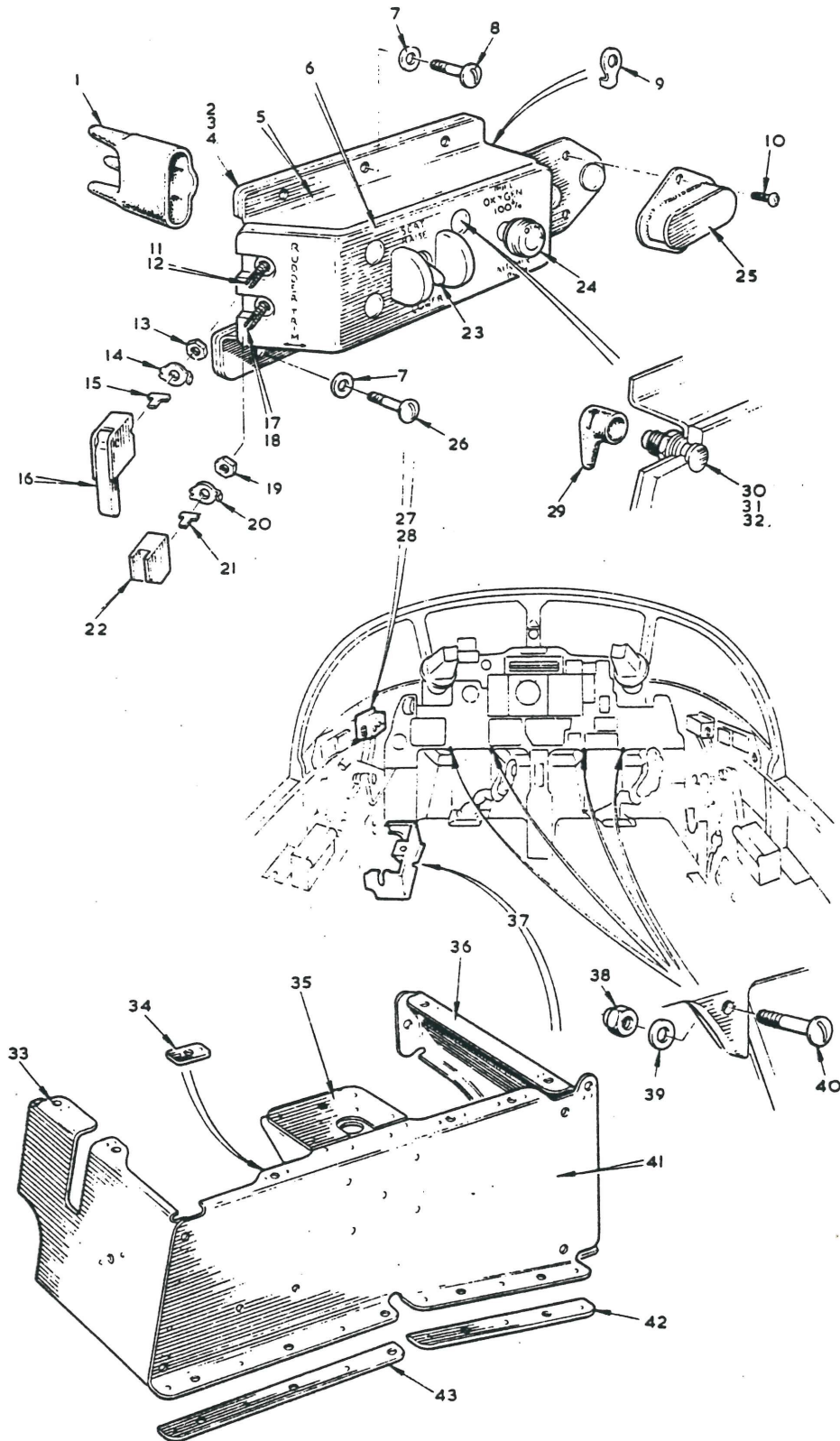
FIG 15. PILOT'S INSTRUMENTS AND CONTROLS Restricted
