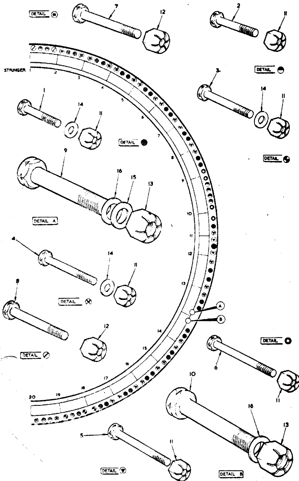
FIG. 1 MISCELLANEOUS ATTACHMENT DETAILS
