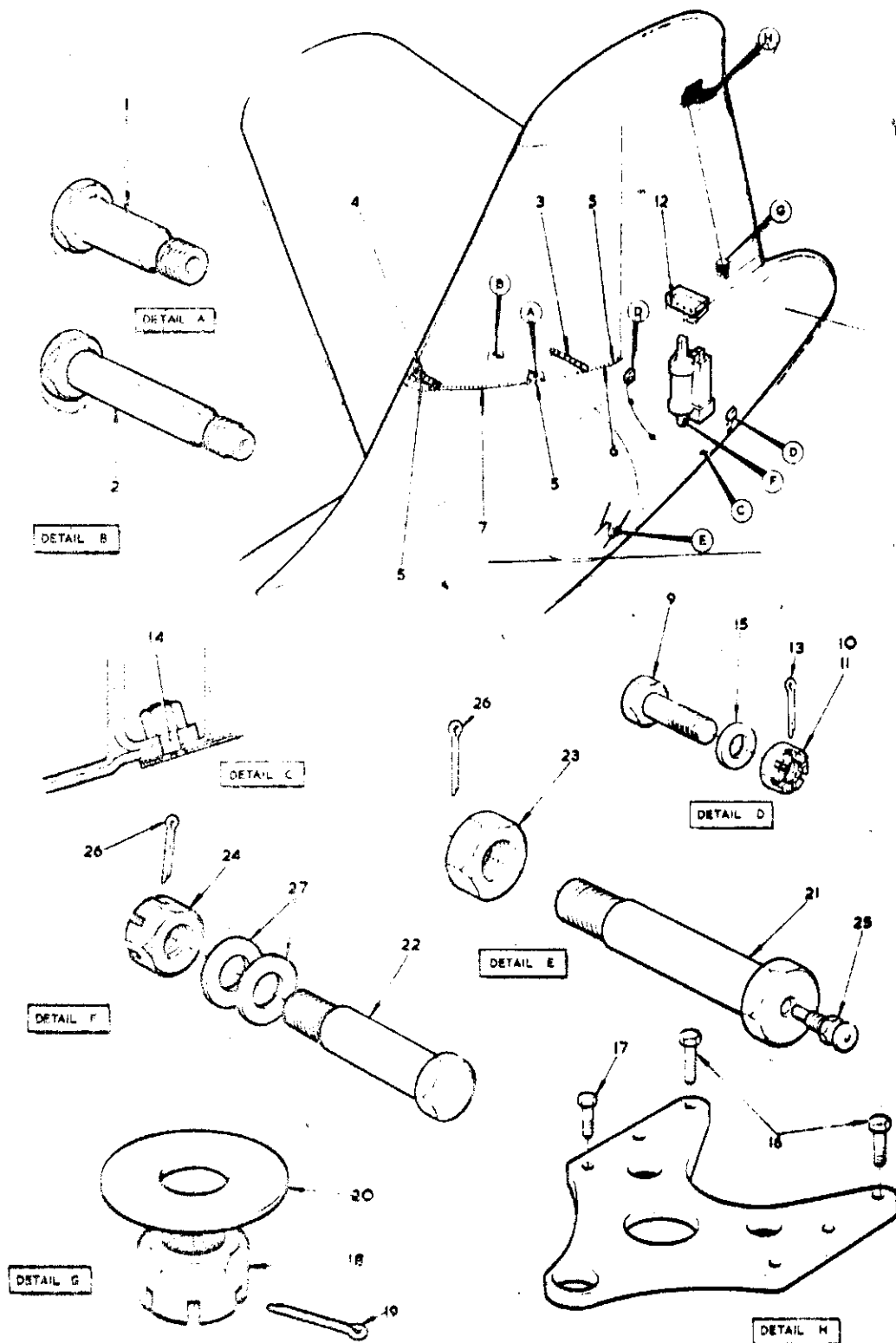
FIG. 4 MISCELLANEOUS ATTACHMENT DETAILS
