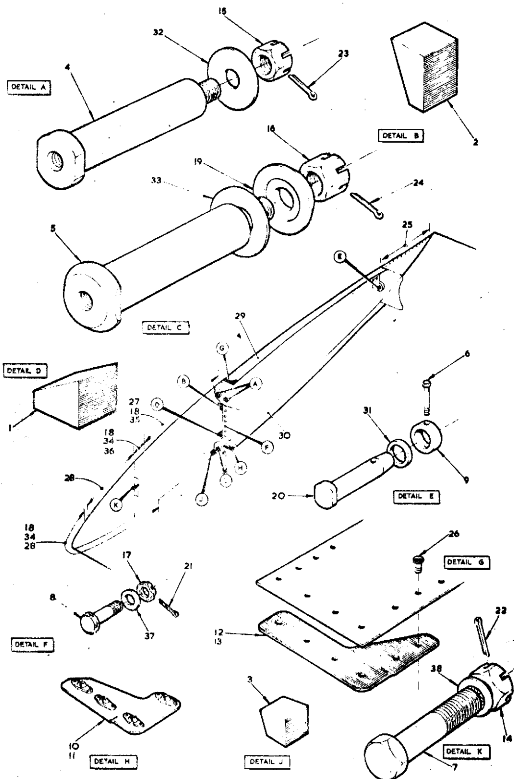
FIG. 3 MISCELLANEOUS ATTACHMENT DETAILS
