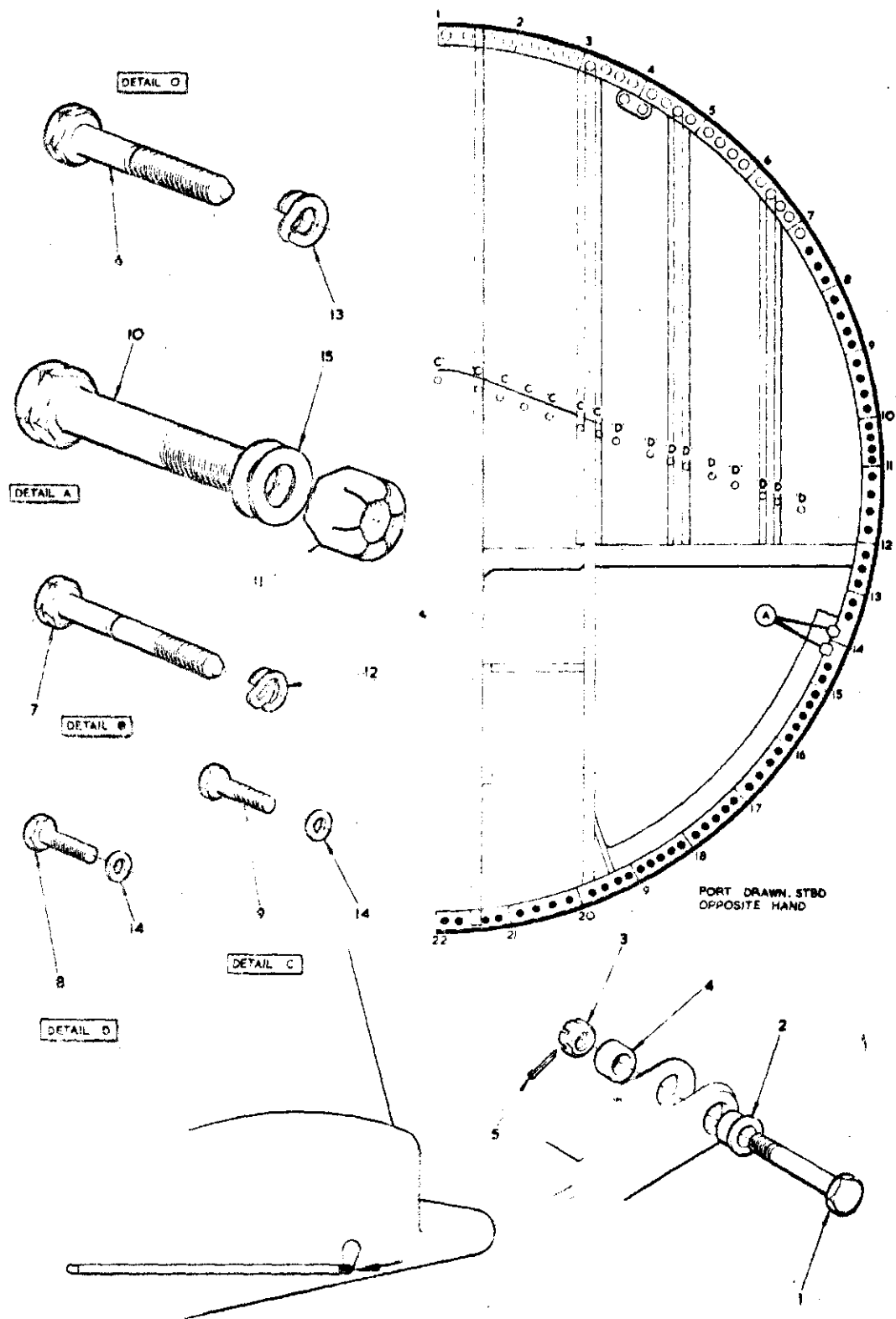
FIG. 2 MISCELLANEOUS ATTACHMENT DETAILS
