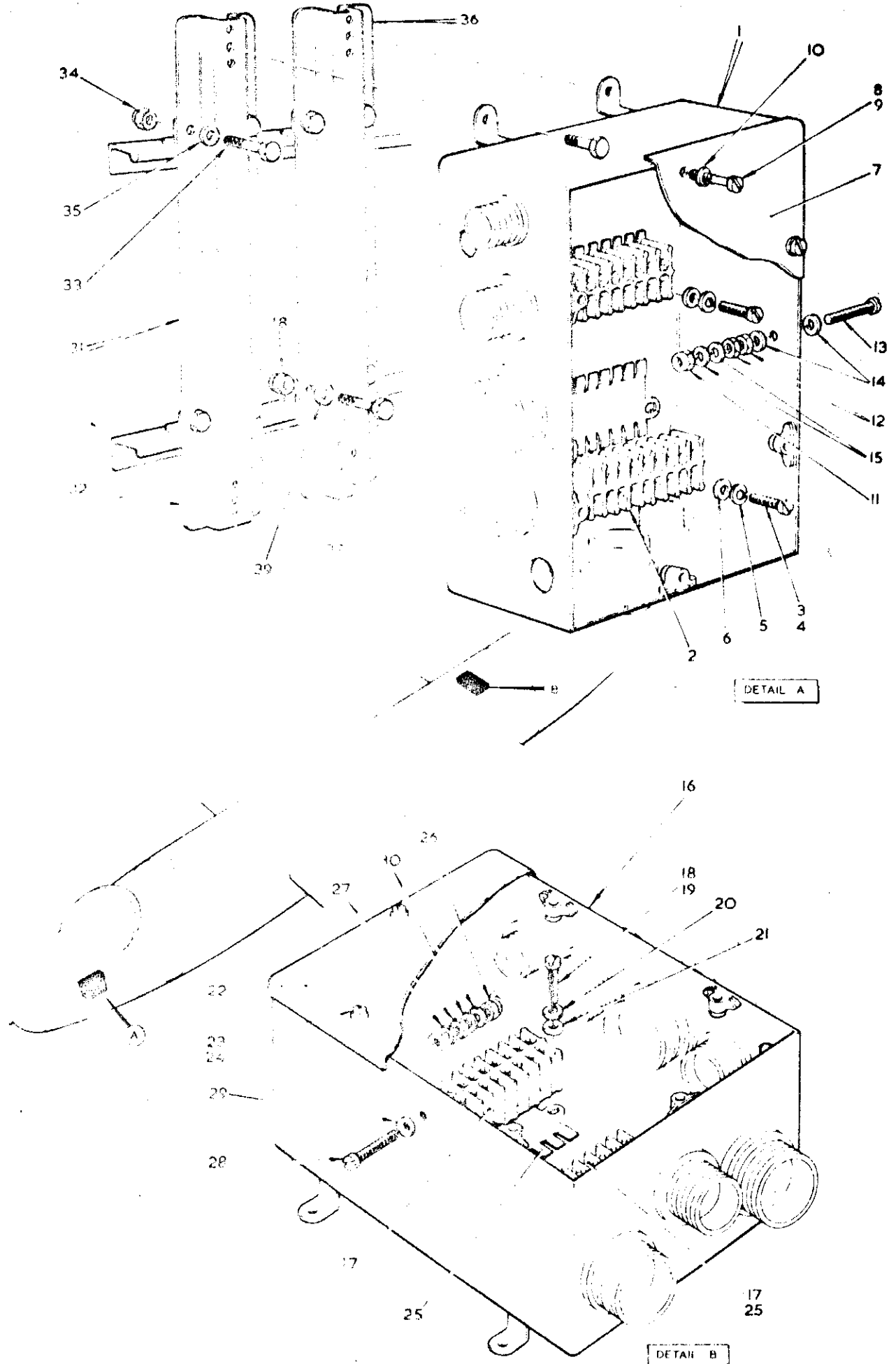
FIG 3 DOPPLER NAVIGATOR
