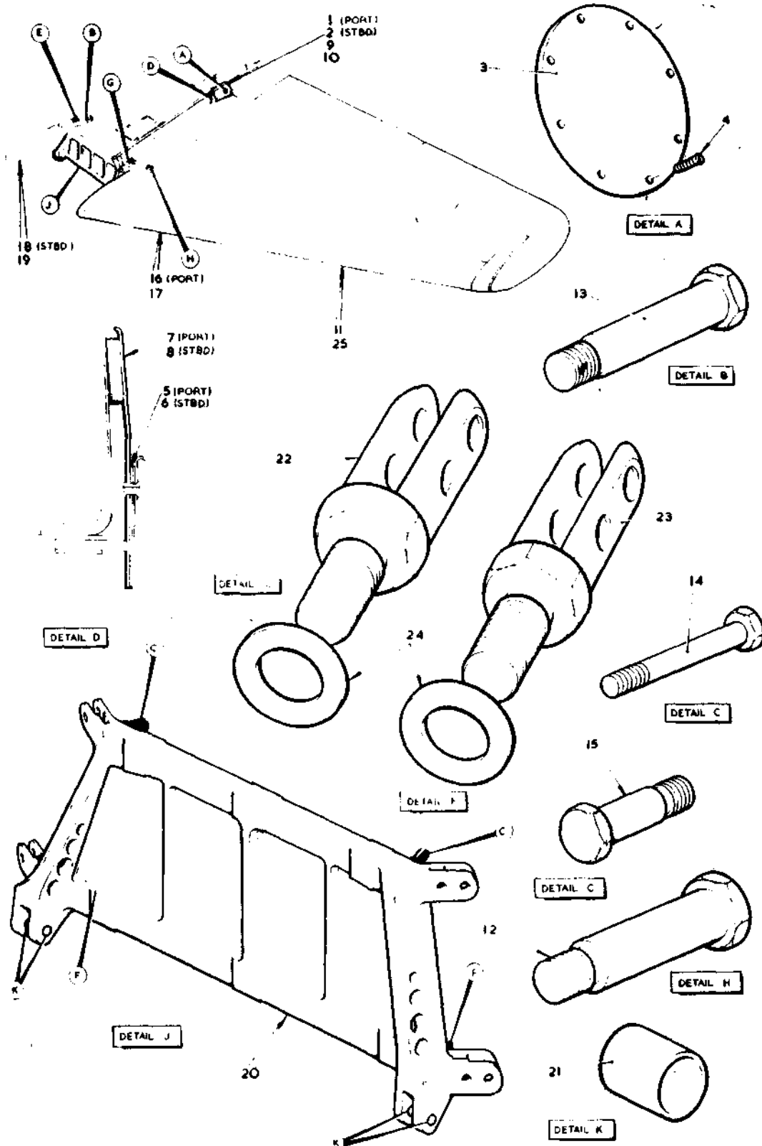
FIG. 7 TAILPLANE AND ELEVATORS
