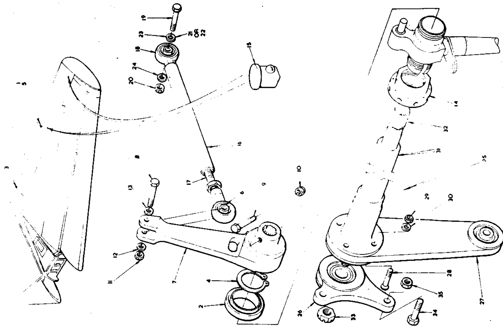
FIG. 5 TAIL UNIT
