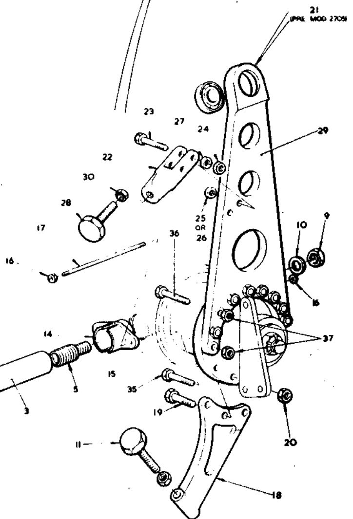
FIG.2 TAIL UNIT
