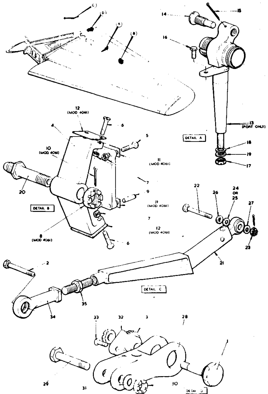
FIG. 6 TAIL UNIT
