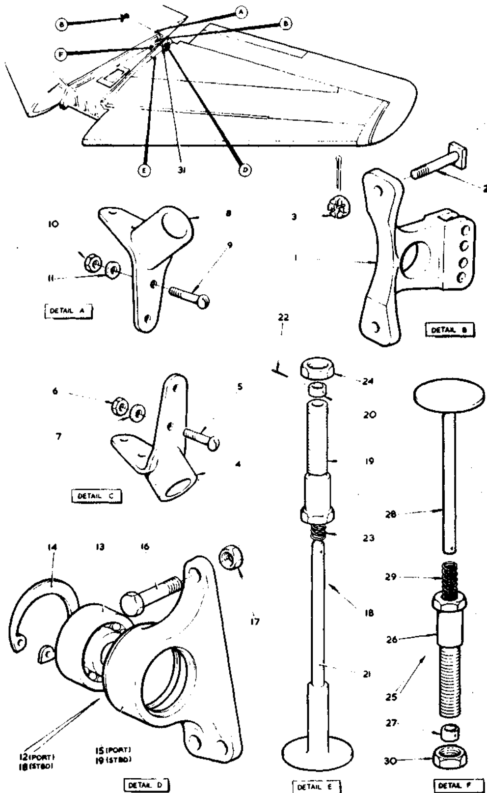
FIG. 9 TAILPLANE AND ELEVATORS
