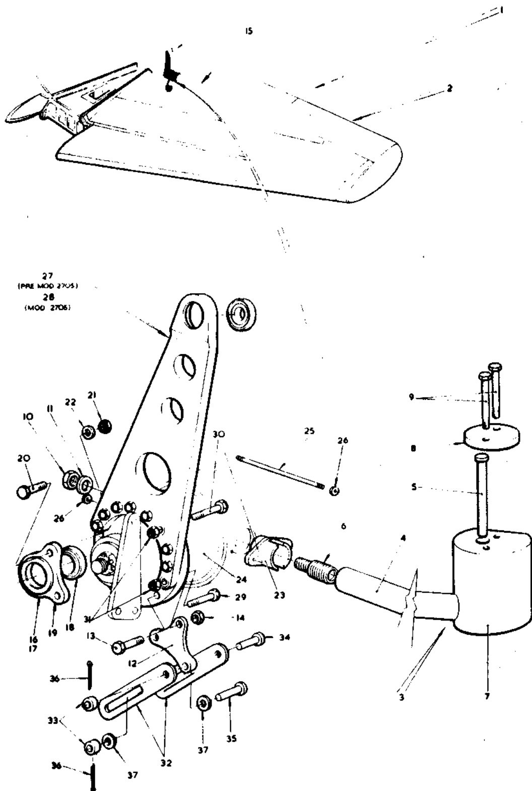
FIG.1 TAIL UNIT
