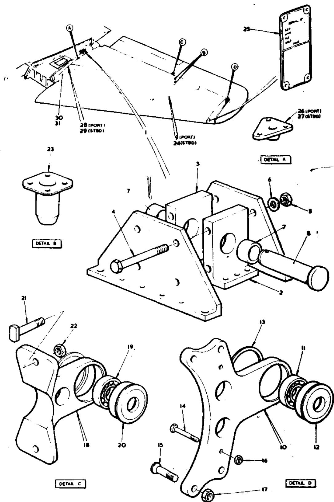
FIG. 8 TAILPLANE AND ELEVATORS
