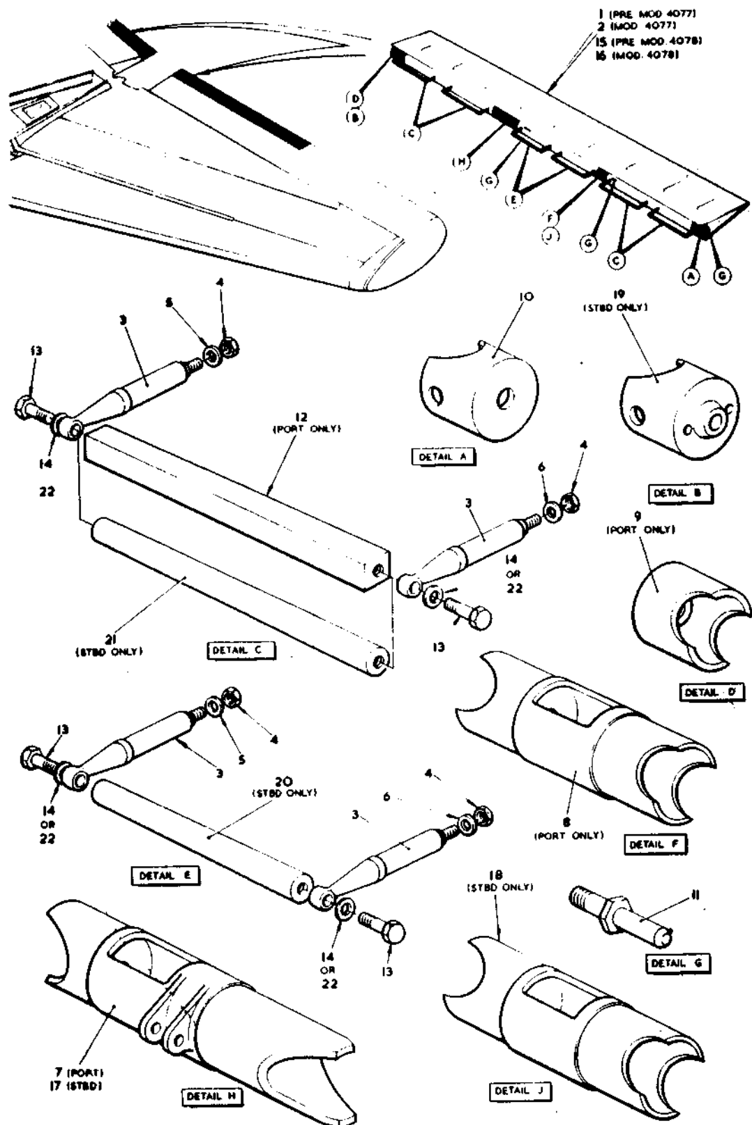
FIG. 4 TAIL UNIT
