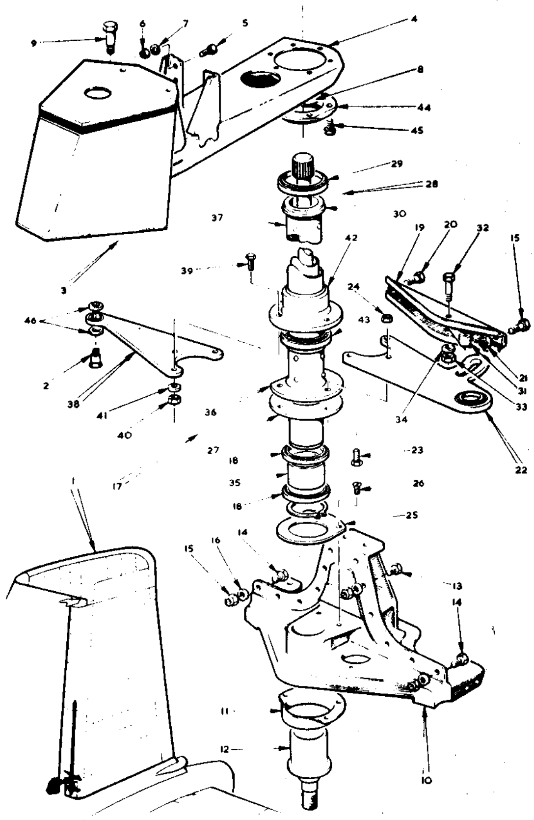
FIG.1 RUDDER C/W TAB
