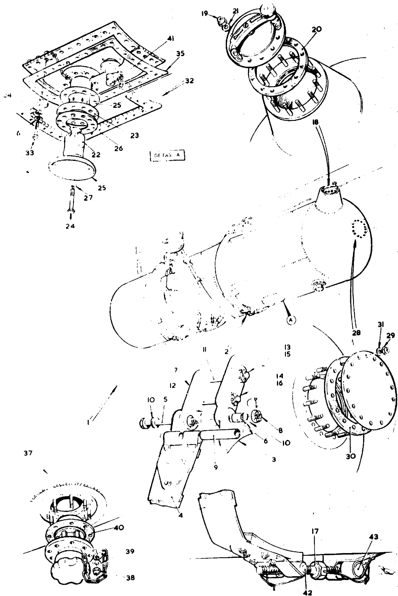
FIG.1 300 GALLON FUEL TANK
