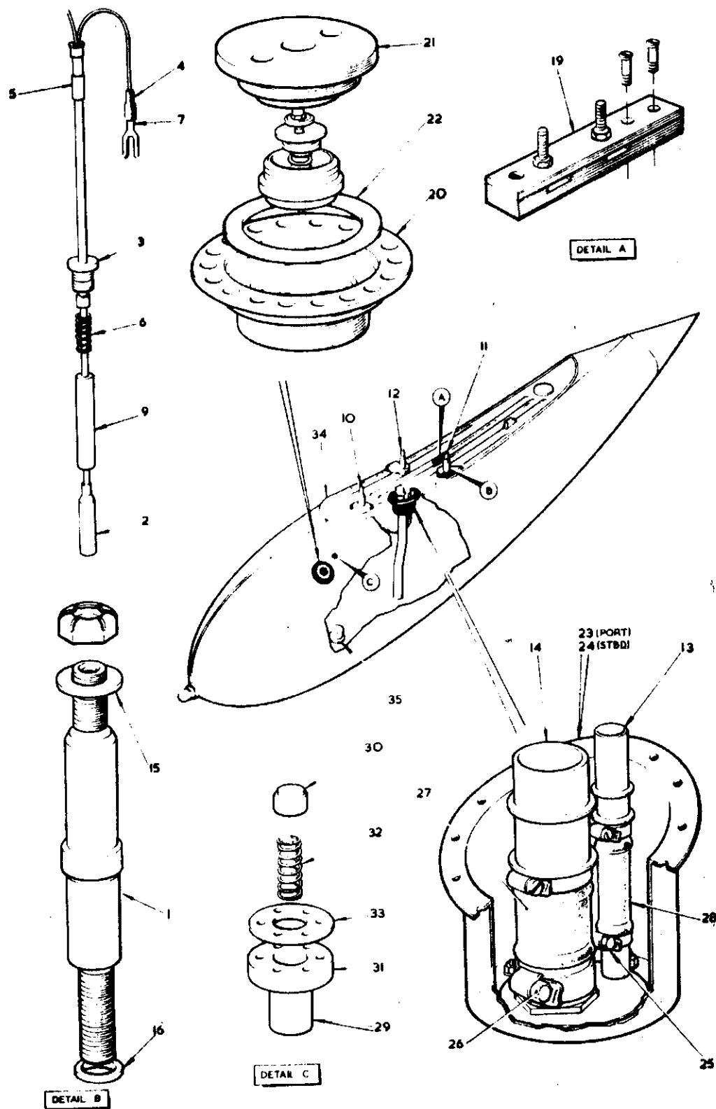
FIG.1 JETTISONABLE WING FUEL TANK
