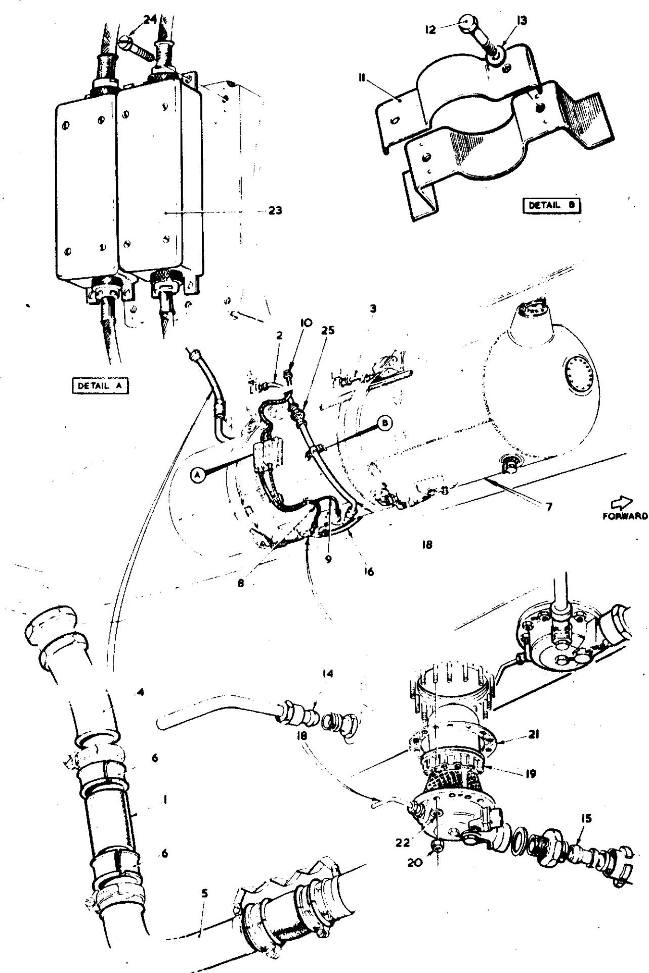
FIG. 2 300 GALLON FUEL TANK
