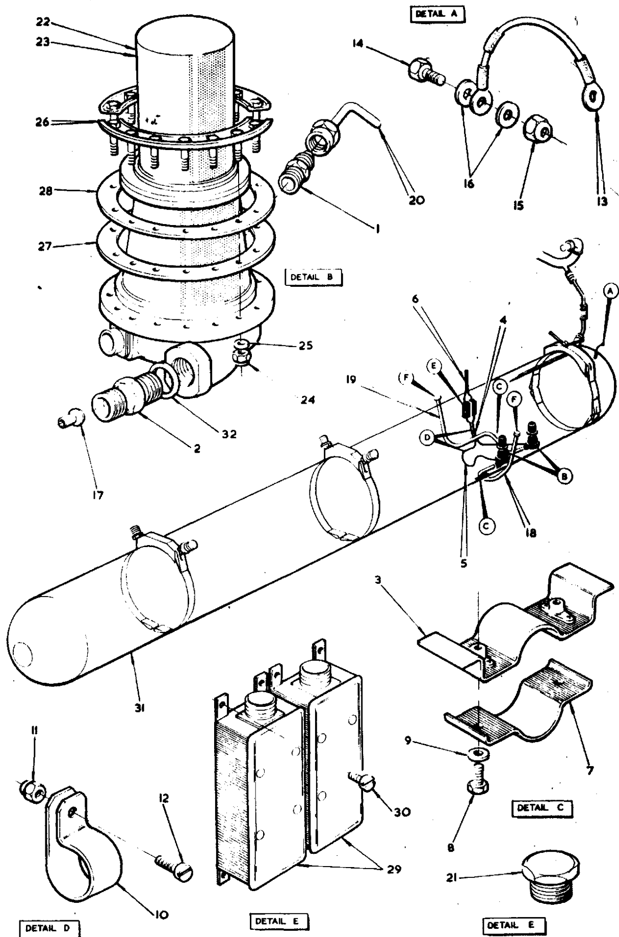
FIG. 2 650 GALLON TANK
