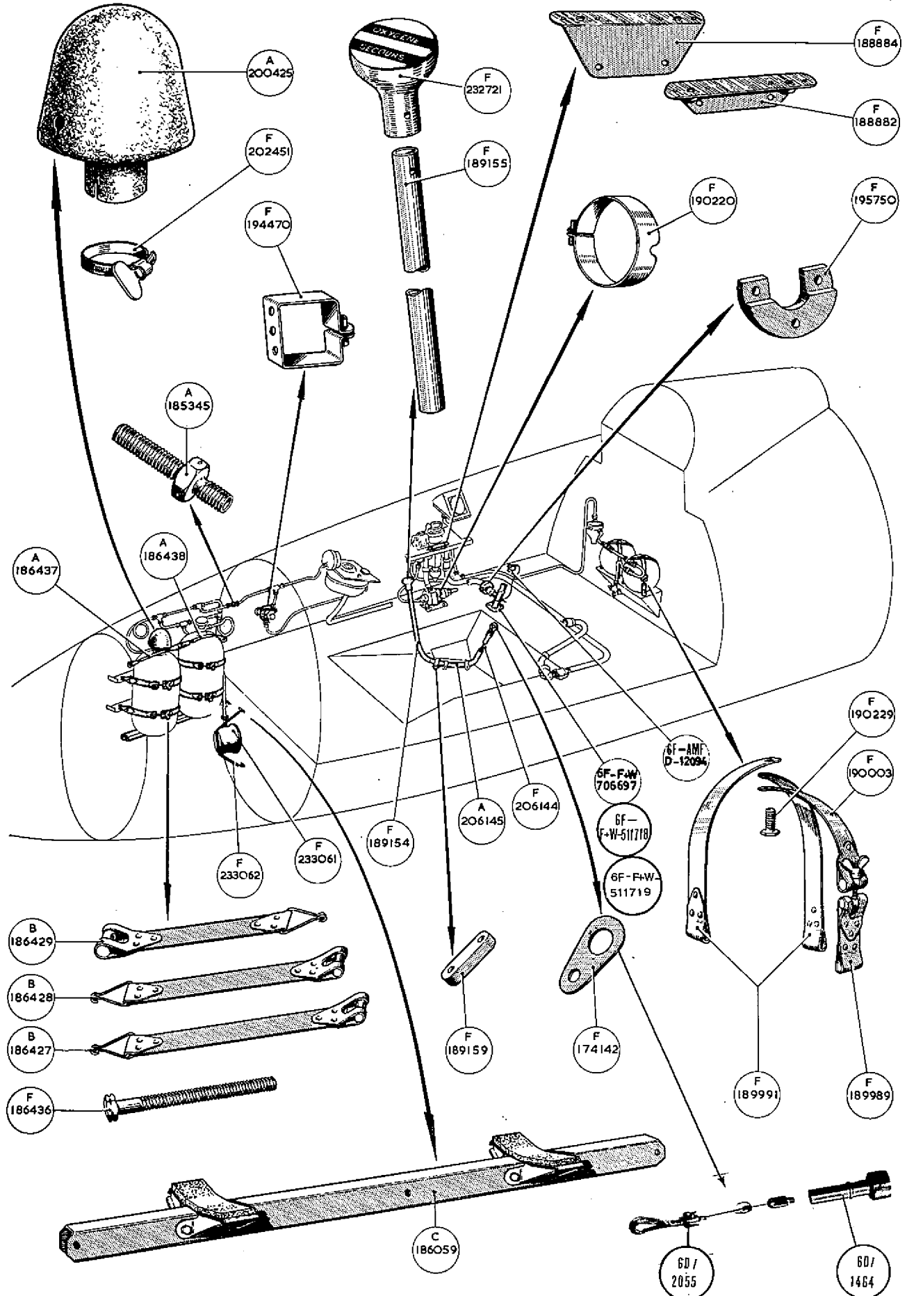
ANTI G &amp; OXYGEN INSTALLATION
