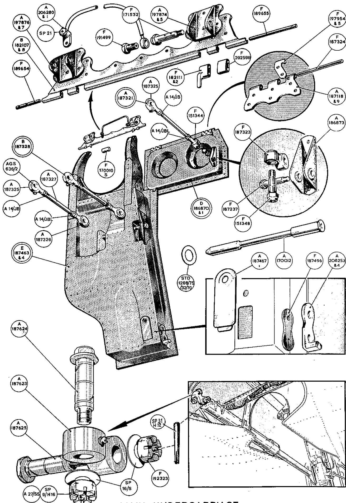
MAIN UNDERCARRIAGE
