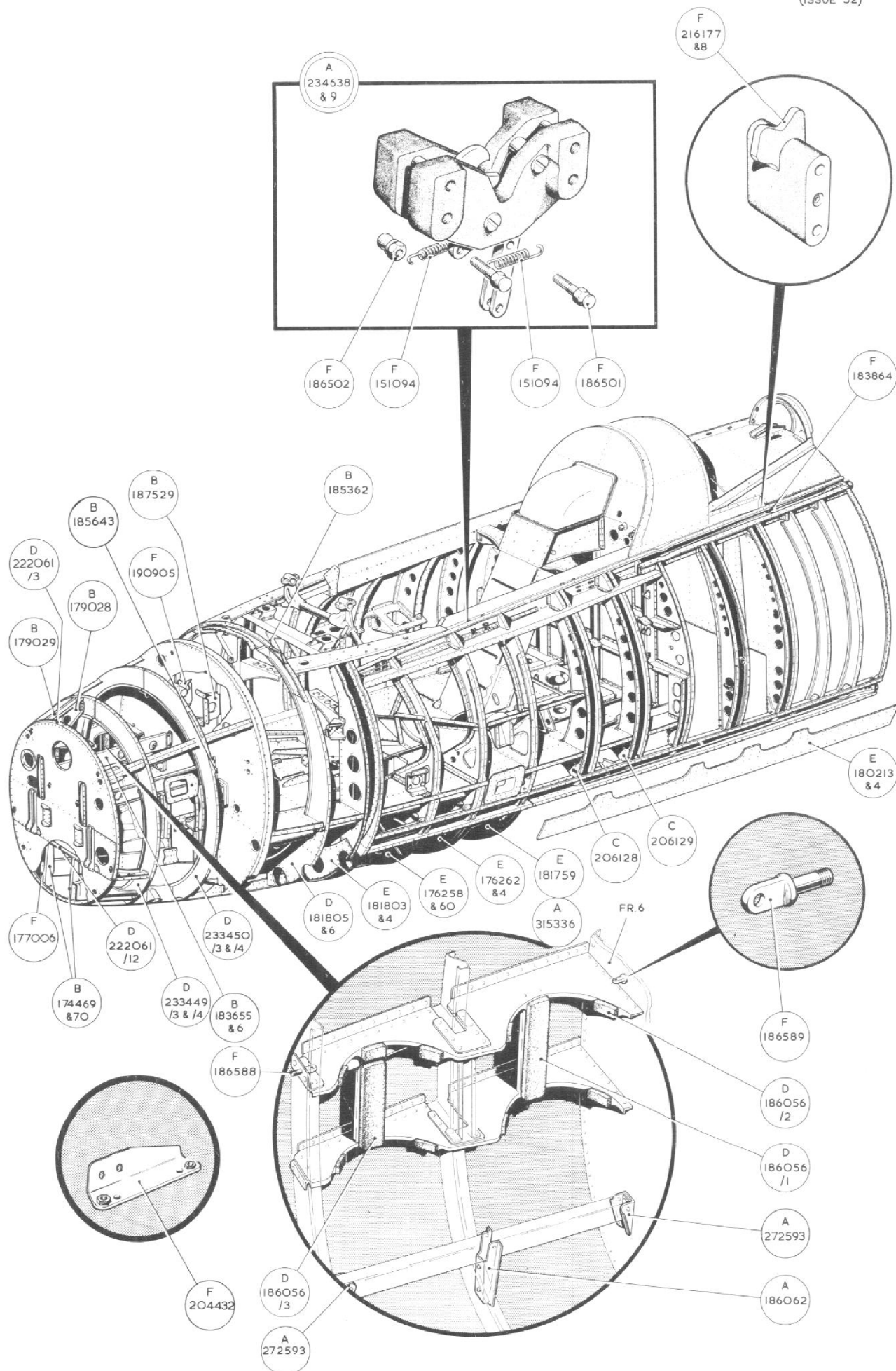
FRONT FUSELAGE
