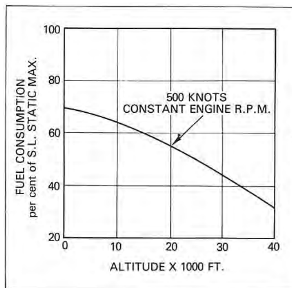
Fig. 10-2 Fuel flow changing with altitude.
