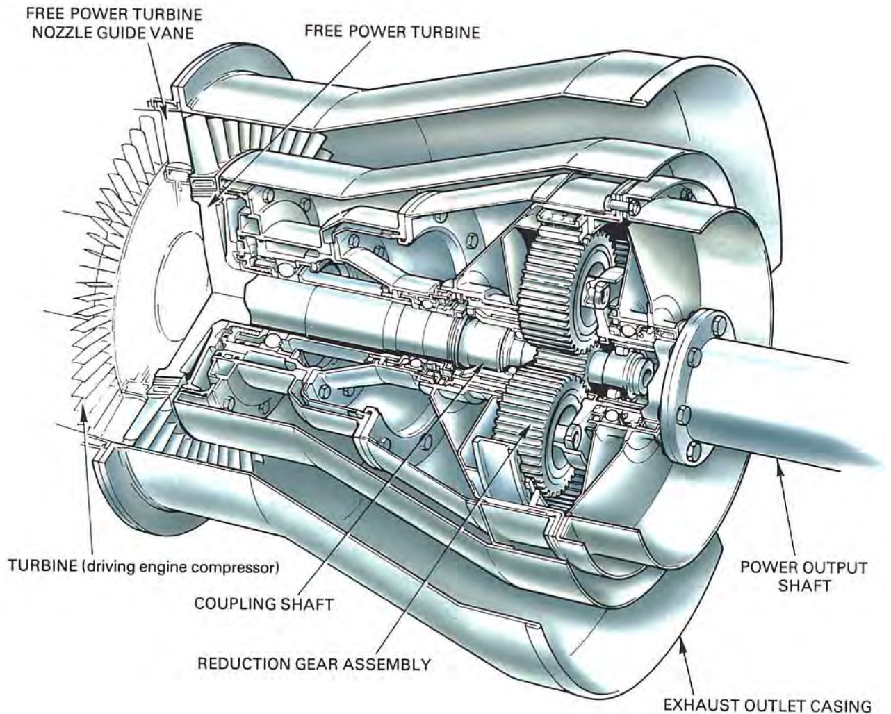
Fig. 5-4 A typical free power turbine.
