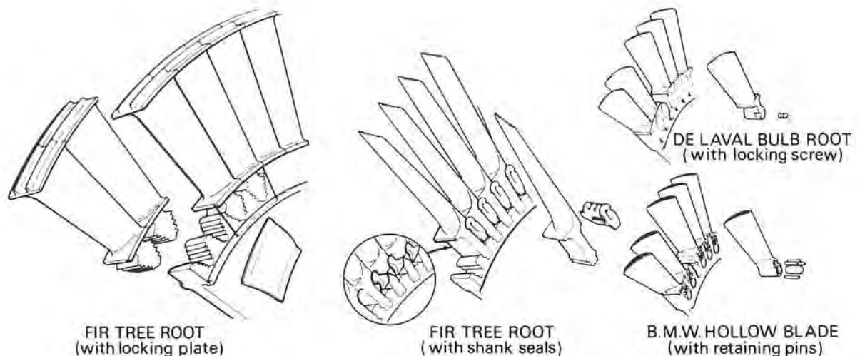
Fig. 5-9 Various methods of attaching blades to turbine discs.
