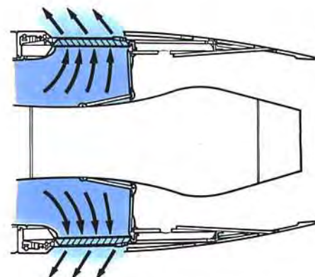
COLD STREAM REVERSER IN REVERSE THRUST POSITION
