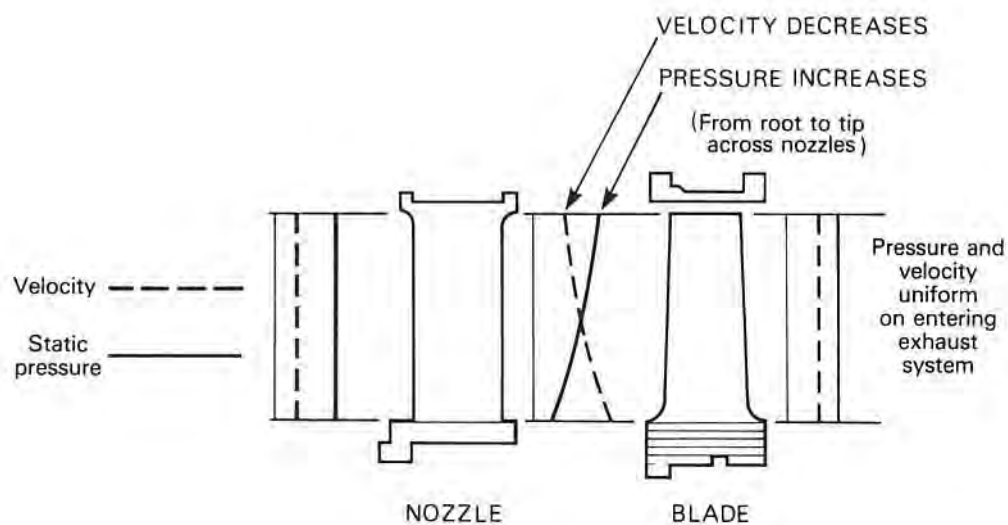
Fig. 5-7 Gas flow pattern through nozzle and blade.
