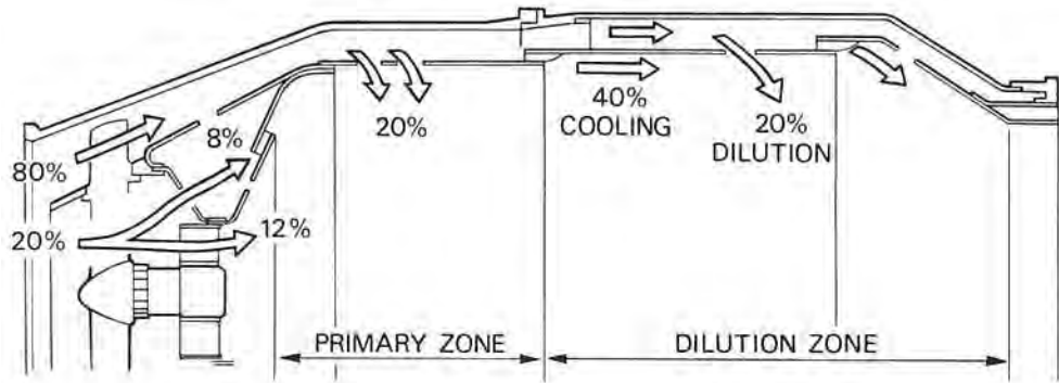
Fig. 4-2 Apportioning the airflow.
