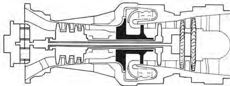
TWIN-SPOOL TURBO-SHAFT (with free-power turbine)
