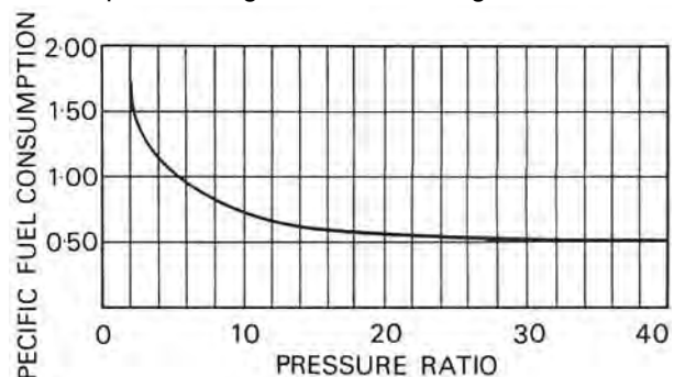
Fig. 3-2 Specific fuel consumption and pressure ratio.
