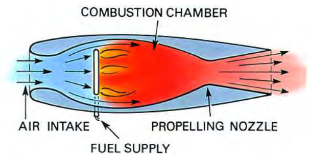
Fig. 1-1 Lorin's jet engine.
