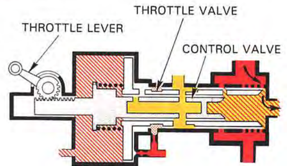
CLOSED POSITION
