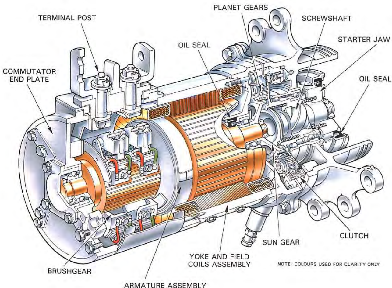
Fig. 11-2 An electric starter.
