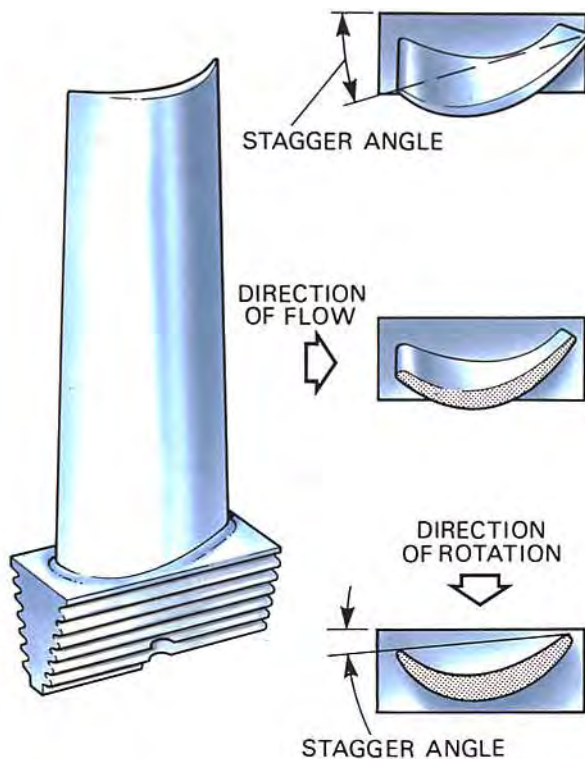
Fig. 5-6 A typical turbine blade showing twisted contour.
