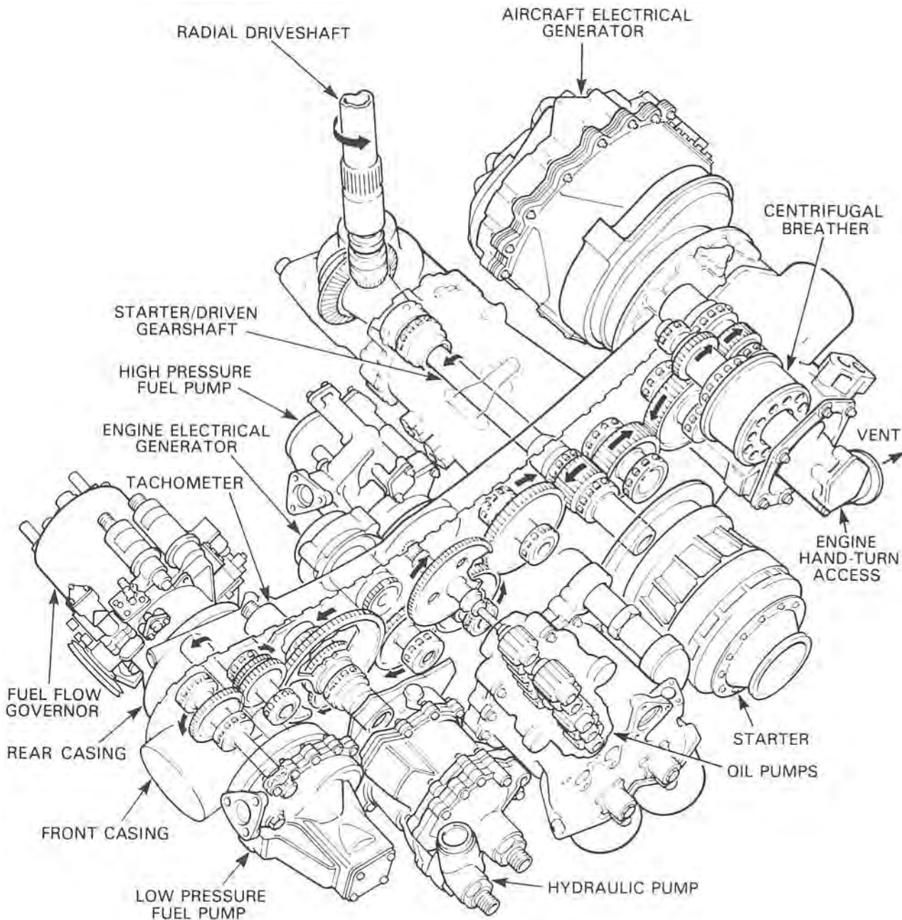
Fig. 7-4 An external gearbox and accessory units.
