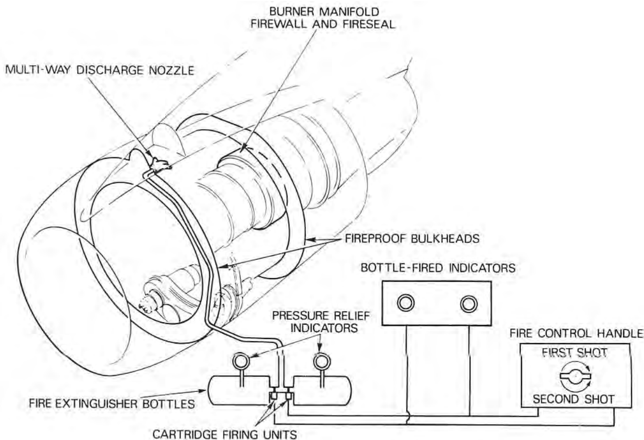
Fig. 14-4 A typical fire extinguishing system.
