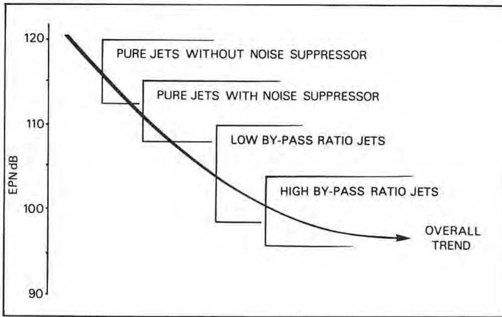
Fig. 19-1 Comparative noise levels of various engine types.
