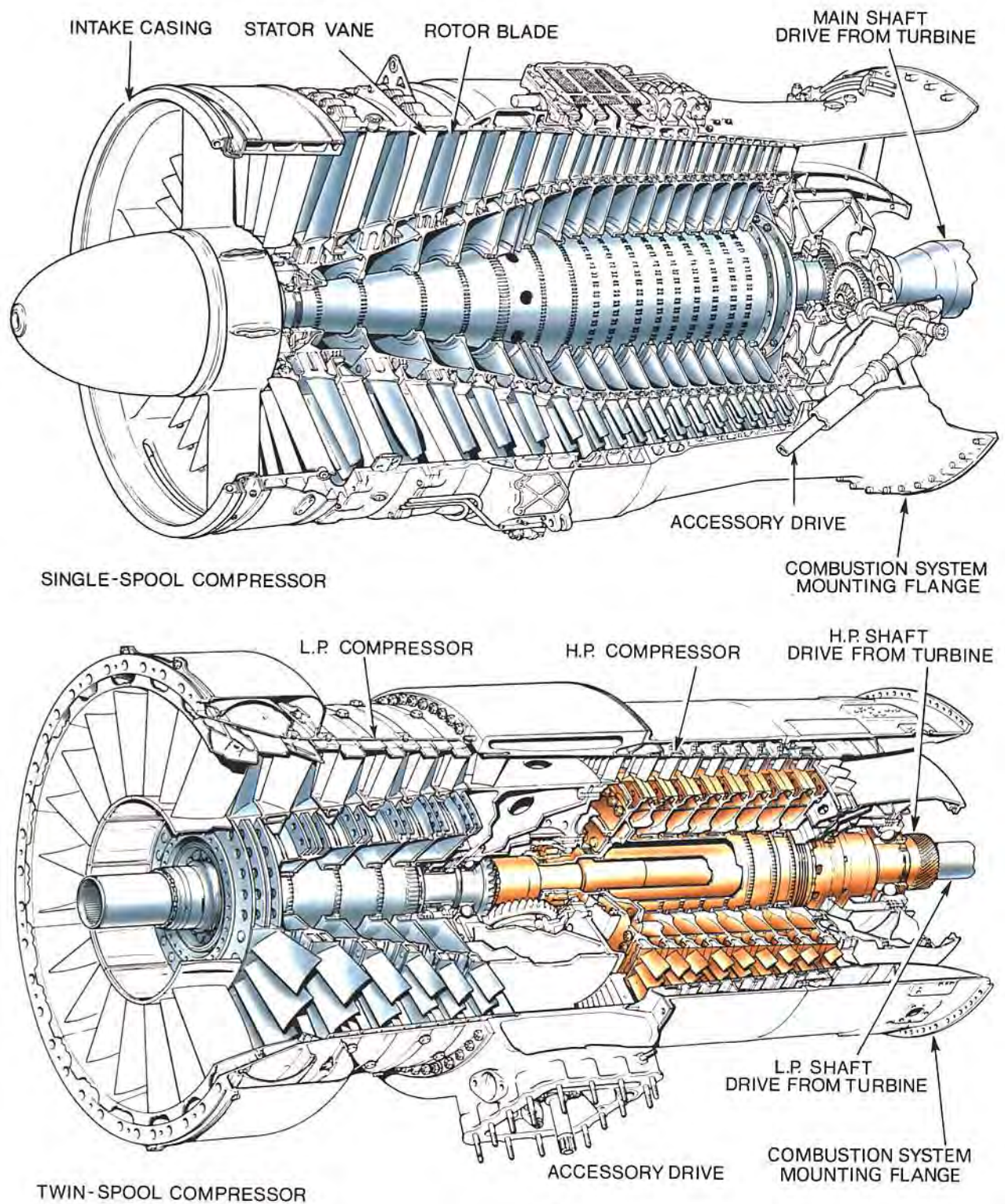
Fig. 3-7 Typical axial flow compressors.
