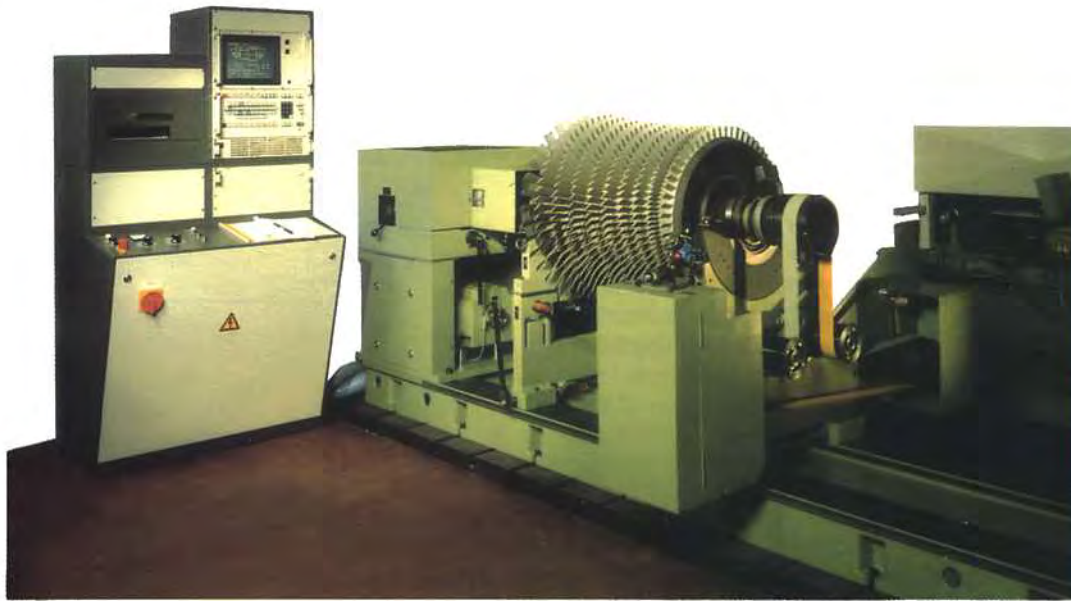
Fig. 25-6 Dynamic balancing machine.
