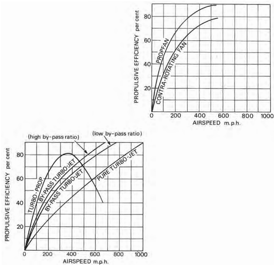
Fig. 21-9 Propulsive efficiencies and aircraft speed.
