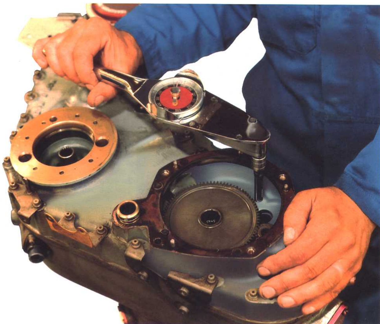
Fig. 25-12 Torque tightening.
