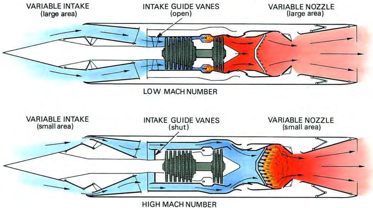
Fig. 1-11 A turbo/ram jet engine.
