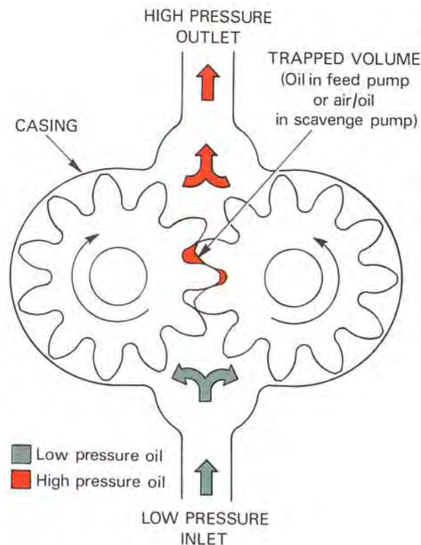
Fig. 8-5 Principle of a gear pump.
