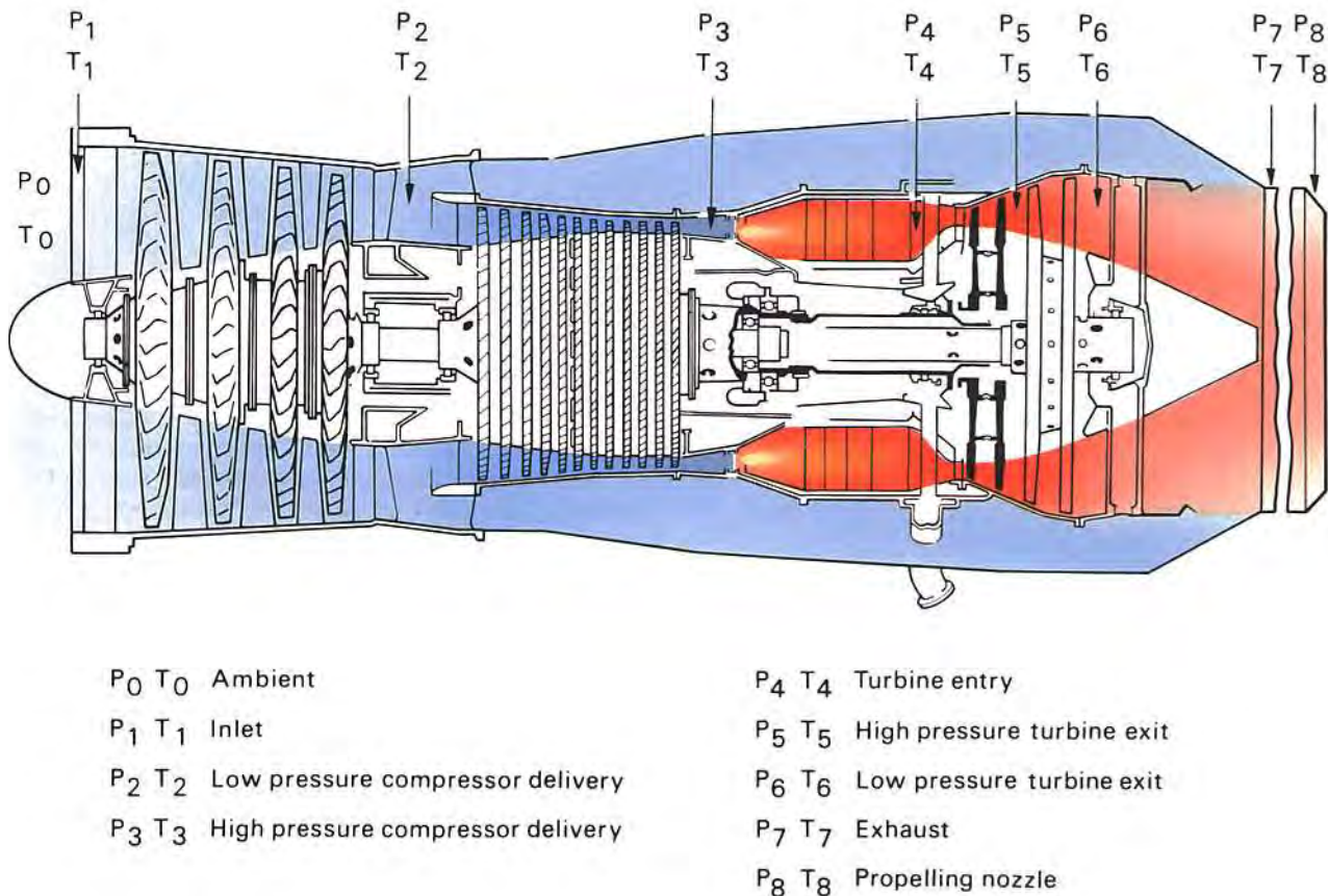
Fig. 21-1 Temperature and pressure notation of a typical turbo-jet engine.
