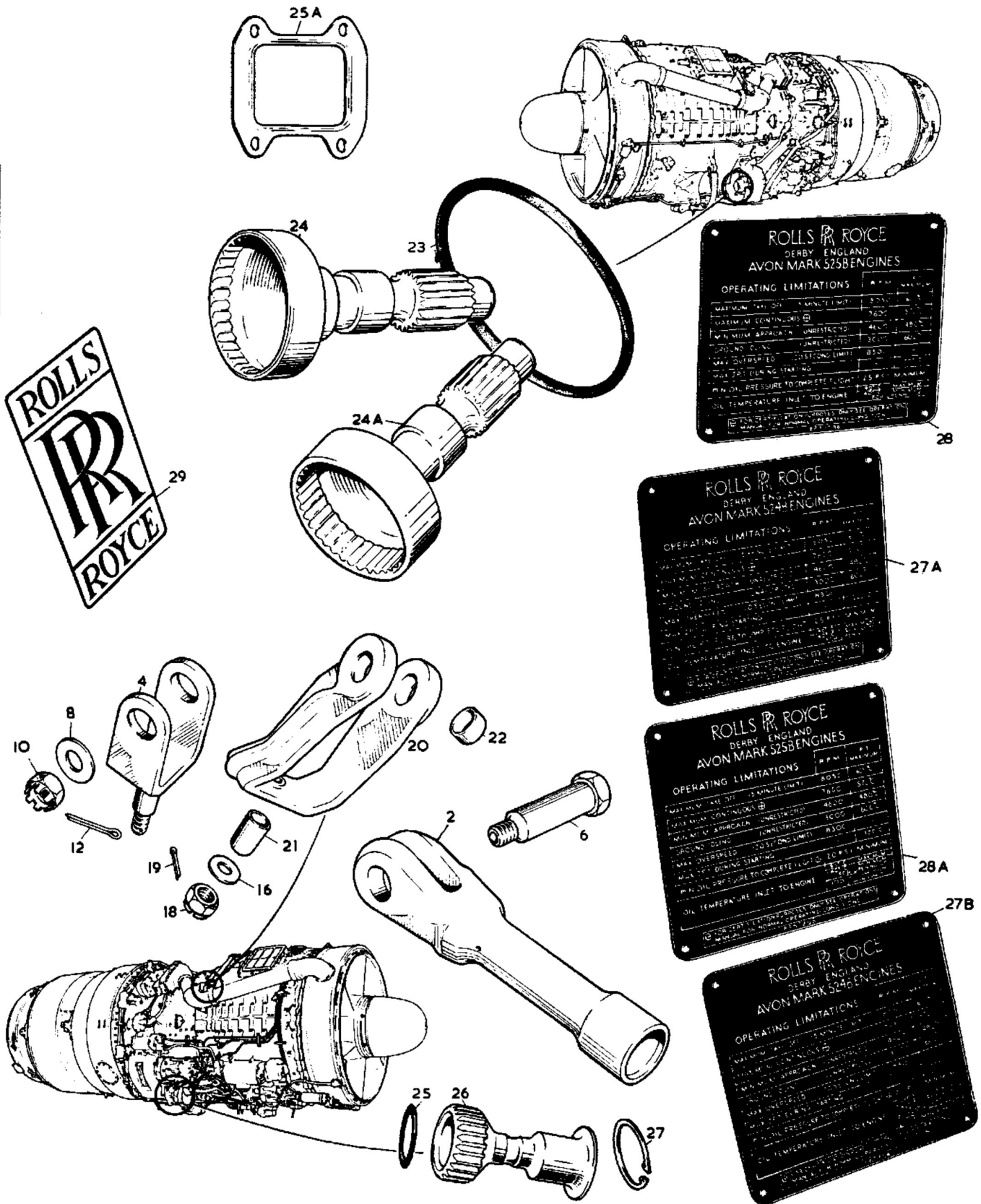
Figure 1 Engine Installation Fittings
