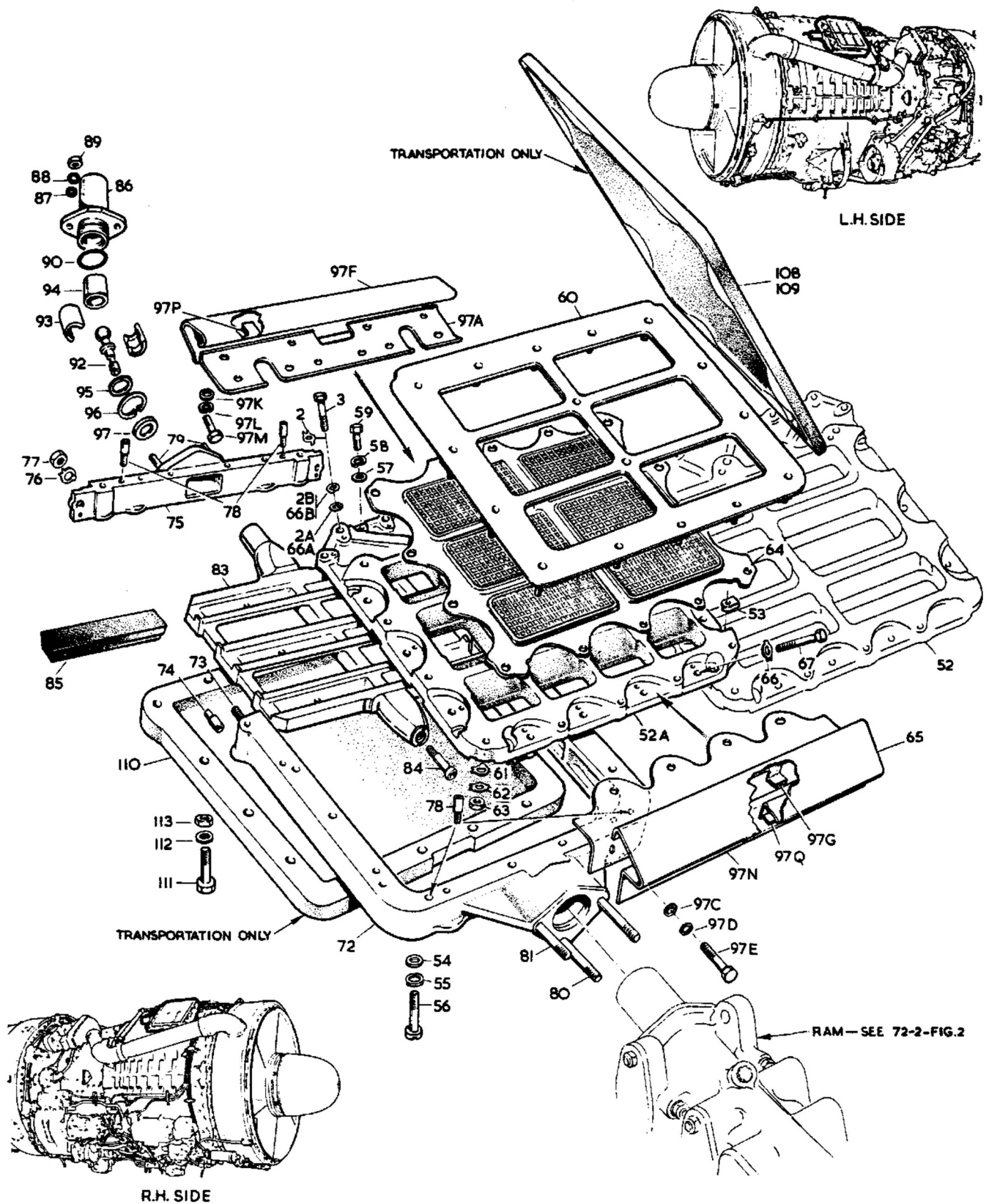
72-2 Figure 1 Compressor Bleed Valves
