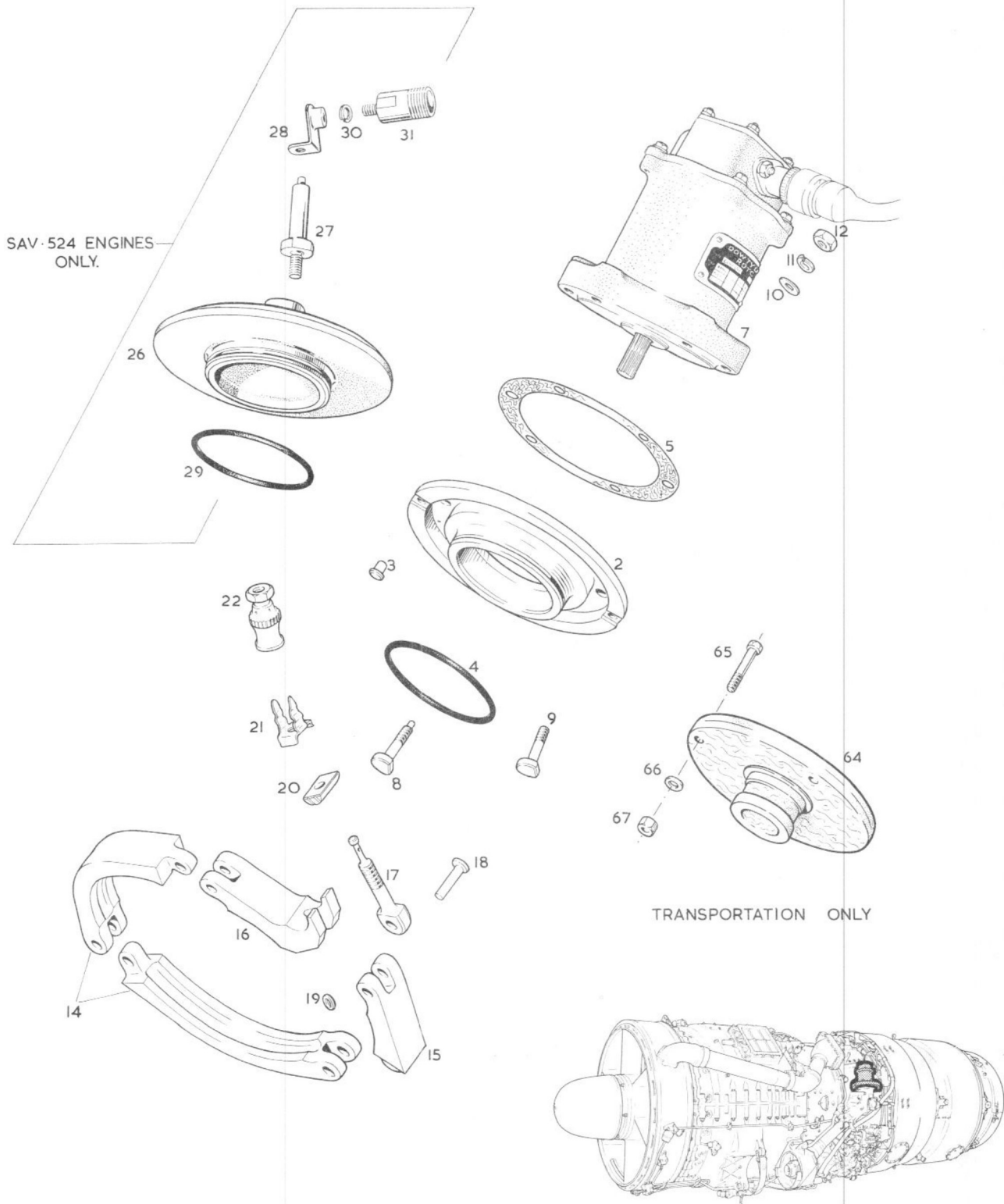
Figure 1 R.P.M. Synchroniser Alternator
