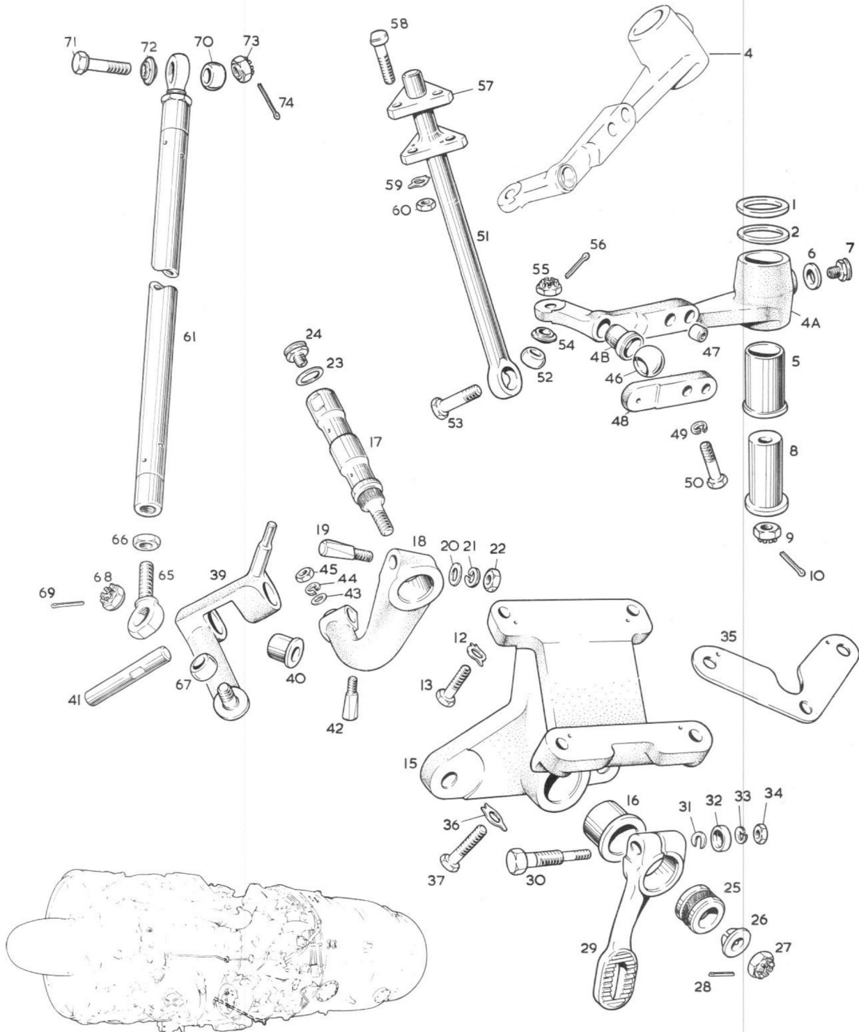
76-1 Figure 1 Control Linkage
