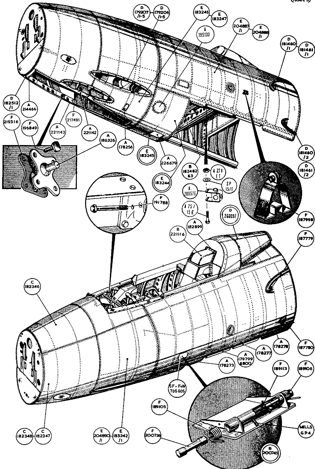
FRONT FUSELAGE
