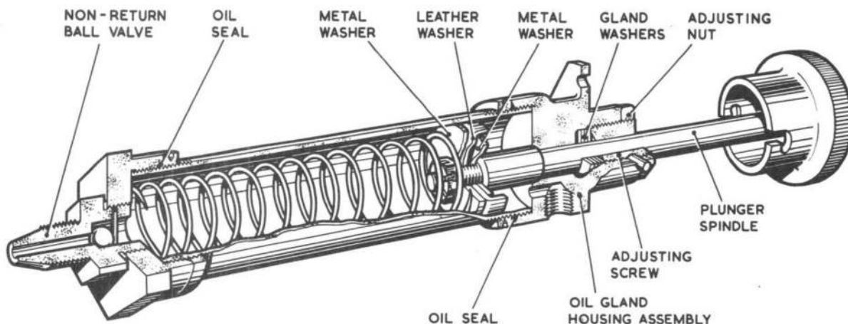
Fig.6. Rotax hand pump, Type M.2601/1
