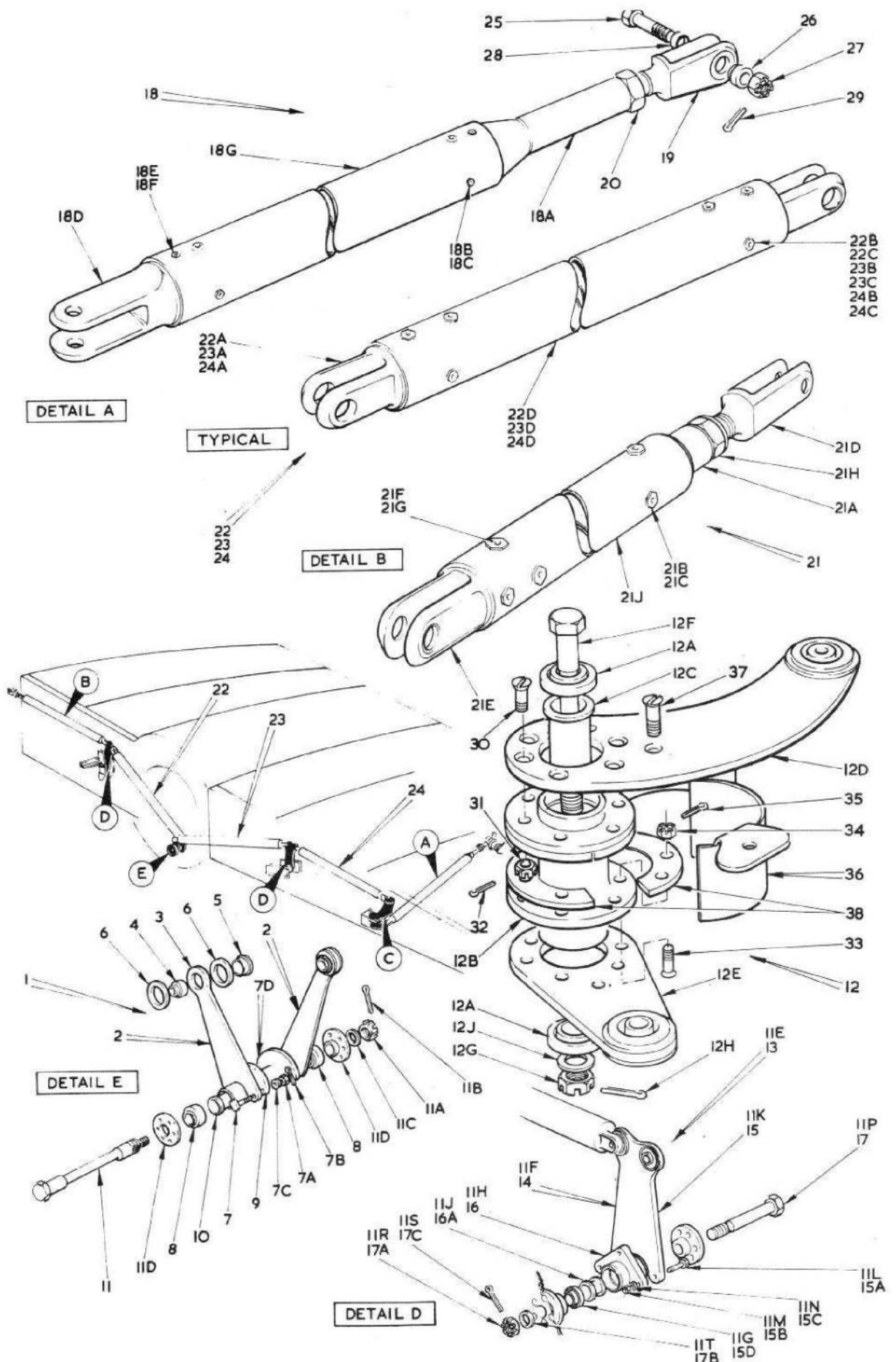
FIG. 1 AILERON CONTROLS IN WING
