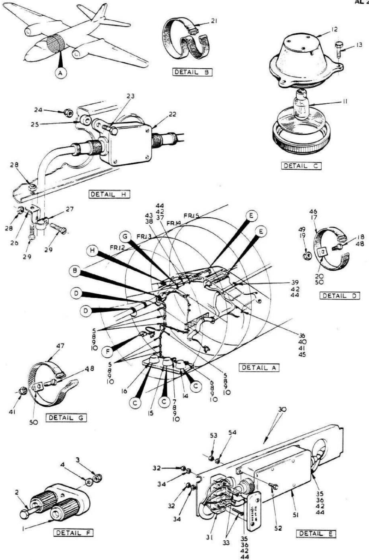
FIG. 9 ELECTRICAL EQUIPMENT IN CENTRE FUSELAGE
