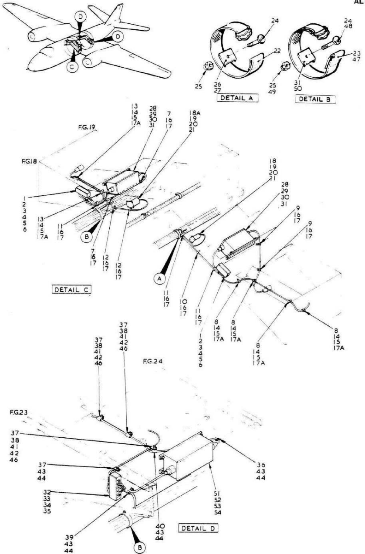
FIG. 10 ELECTRICAL EQUIPMENT IN CENTRE FUSELAGE
