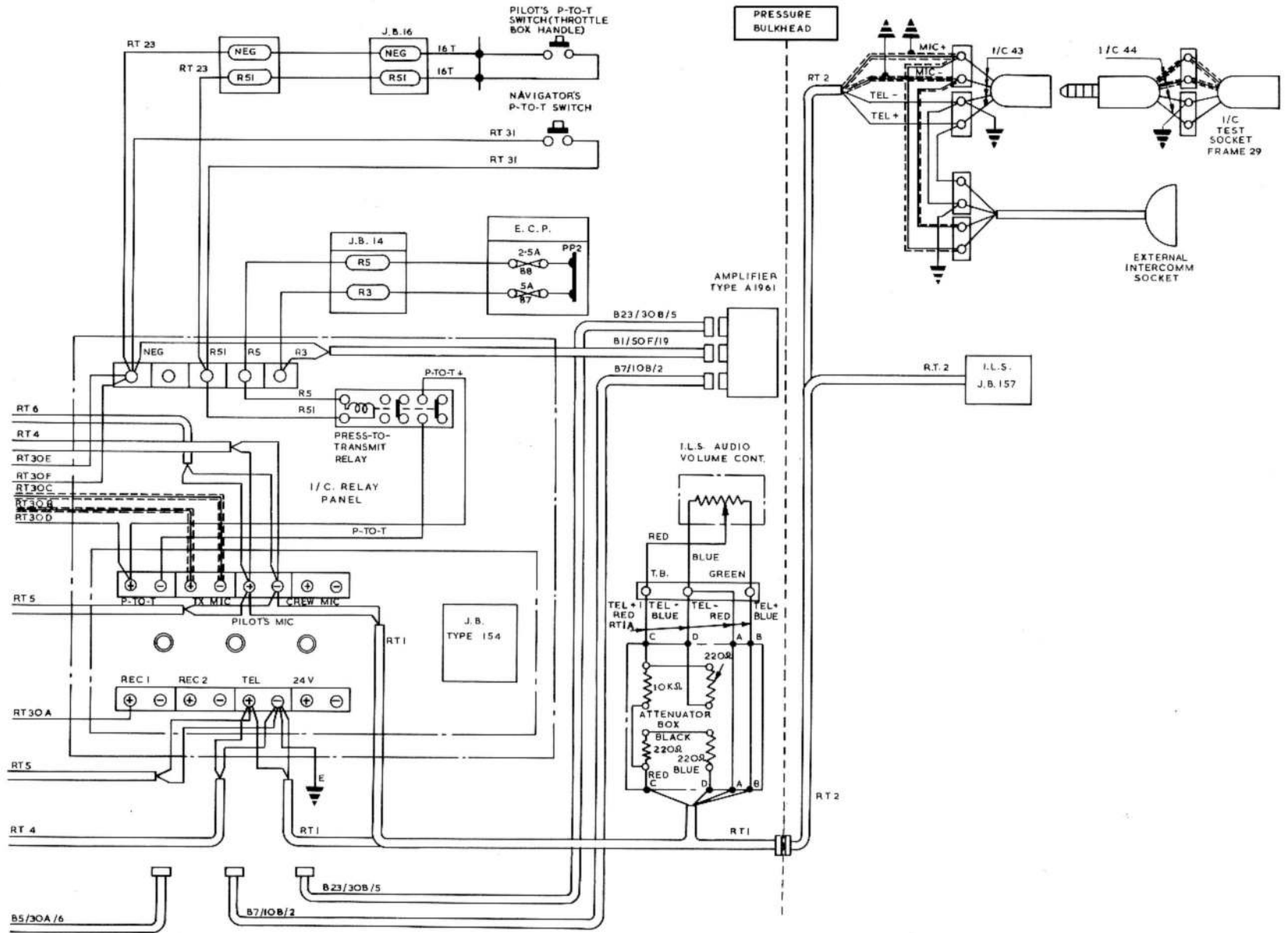
FIG. 2A. INTERCOMMUNICATION ( B (I) MK.6 AIRCRAFT )
