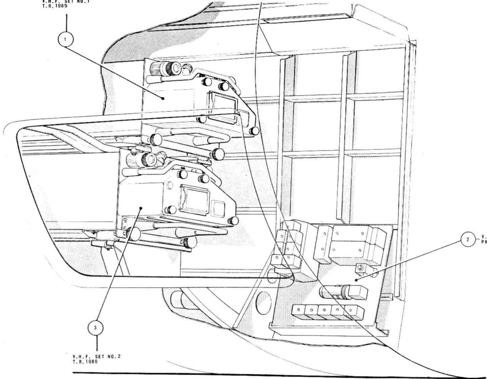
FIG.18. WIRELESS INSTALLATION - PORT EQUIPMENT COMPARTMENT (B MK.6 AIRCRAFT)
