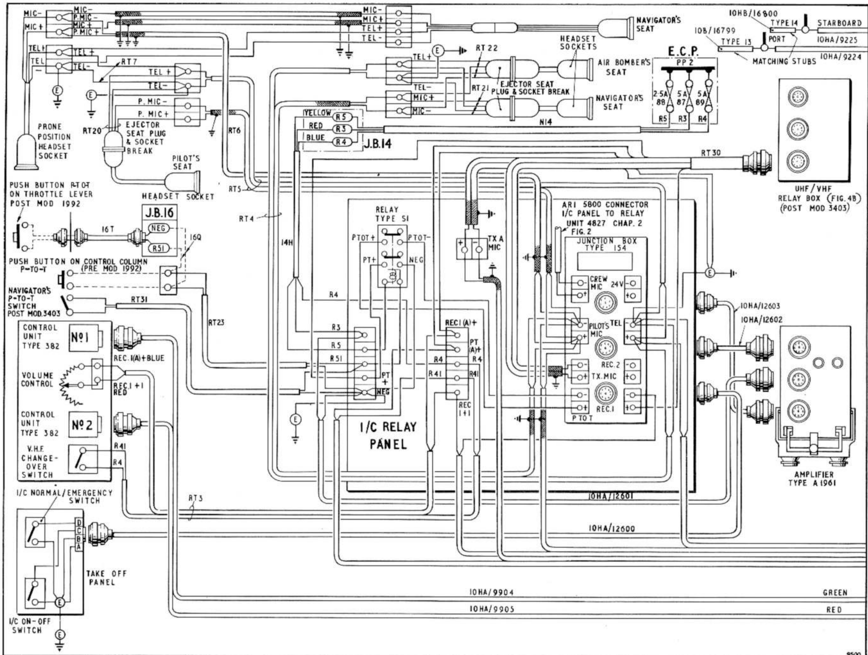
FIG. 1. INTERCOMMUNICATION AND V.H.F. COMMUNICATION ( B MK.6 AIRCRAFT )
