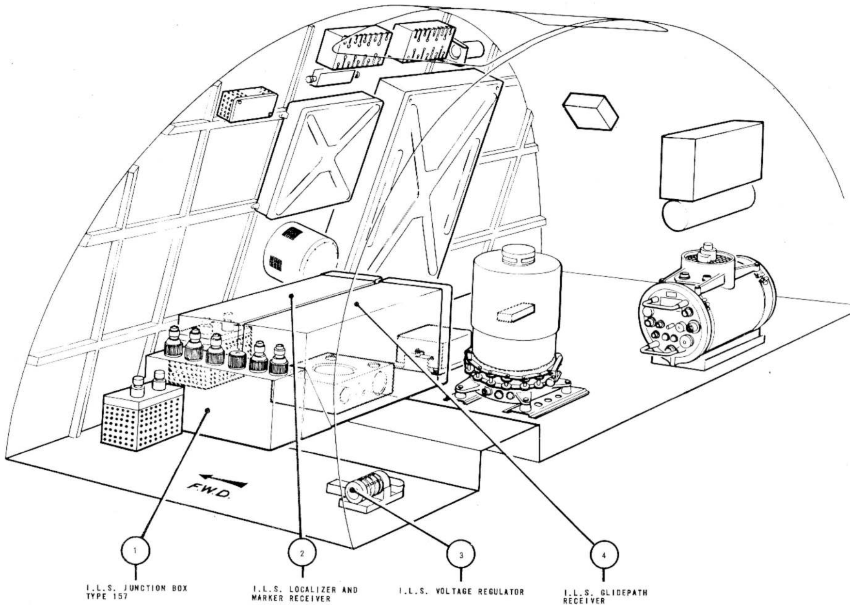
FIG.16. WIRELESS INSTALLATION - UPPER EQUIPMENT COMPARTMENT (B MK.6 AIRCRAFT)
