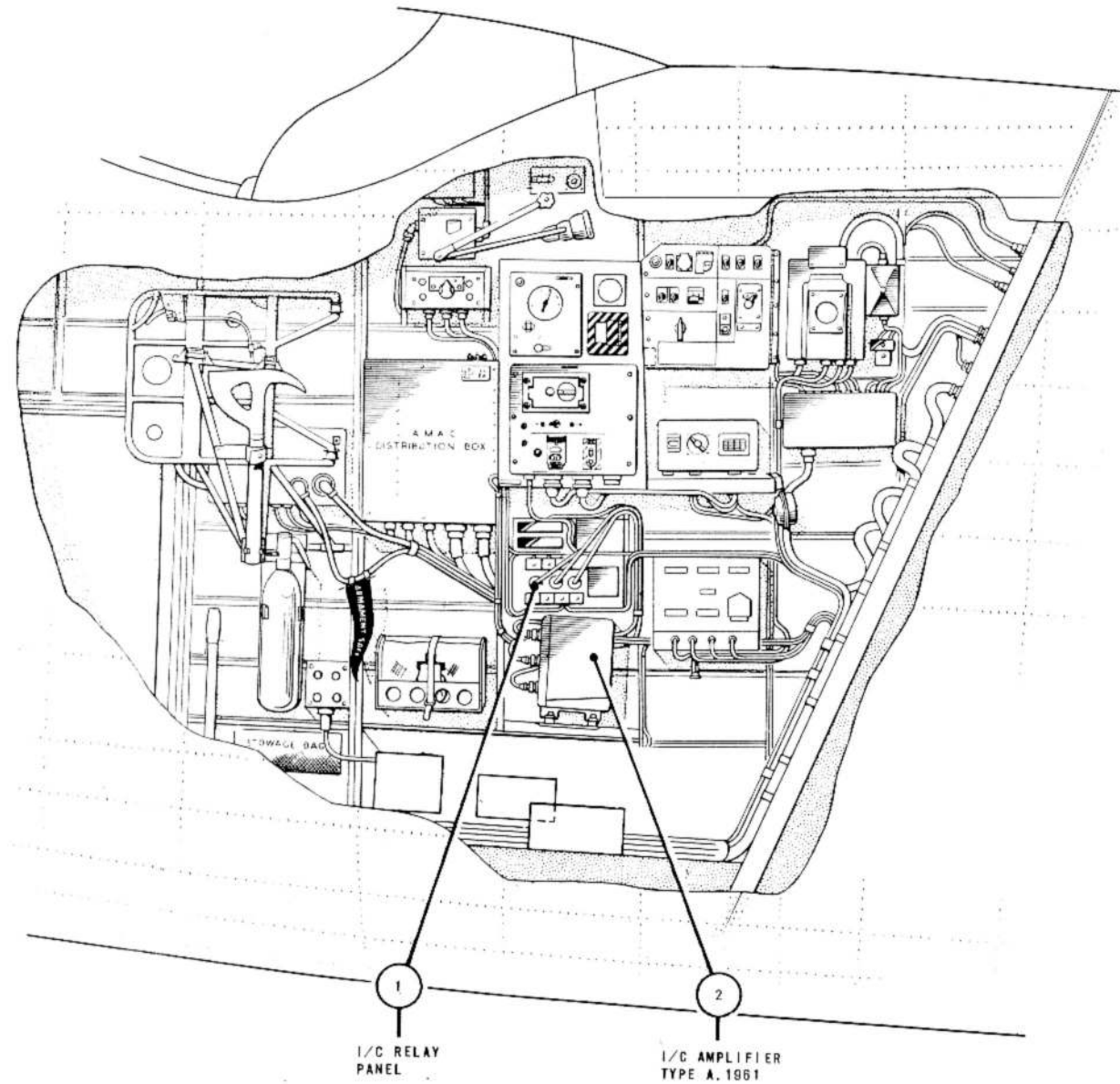
FIG.15. WIRELESS INSTALLATION - AIR BOMBER'S REAR STATION (B(1)MK.6 AIRCRAFT)
