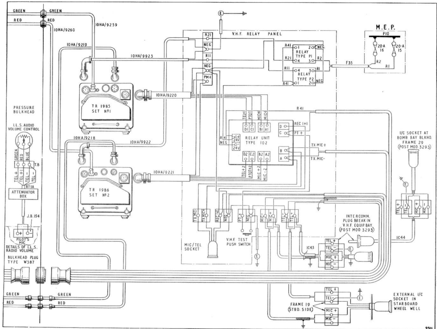
FIG. 1A. INTERCOMMUNICATION AND V.H.F. COMMUNICATION ( B MK.6 AIRCRAFT )
