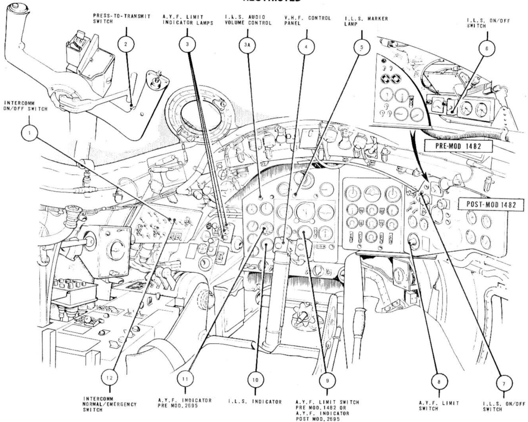
FIG.10. WIRELESS INSTALLATION - PILOT'S STATION (B MK.6 AIRCRAFT)
