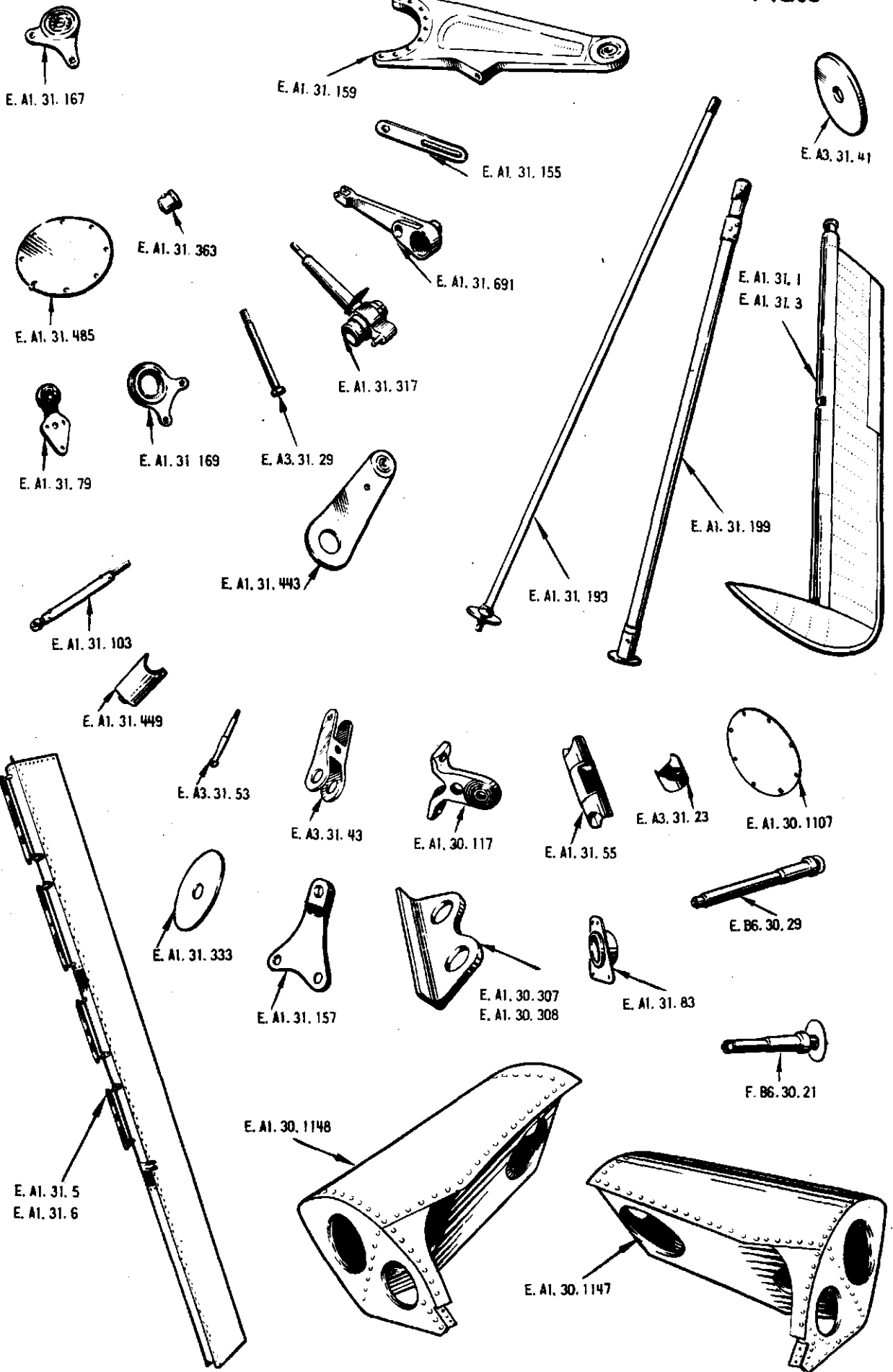
TAILPLANE AND ELEVATORS
